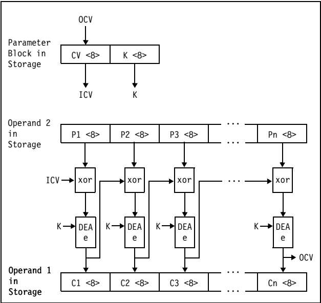
Figure 7-24. KMC-DEA Encipher Operation
