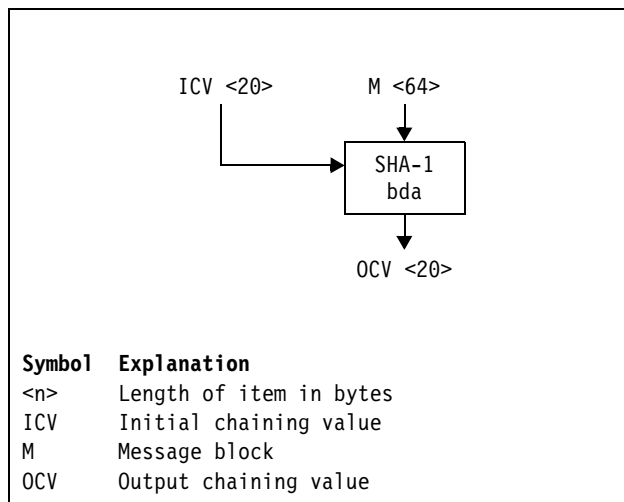
Figure 7-52. Symbol for SHA-1 Block Digest Algorithm
