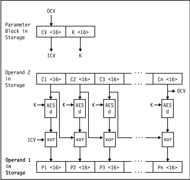
Figure 7-34. KMC-AES-128 Decipher Operation
