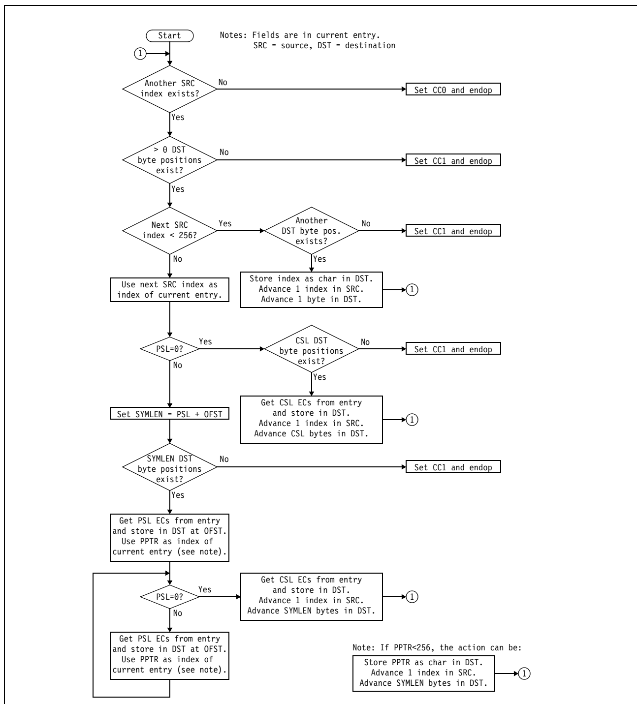
Figure 7-48. Expansion Process
