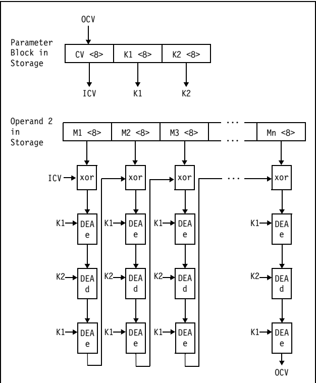
Figure 7-79. KMAC-TDEA-128
