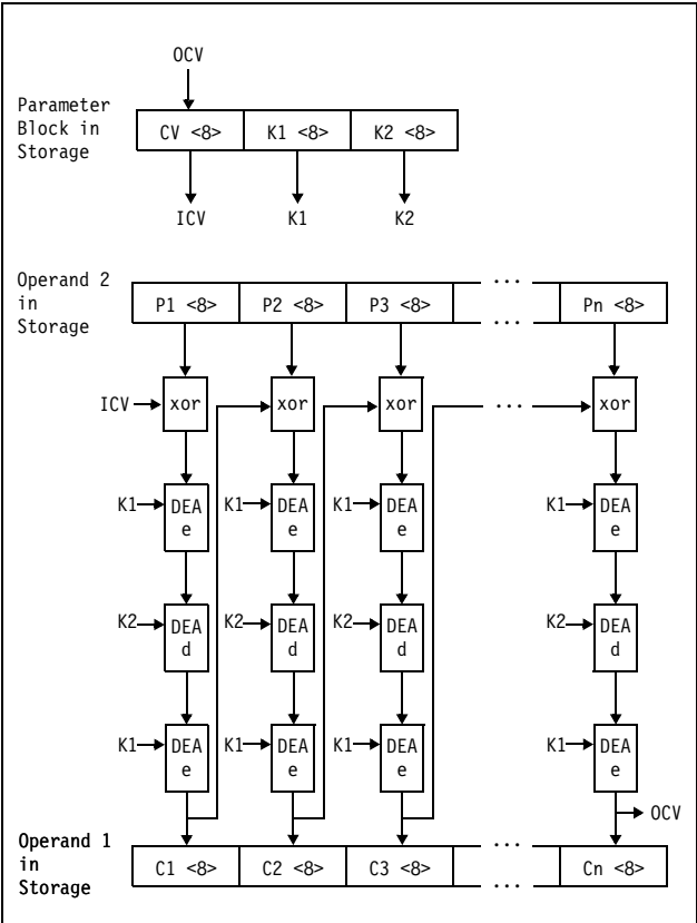
Figure 7-27. KMC-TDEA-128 Encipher Operation
