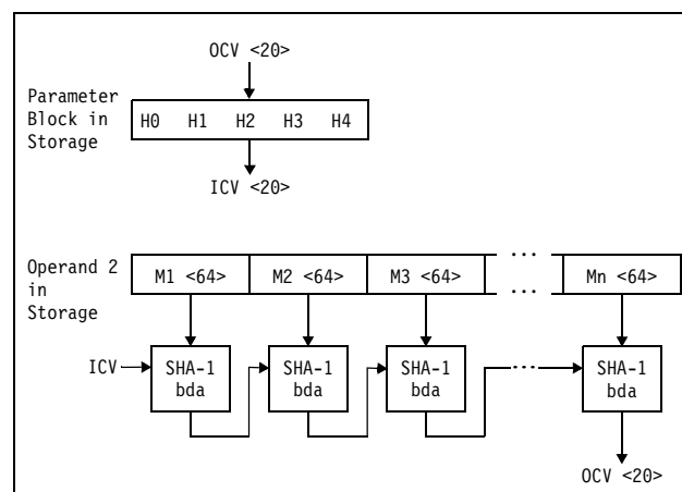
Figure 7-56. KIMD-SHA-1
