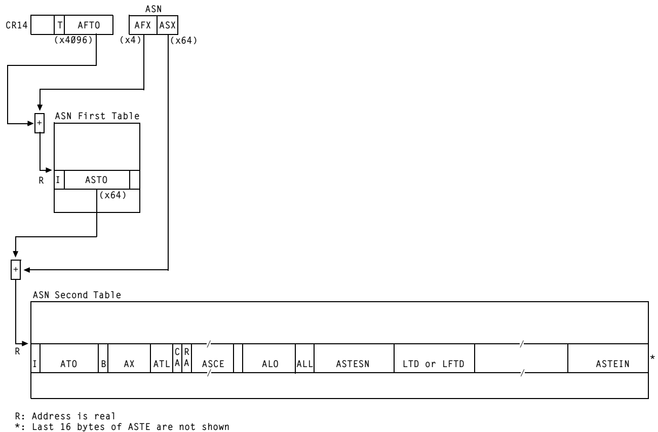
Figure 3-7. ASN Translation
