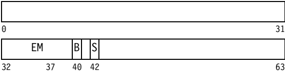
Control Register 10
