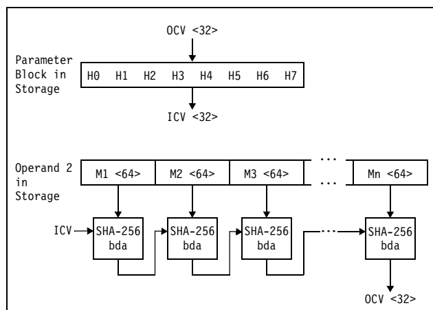
Figure 7-58. KIMD-SHA-256
