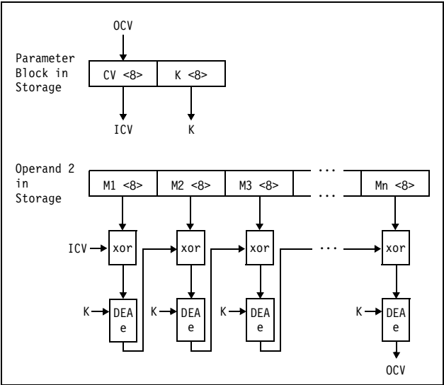
Figure 7-77. KMAC-DEA
