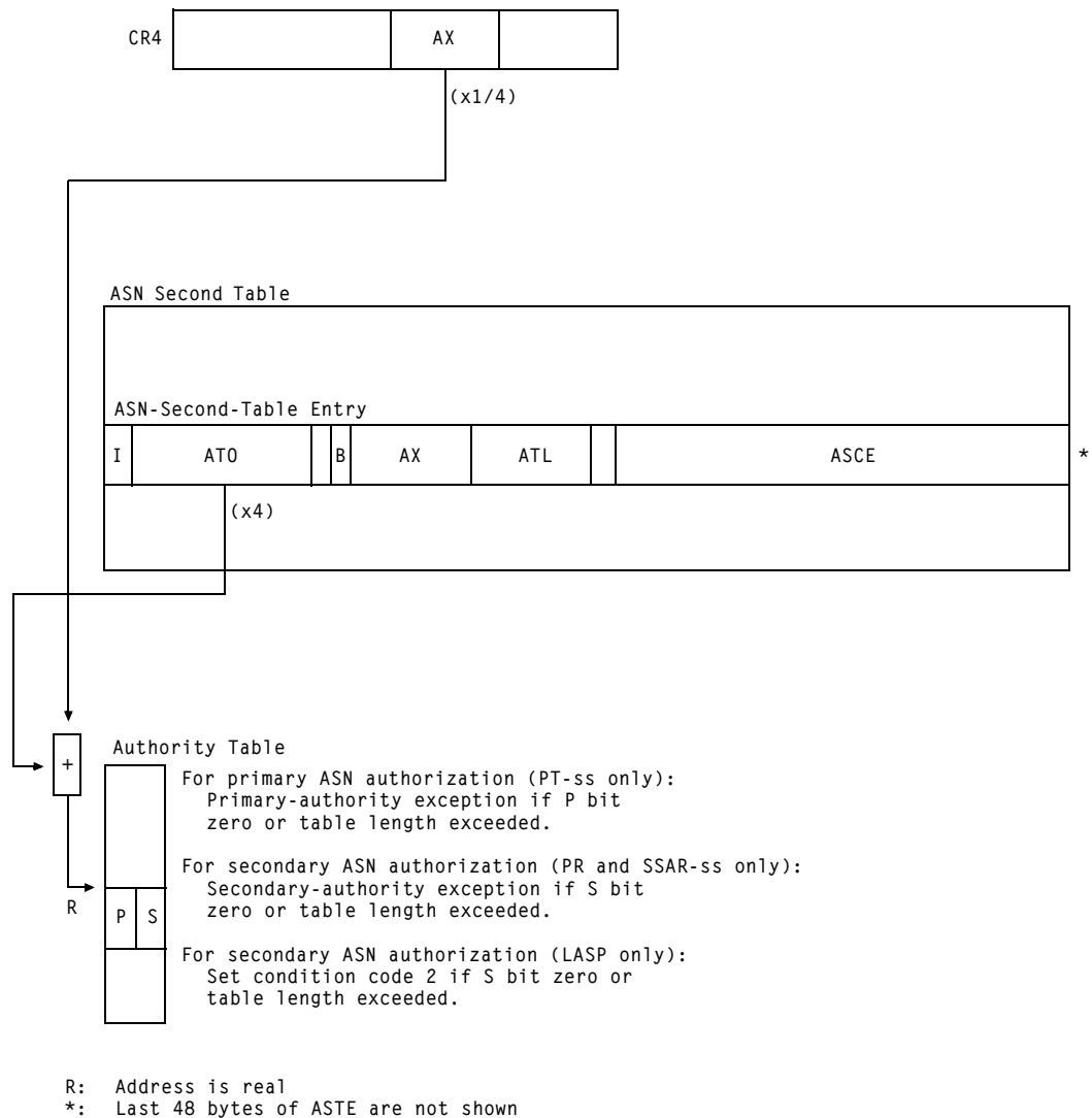
Figure 3-8. ASN Authorization
