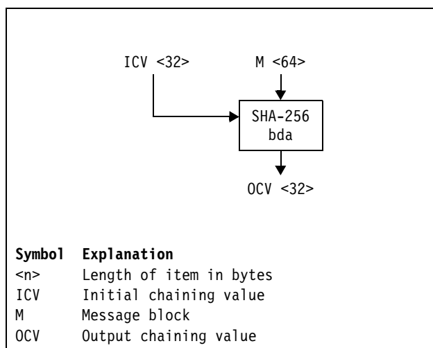
Figure 7-53. Symbol for SHA-256 Block Digest Algorithm
