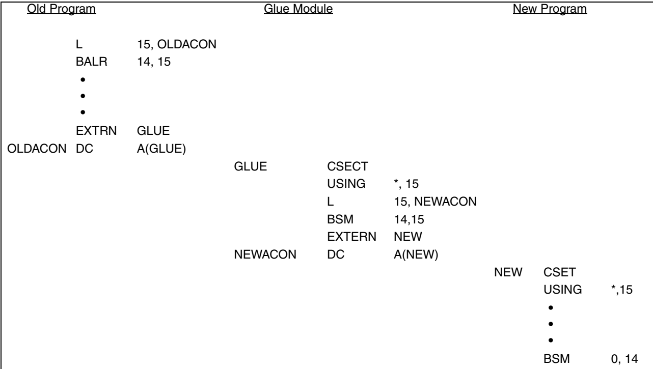
Figure 5-5. Glue Module for Linkage from the 24-Bit Mode to the 31-Bit Mode
