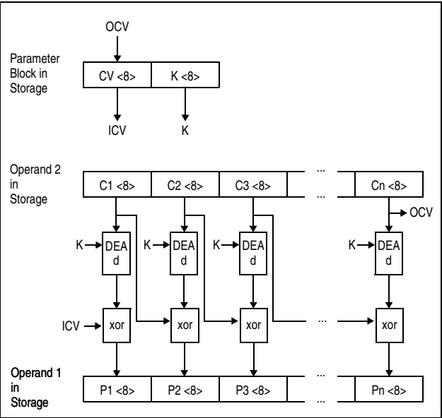
Figure 7-25. KMC-DEA Decipher Operation
