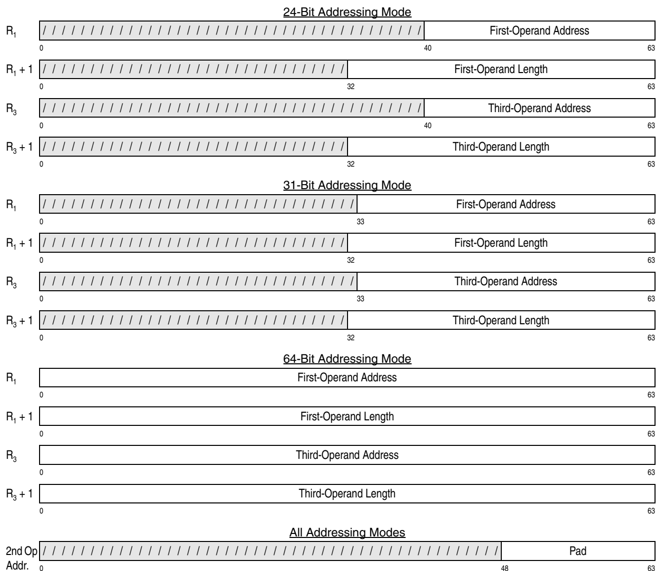
Figure 7-44. Register Contents and Second-Operand Address for COMPARE LOGICAL LONG UNICODE
