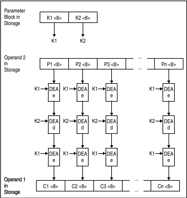
Figure 7-14. KM-TDEA-128 Encipher Operation
