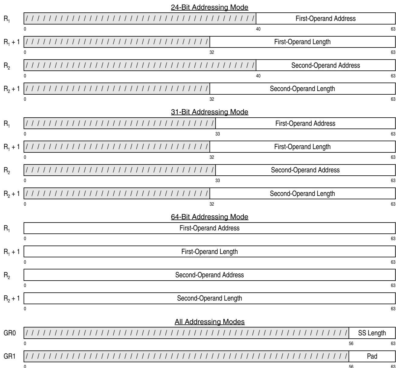
Figure 7-45. Register Contents and Second-Operand Address for COMPARE UNTIL SUBSTRING EQUAL
