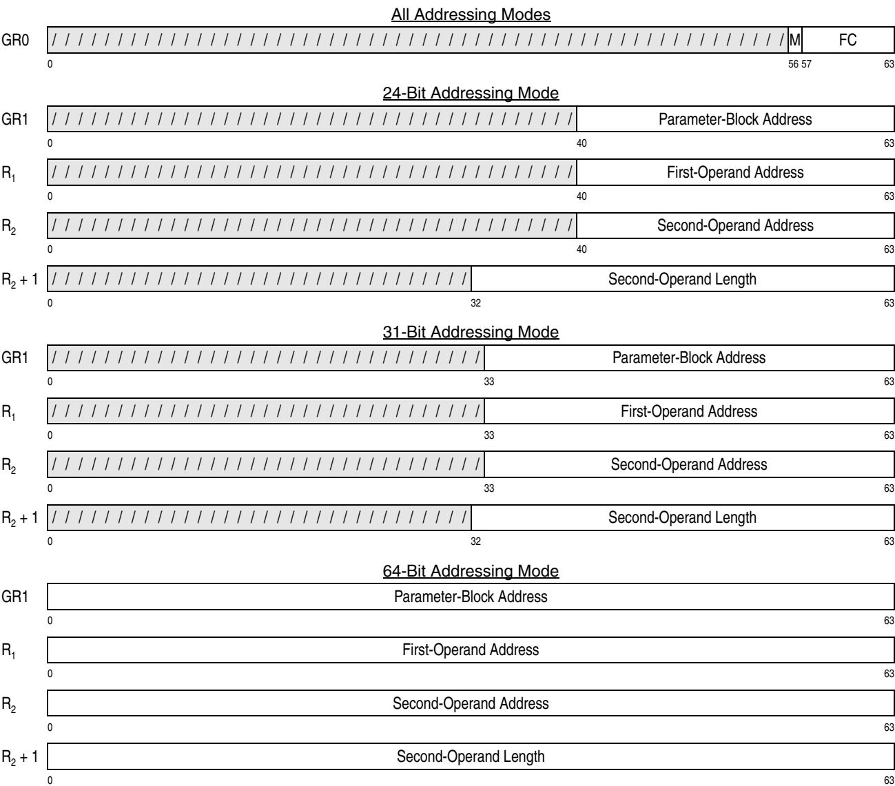
Figure 7-5. General Register Assignment for KM and KMC
