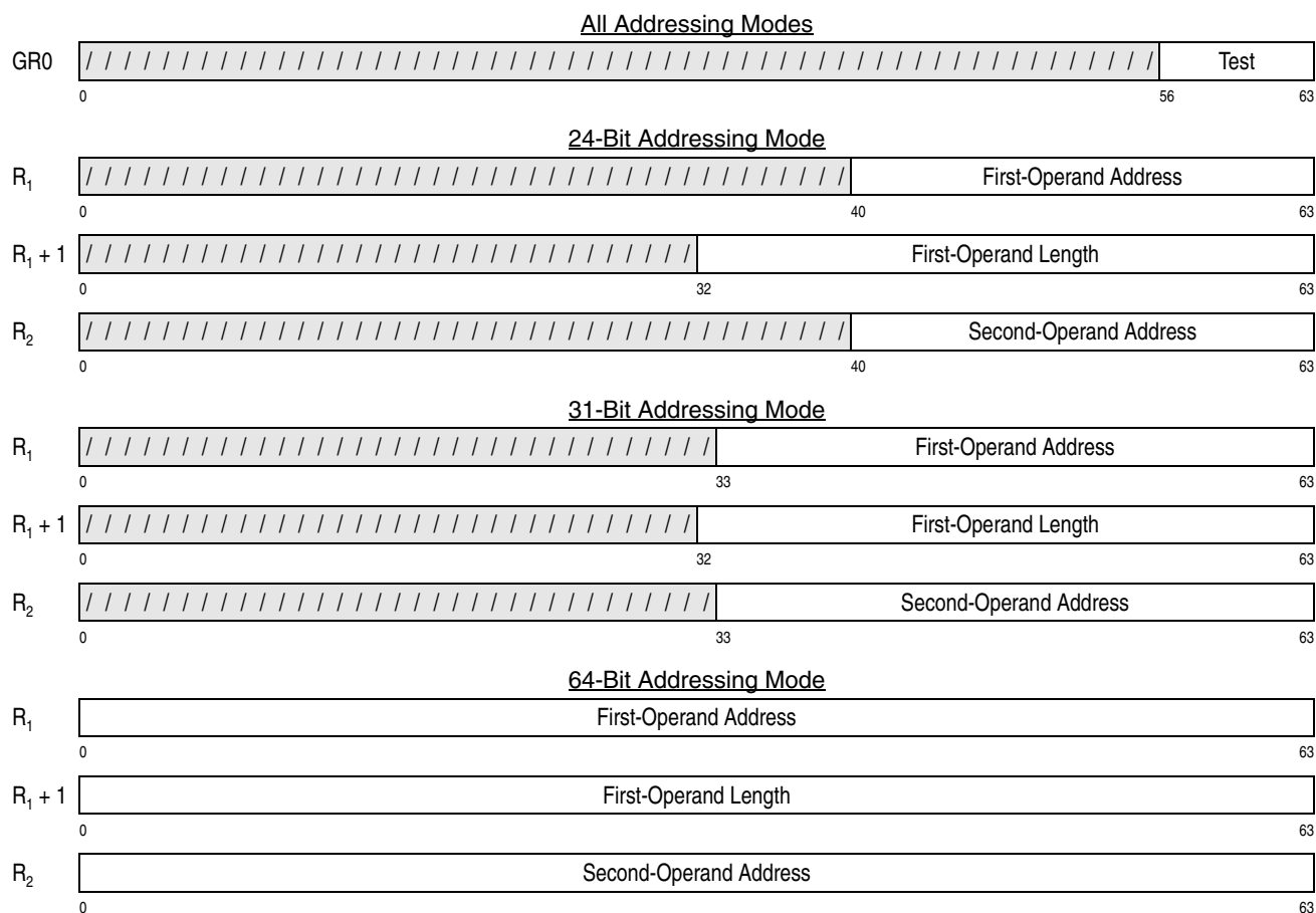
Figure 7-98. Register Contents for TRANSLATE EXTENDED
