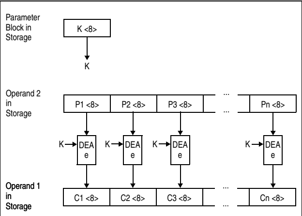
Figure 7-11. KM-DEA Encipher Operation
