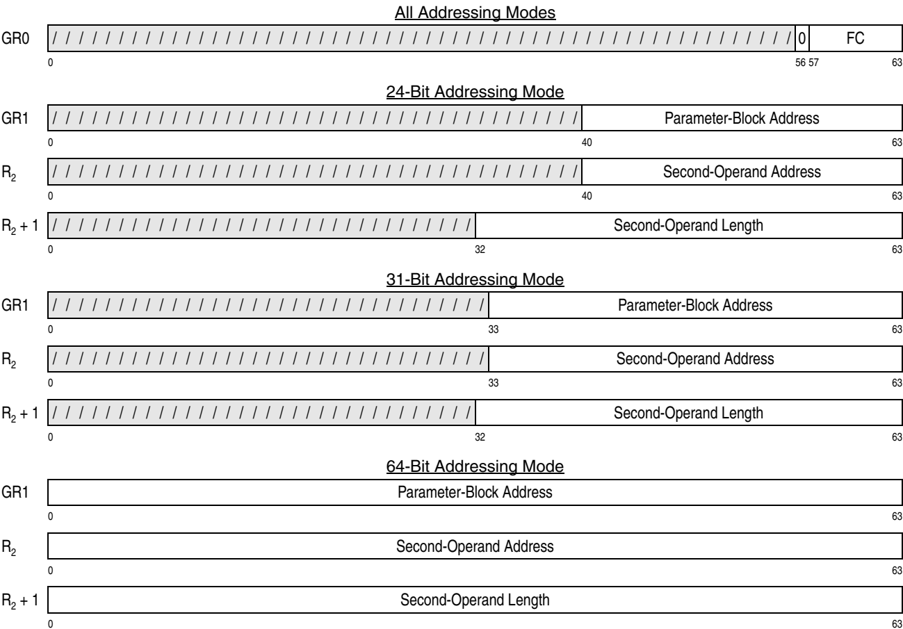
Figure 7-72. General Register Assignment for KMAC
