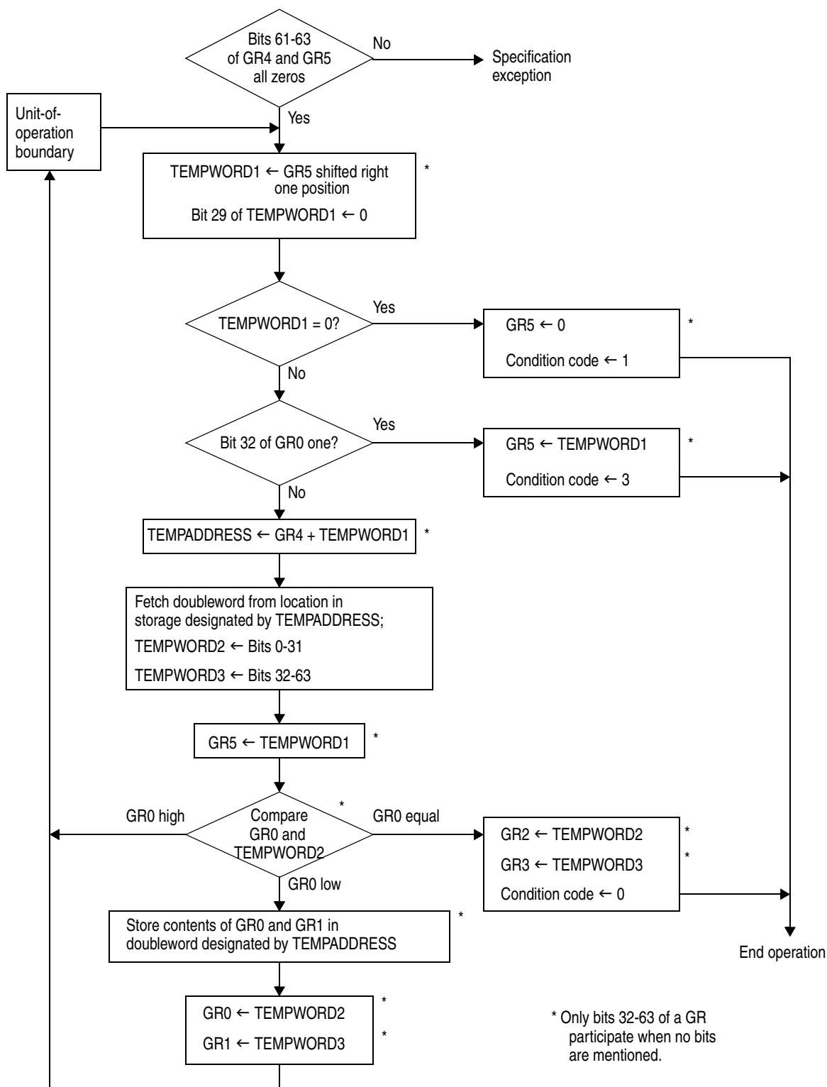
Figure 7-100. Execution of UPDATE TREE in the 24-Bit or 31-Bit Addressing Mode
