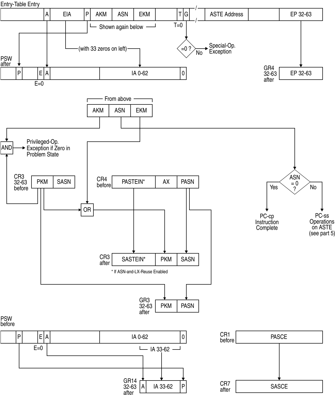
Figure 10-43. Execution of PROGRAM CALL (Part 1 of 5).
