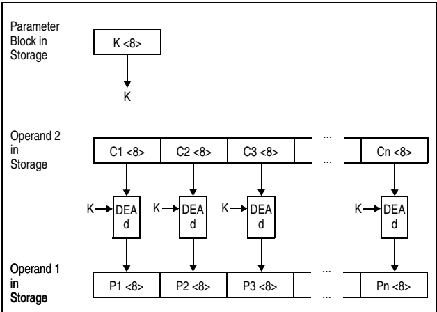
Figure 7-12. KM-DEA Decipher Operation
