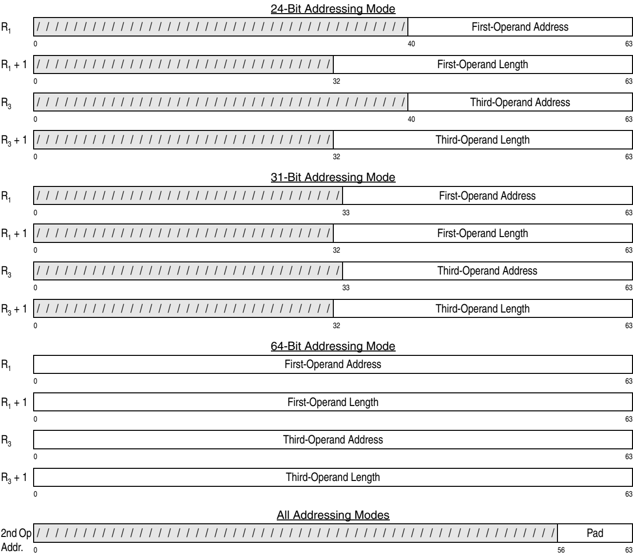
Figure 7-91. Register Contents and Second-Operand Address for MOVE LONG EXTENDED
