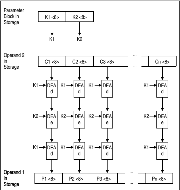
Figure 7-15. KM-TDEA-128 Decipher Operation
