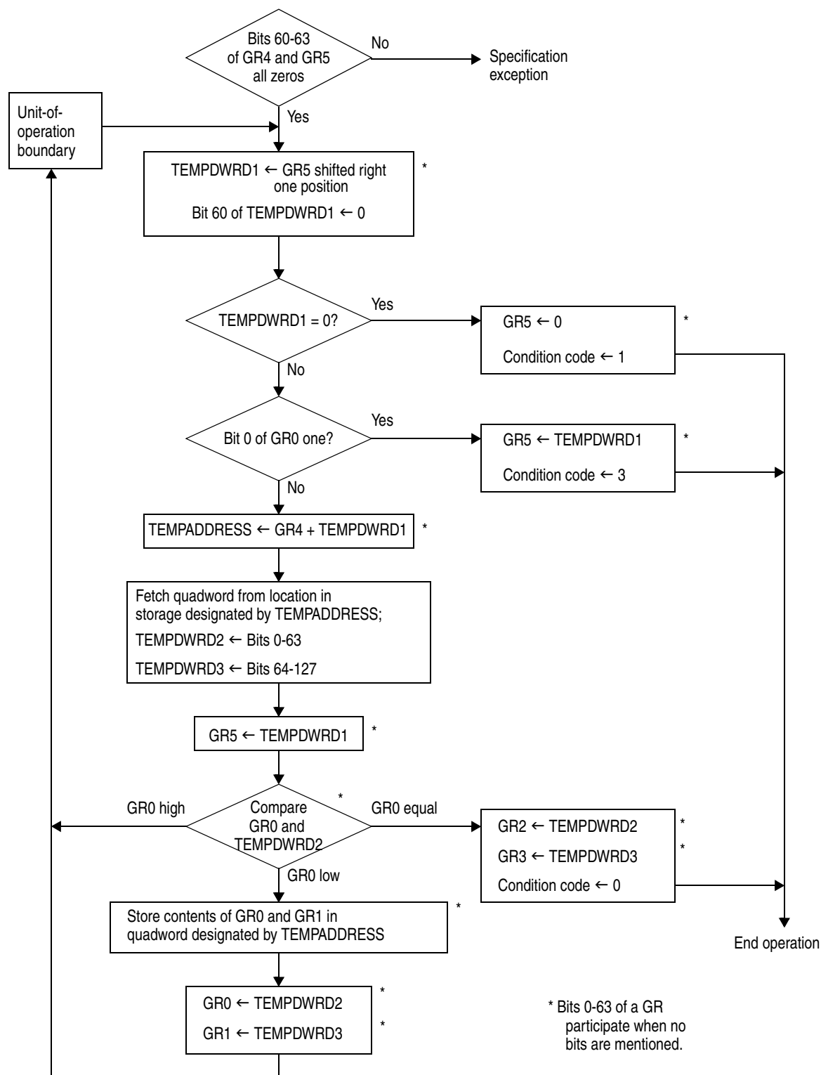
Figure 7-101. Execution of UPDATE TREE in the 64-Bit Addressing Mode
