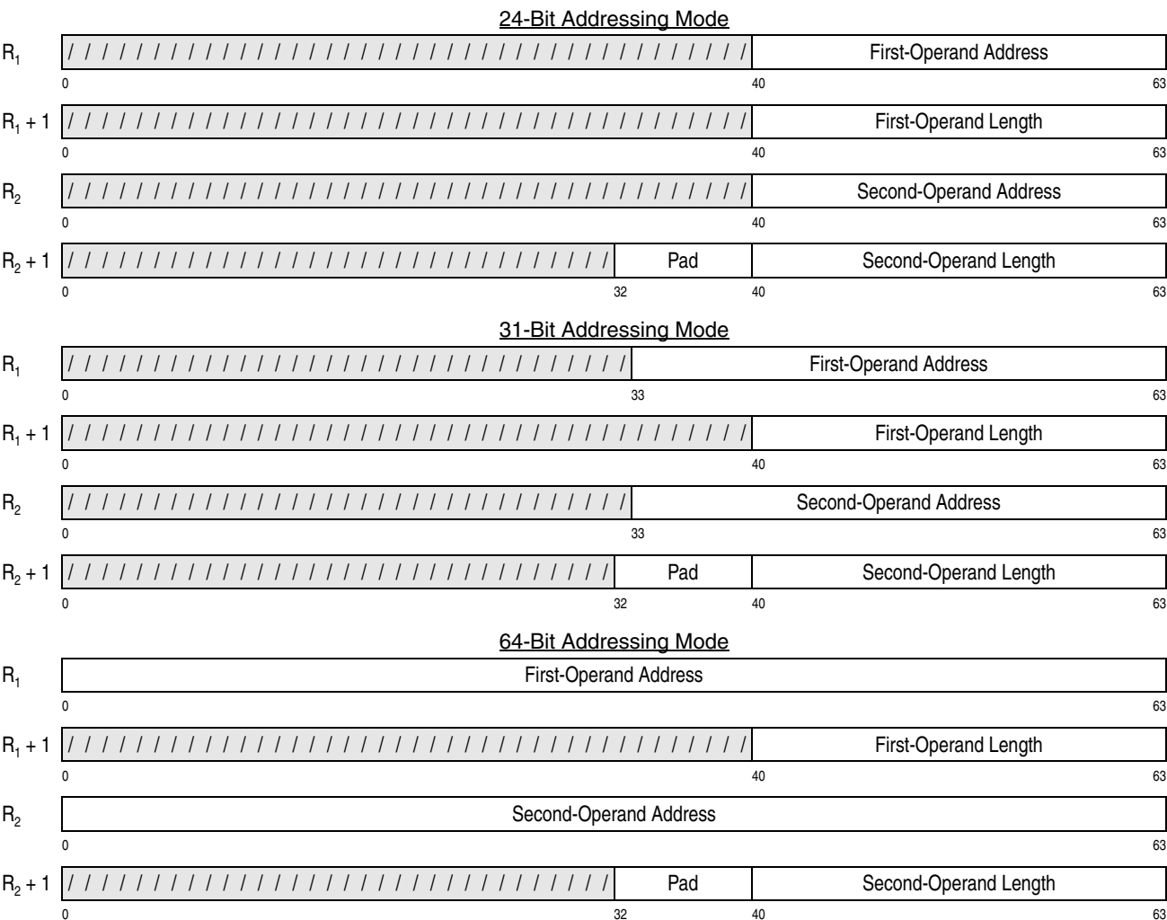
Figure 7-42. Register Contents for COMPARE LOGICAL LONG
