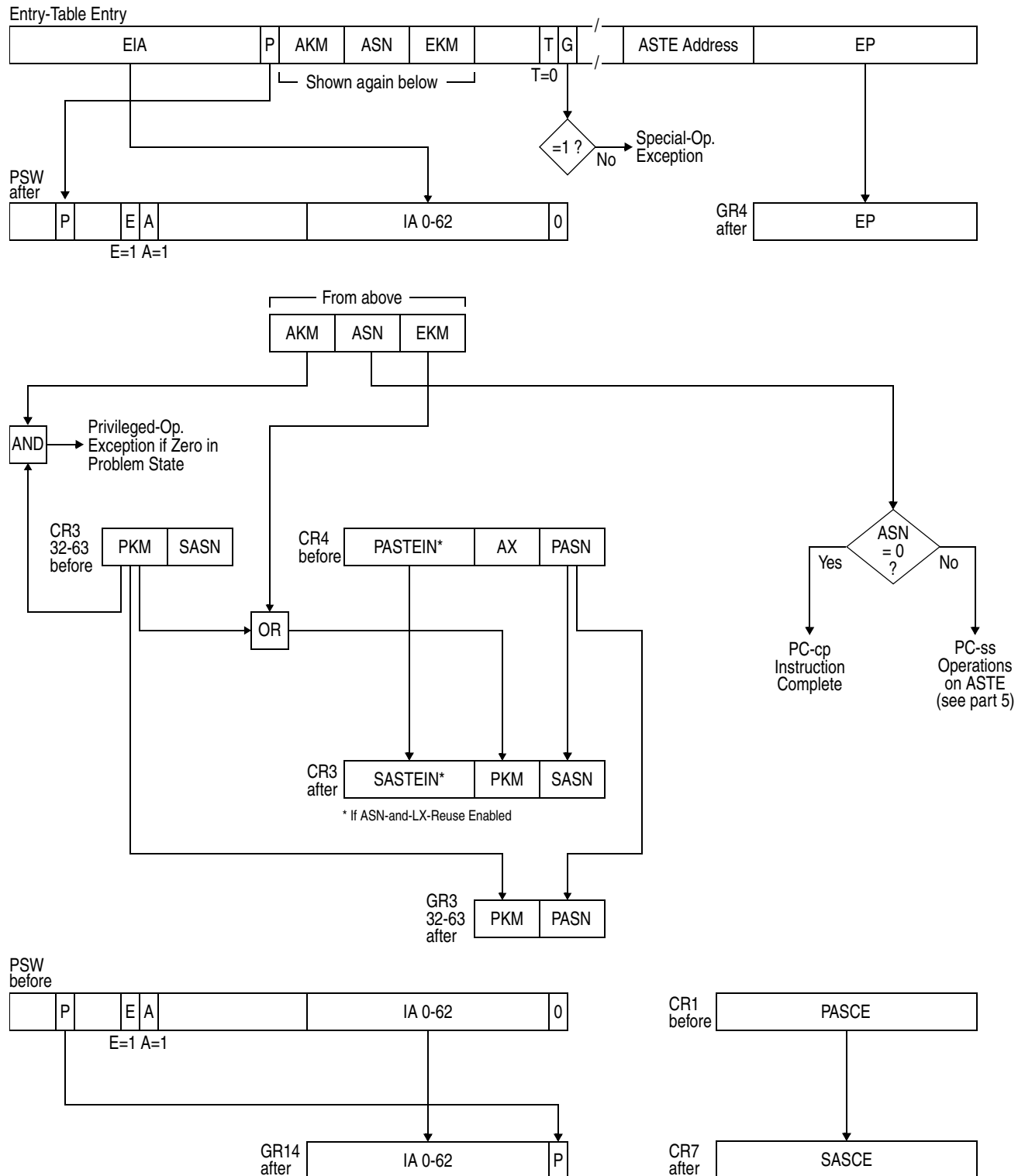
Figure 10-43. Execution of PROGRAM CALL (Part 2 of 5).
