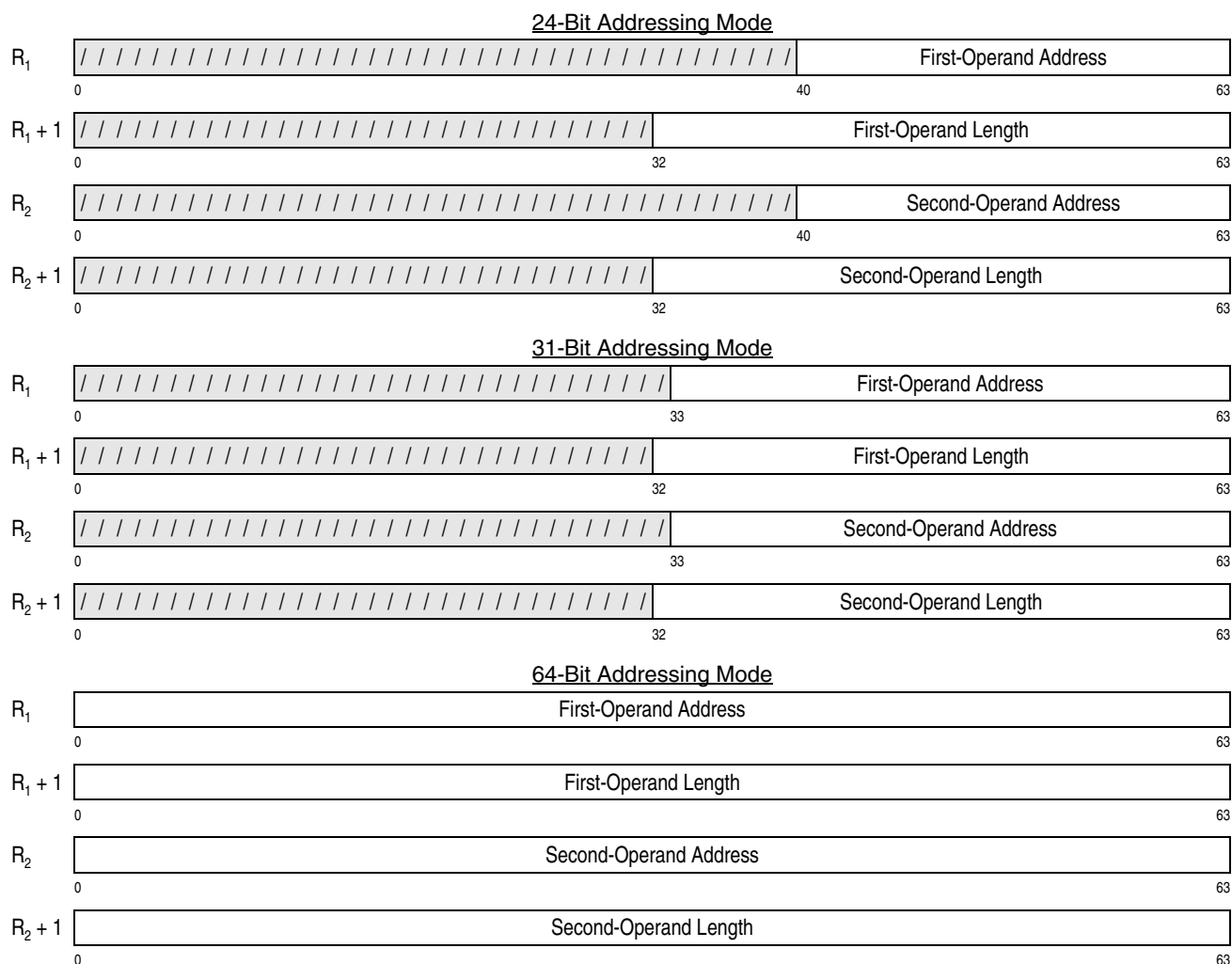
Figure 7-88. Register Contents for CONVERT UTF-8 TO UTF32
