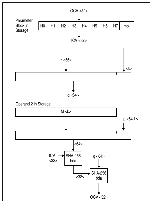
Figure 7-69. KLMD-SHA-256 Partial-Block Case 2 ( 56 \leq L \leq 63 )
