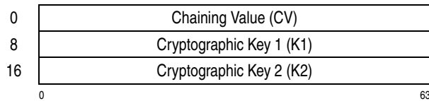
Figure 7-78. Parameter Block for KMAC-TDEA-128
