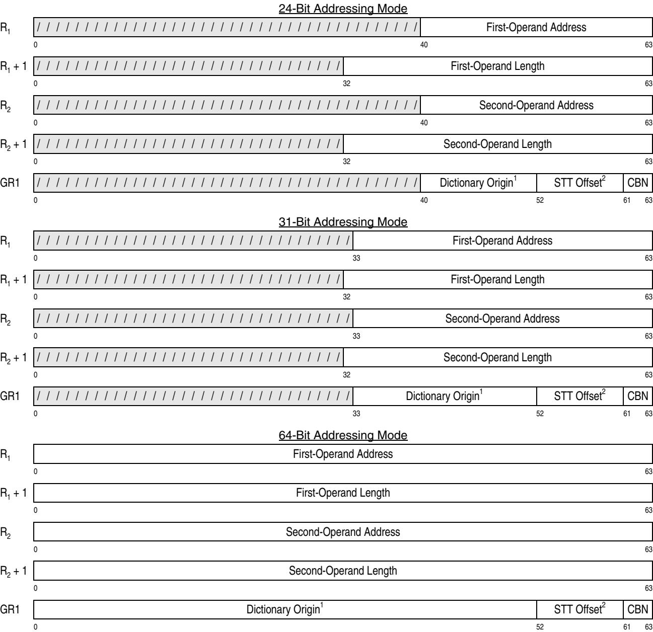
Figure 7-46. Register Contents for COMPRESSION CALL (Part 1 of 2)
