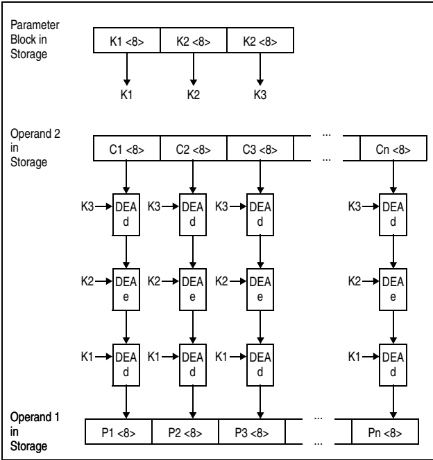
Figure 7-18. KM-TDEA-192 Decipher Operation
