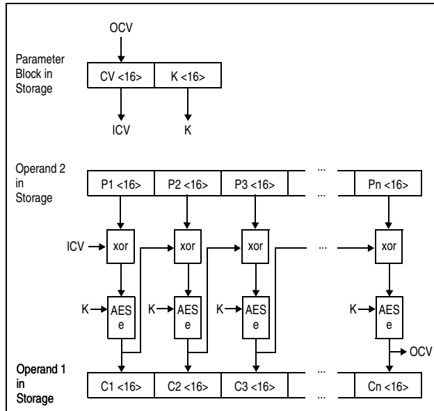
Figure 7-33. KMC-AES-128 Encipher Operation
