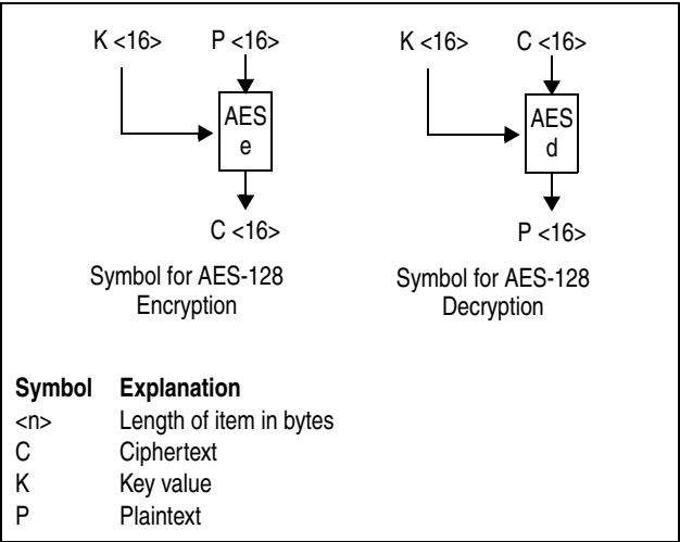
Figure 7-8. Symbols for AES-128 Encryption and Decryption
