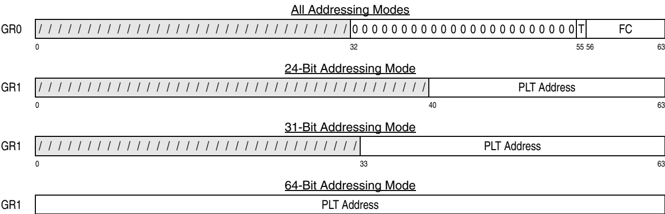
Figure 7-94. General Register Assignment for PLO
