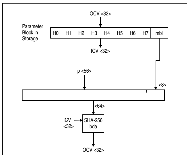
Figure 7-67. KLMD-SHA-256 Empty Block ( L = 0 )
