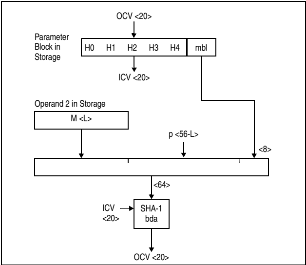
Figure 7-63. KLMD-SHA-1 Partial-Block Case 1 (1 ≤ L ≤ 55)
