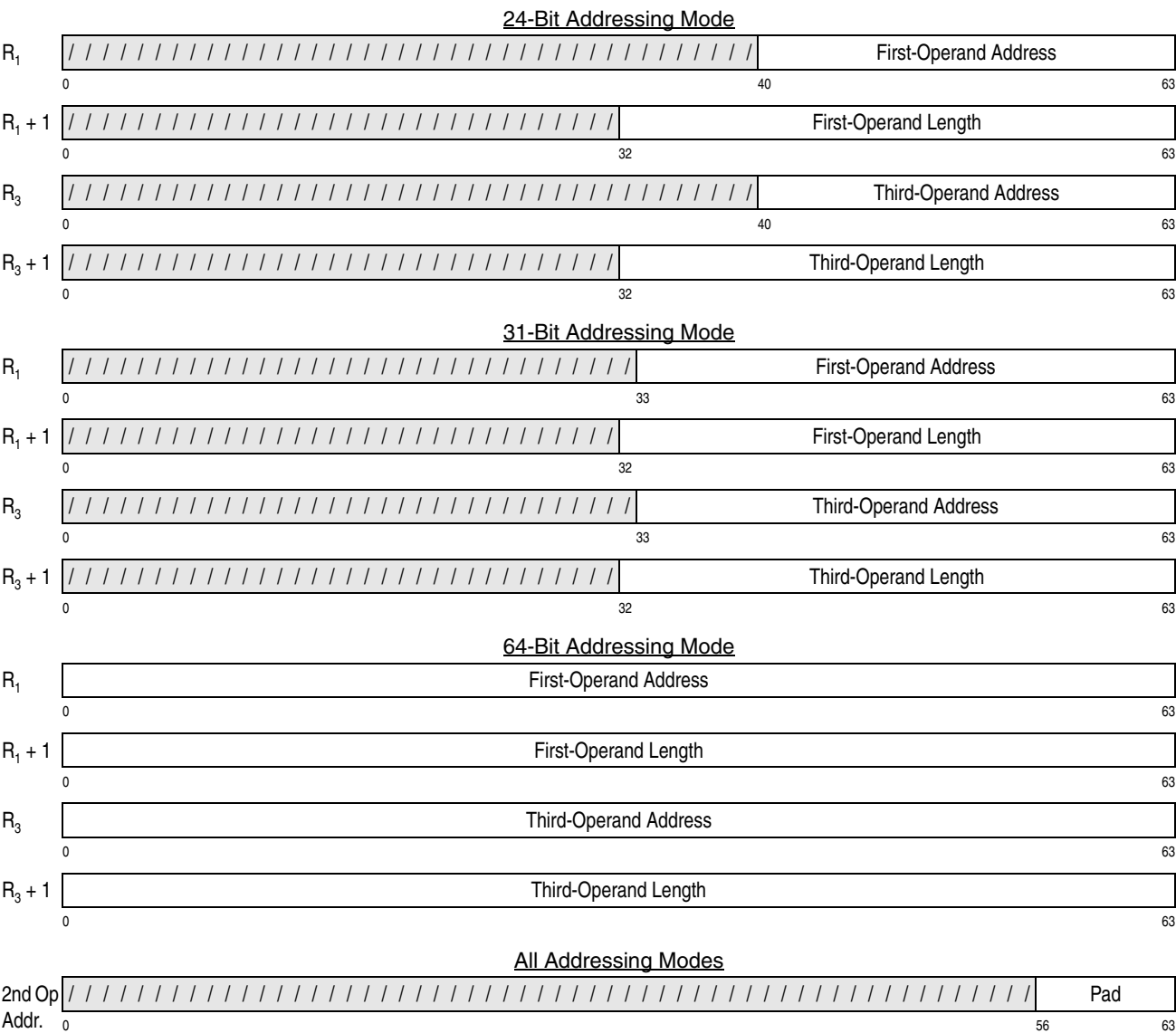
Figure 7-43. Register Contents and Second-Operand Address for COMPARE LOGICAL LONG EXTENDED
