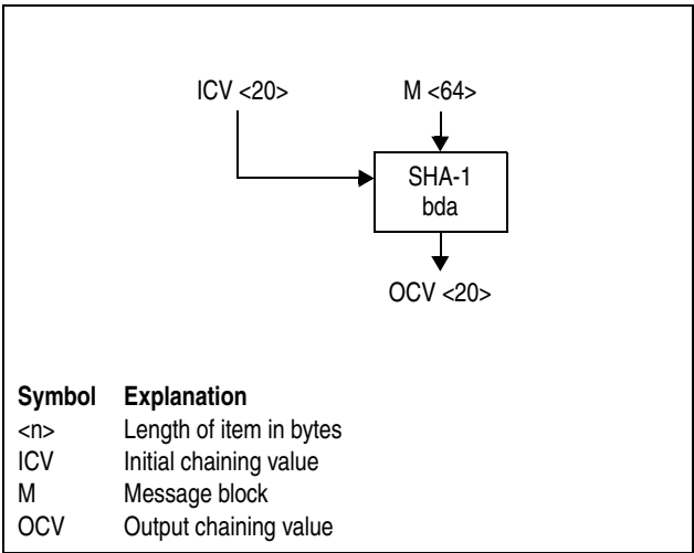
Figure 7-52. Symbol for SHA-1 Block Digest Algorithm
