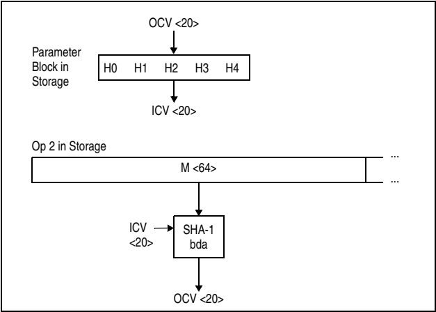
Figure 7-61. KLMD-SHA-1 Full Block (L ≥ 64)
