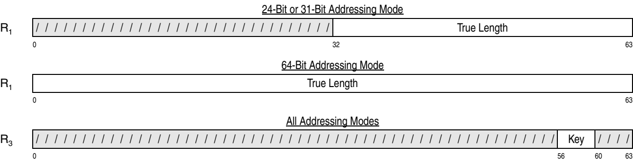
Figure 10-26. Register Contents of MOVE WITH KEY
