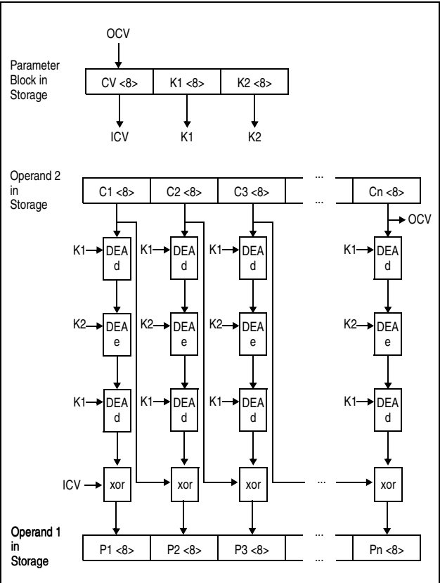
Figure 7-28. KMC-TDEA-128 Decipher Operation
