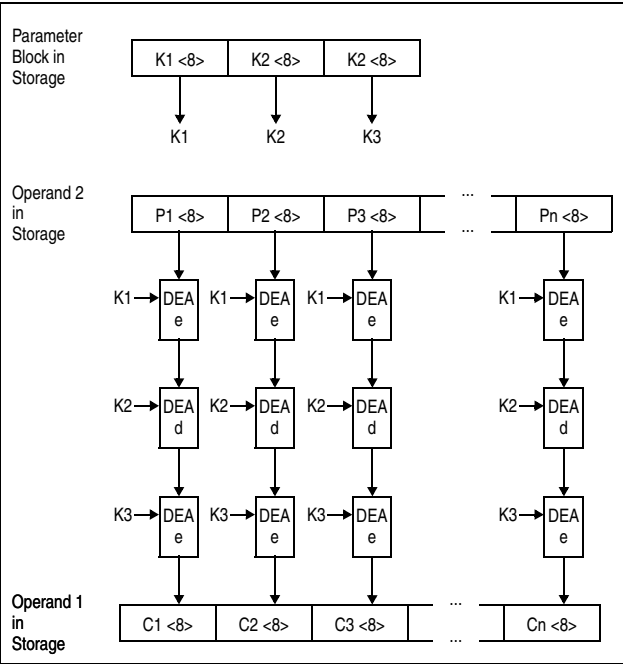
Figure 7-17. KM-TDEA-192 Encipher Operation
