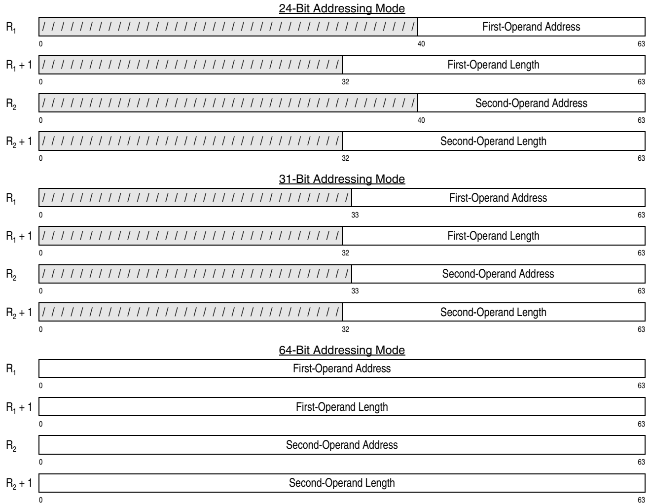
Figure 7-87. Register Contents for CONVERT UTF-8 TO UTF-16
