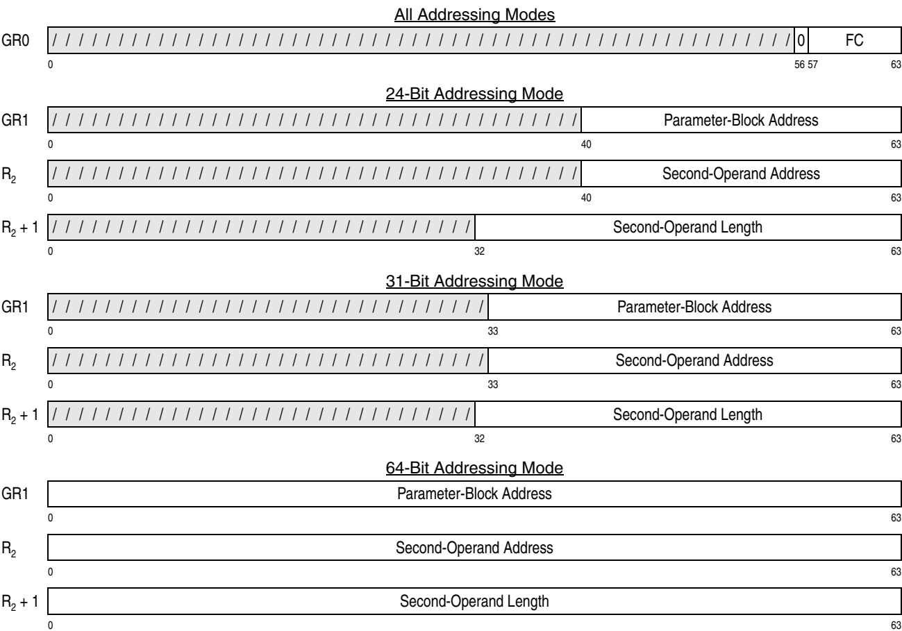
Figure 7-51. General Register Assignment for KIMD and KLMD
