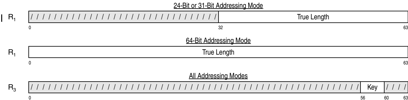
Figure 10-23. Register Contents of MOVE TO PRIMARY and MOVE TO SECONDARY
