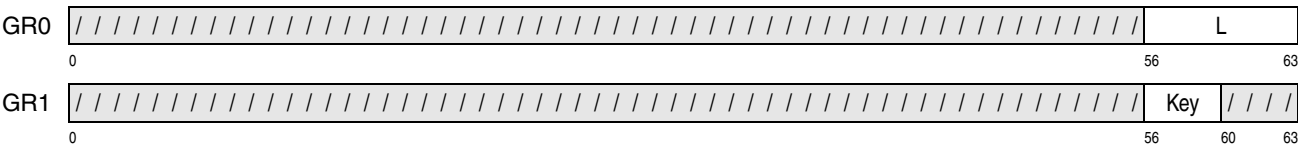
Figure 10-28. Register Contents of MOVE WITH SOURCE KEY
