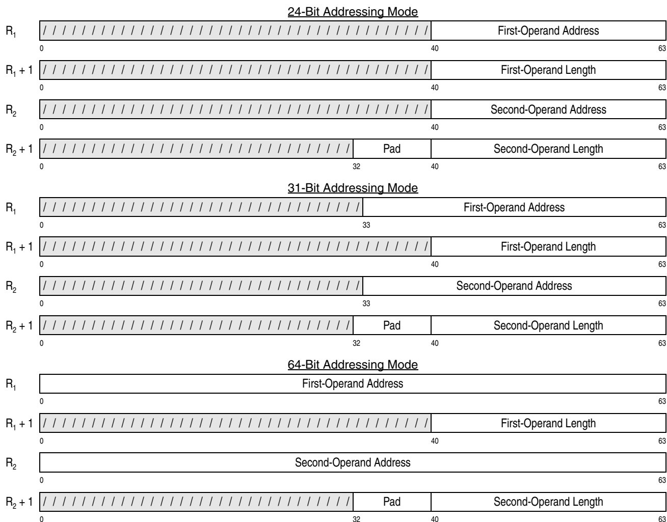
Figure 7-90. Register Contents for MOVE LONG
