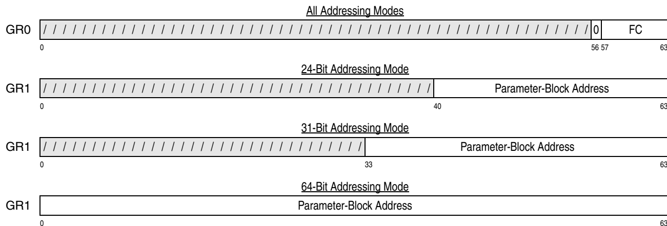
Figure 10-29. General Register Assignment for PERFORM TIMING FACILITY FUNCTION
