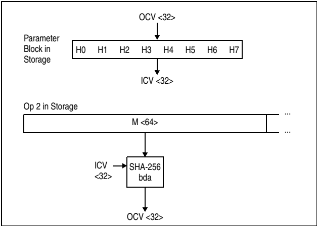
Figure 7-66. KLMD-SHA-256 Full Block (L ≥ 64)
