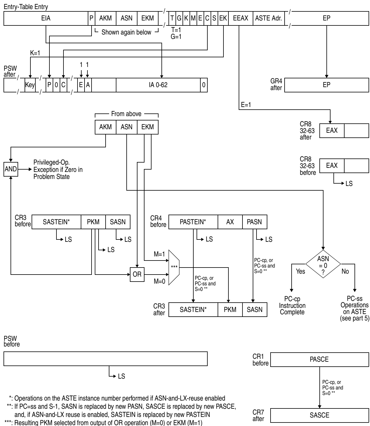
Figure 10-43. Execution of PROGRAM CALL (Part 3 of 5).
