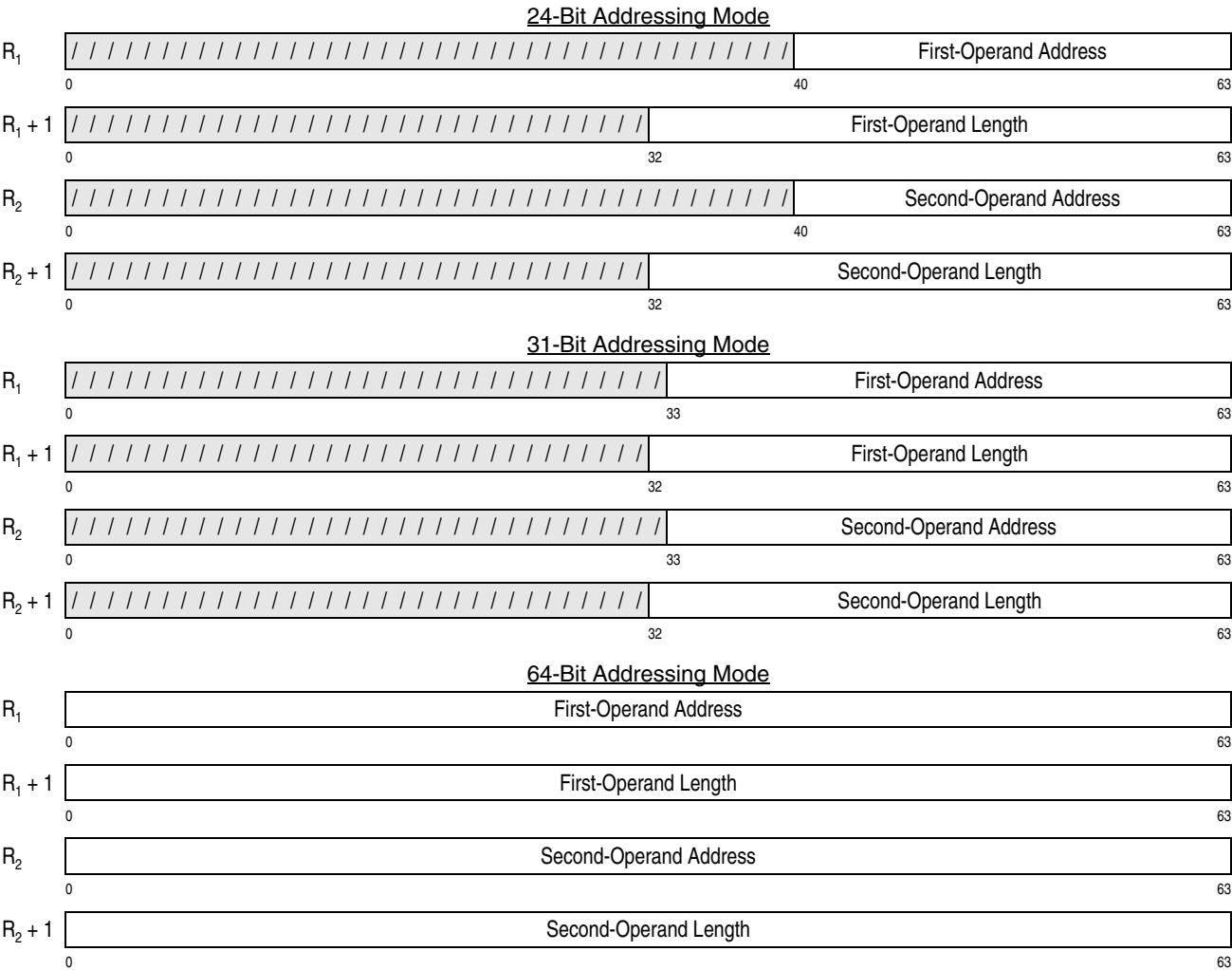
Figure 7-85. Register Contents for CONVERT UTF-32 TO UTF-16
