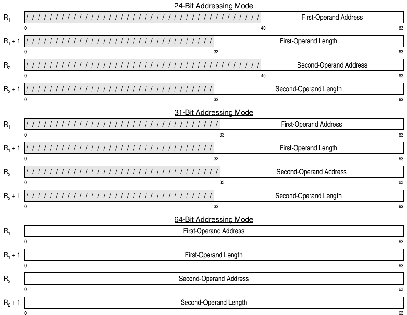
Figure 7-83. Register Contents for CONVERT UTF-16 TO UTF-32
