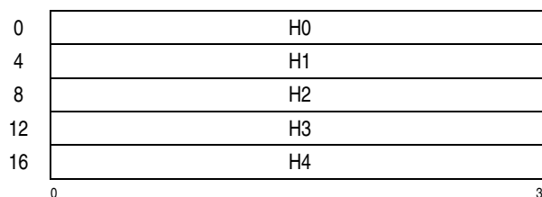
Figure 7-55. Parameter Block for KIMD-SHA-1
