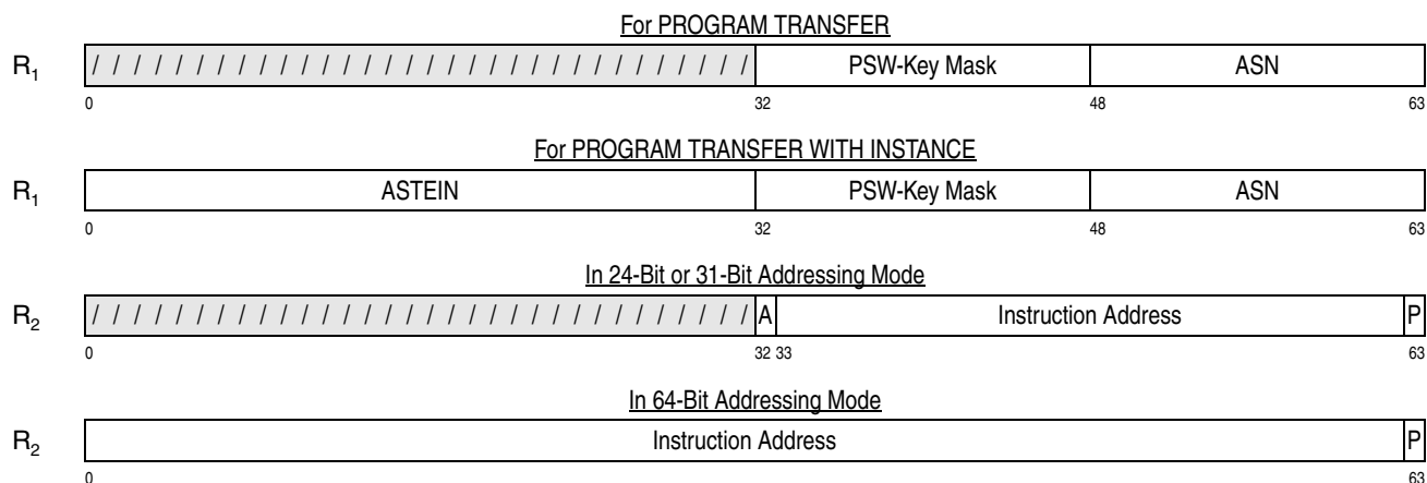
Figure 10-45. Register Contents for PROGRAM TRANSFER (WITH INSTANCE)
