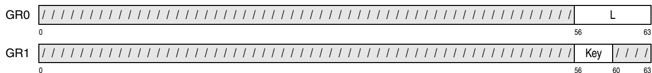
Figure 10-25. Register Contents of MOVE WITH DESTINATION KEY
