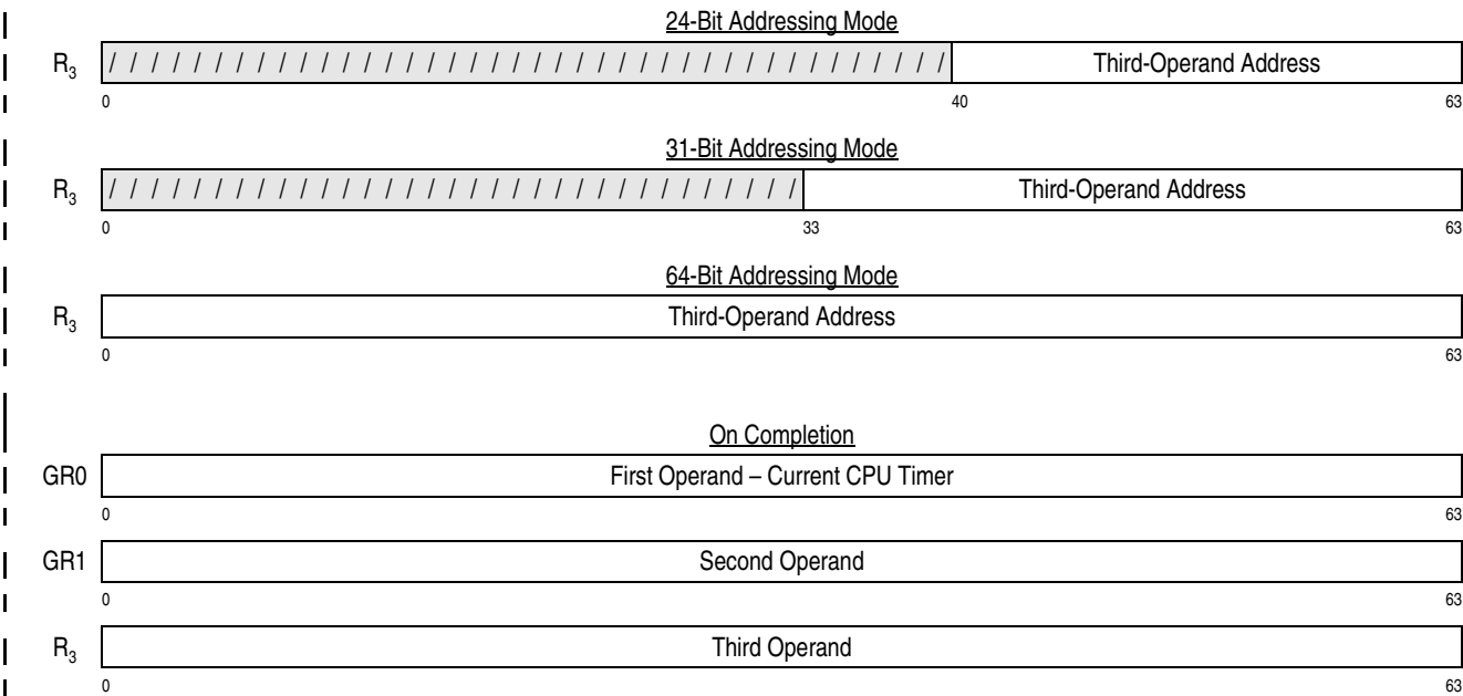
Figure 7-89. General Register Assignment for EXTRACT CPU TIME
