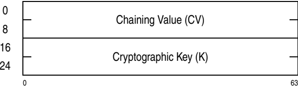
Figure 7-32. Parameter Block for KMC-AES-128
