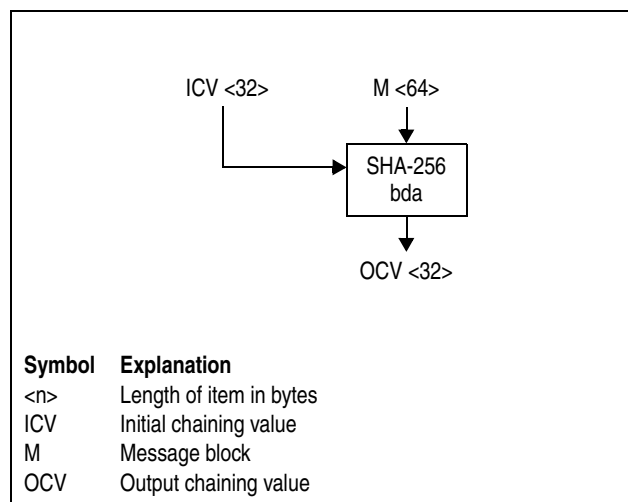
Figure 7-53. Symbol for SHA-256 Block Digest Algorithm
