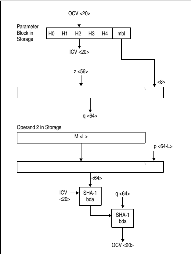
Figure 7-64. KLMD-SHA-1 Partial-Block Case 2 (56 ≤ L ≤ 63)
