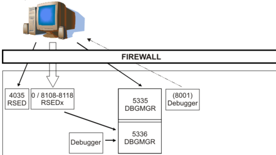
Figure 3. TCP/IP ports
