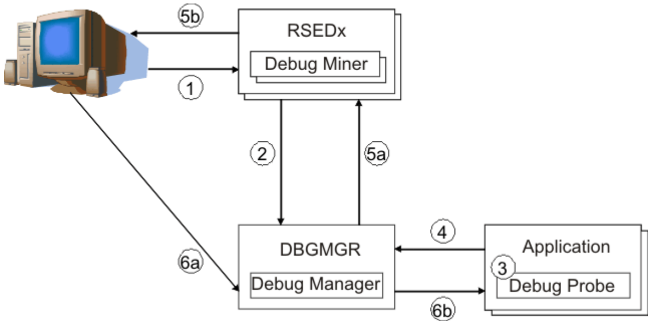
Figure 2. Debug Manager
