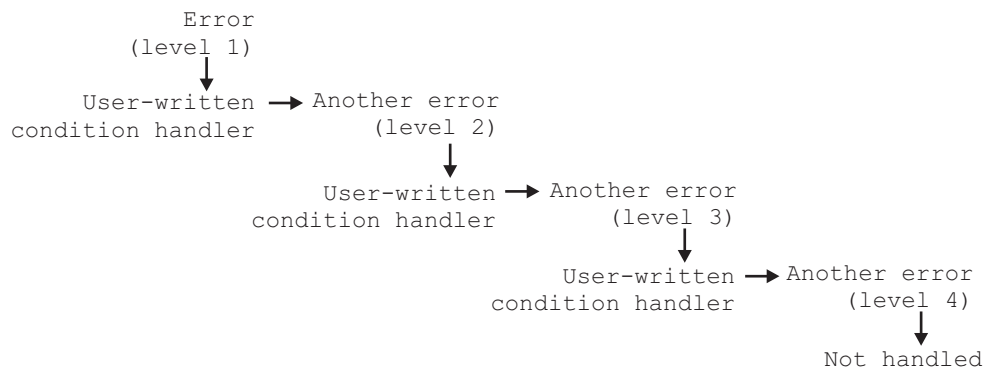
Figure 2. Effect of DEPTHCONDLMT(3) on Condition Handling
