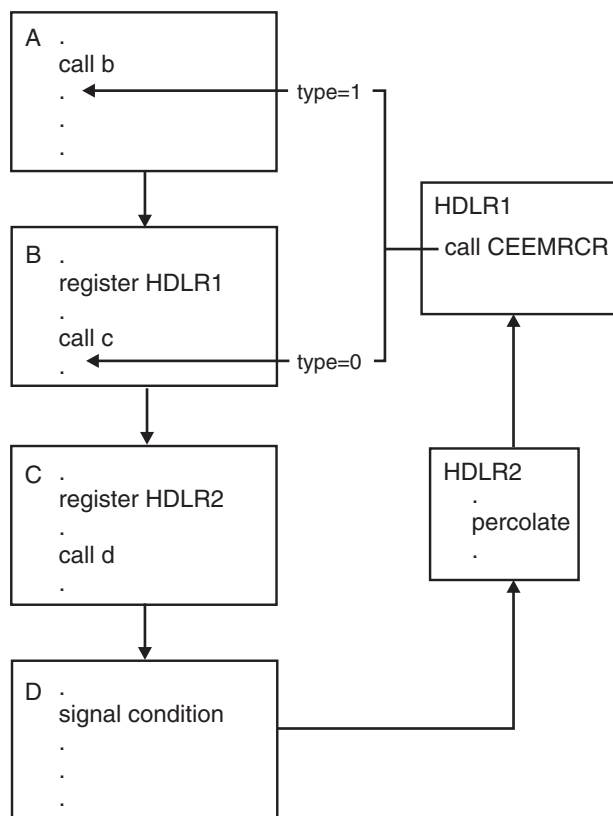
Figure 145. First Example Moving Resume Cursor Using CEEMRCR
