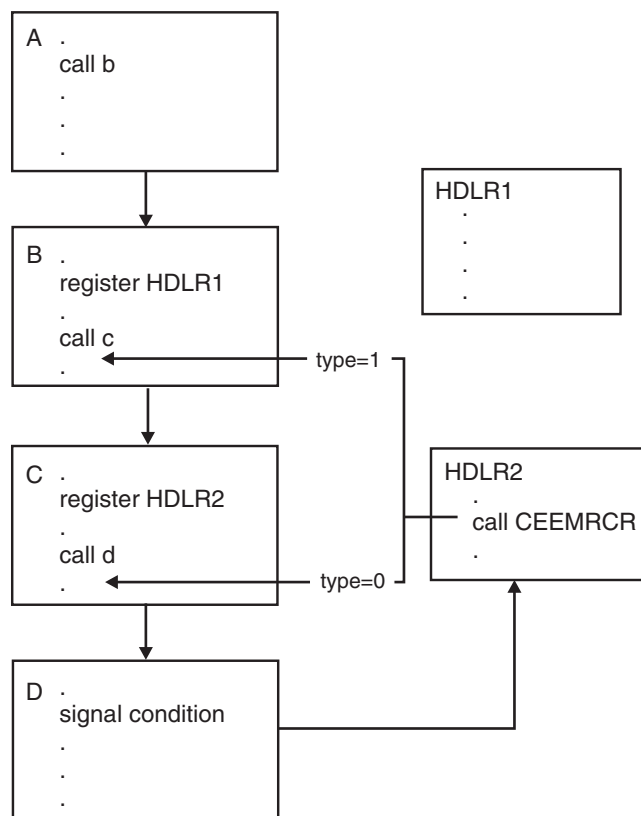
Figure 146. Second Example Moving Resume Cursor Using CEEMRCR
