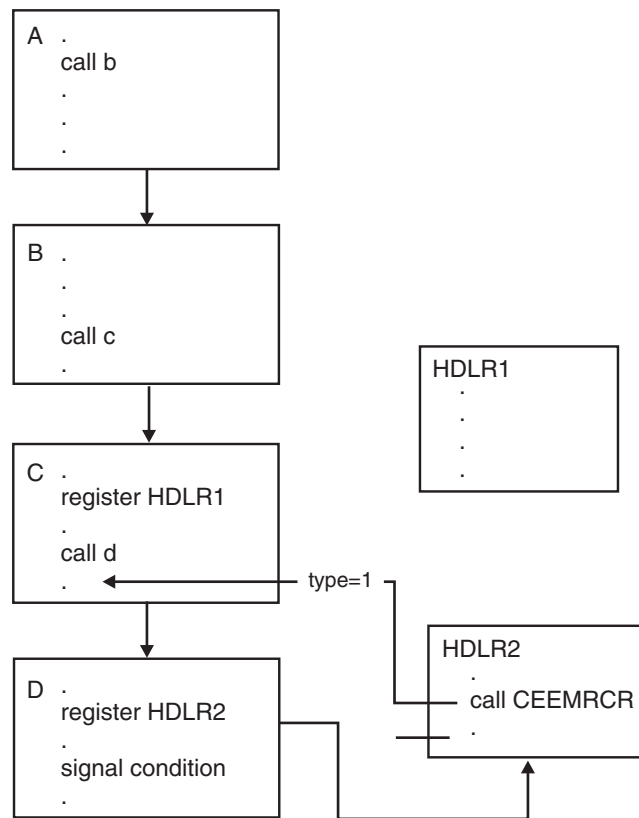
Figure 147. Third Example Moving Resume Cursor Using CEEMRCR
