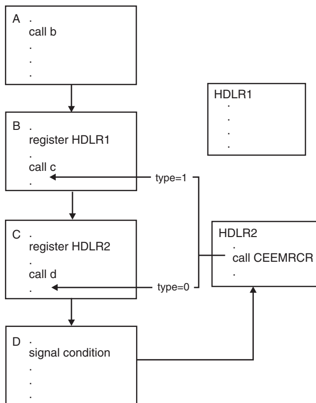
Figure 157. Second Example Moving Resume Cursor Using CEEMRCR
