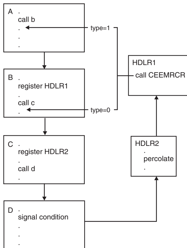
Figure 156. First Example Moving Resume Cursor Using CEEMRCR
