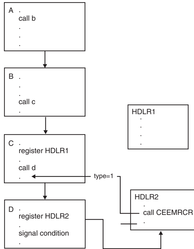
Figure 158. Third Example Moving Resume Cursor Using CEEMRCR
