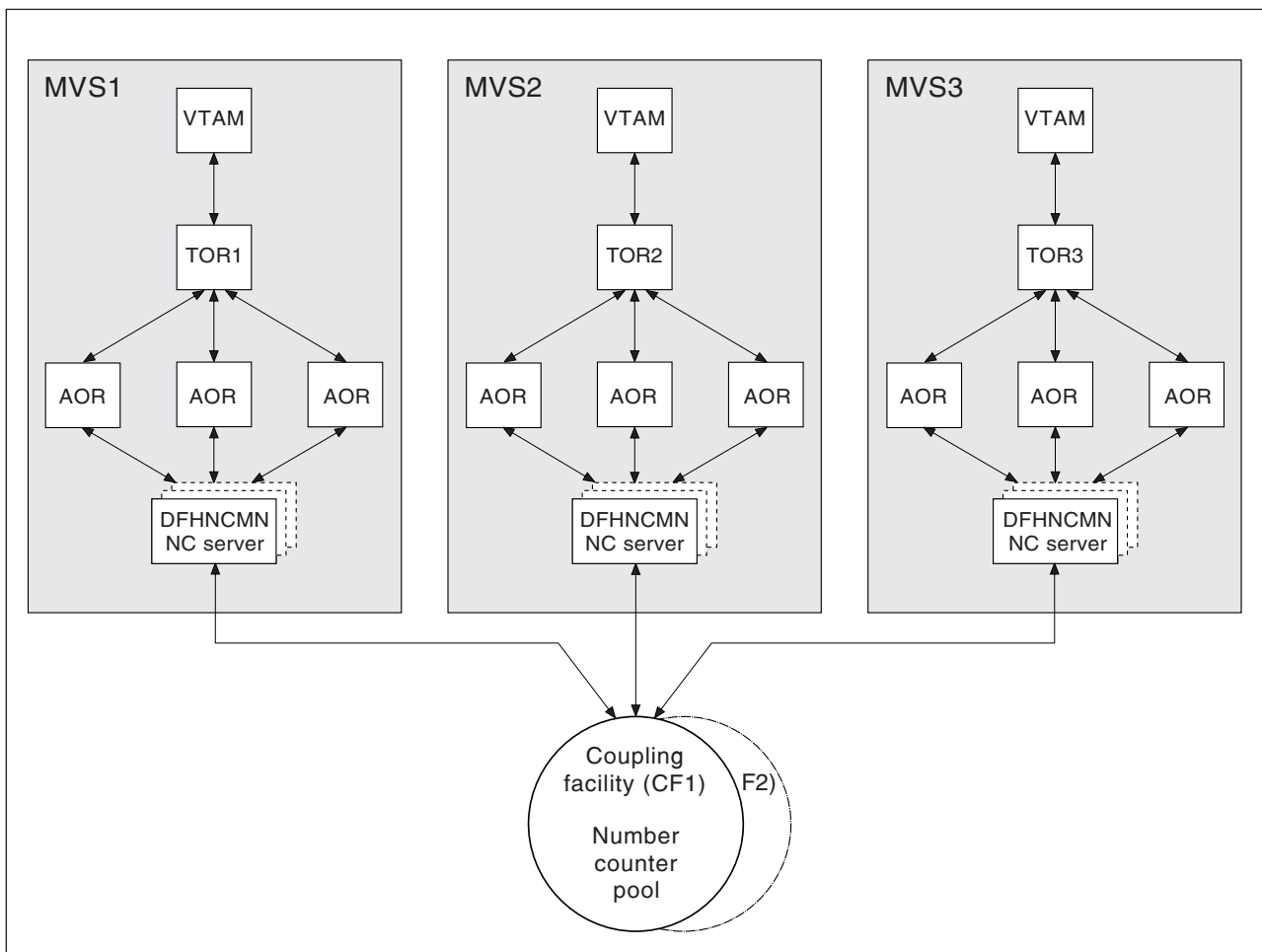
Figure 44. Conceptual view of a Parallel Sysplex with named counter servers
