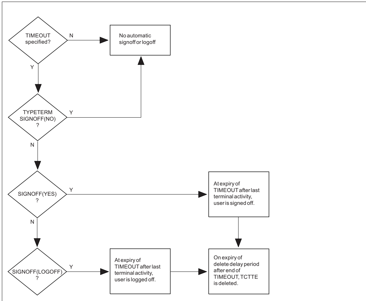
Figure 37. Automatic sign-off, logoff and deletion of autoinstalled terminals.
