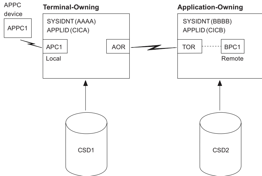
Figure 7. Maintaining local and remote definitions separately.
