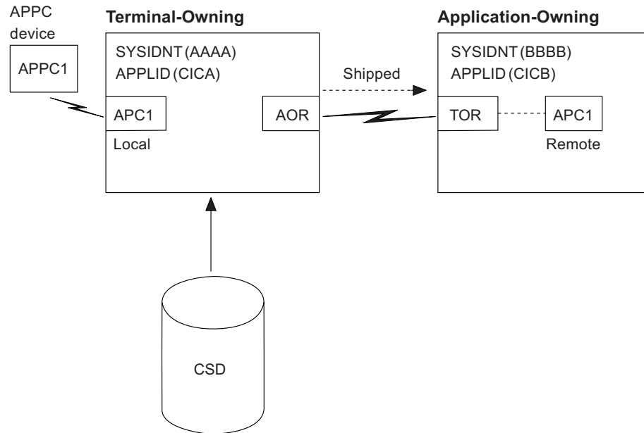
Figure 9. Shipping local definitions to an application-owning system.
