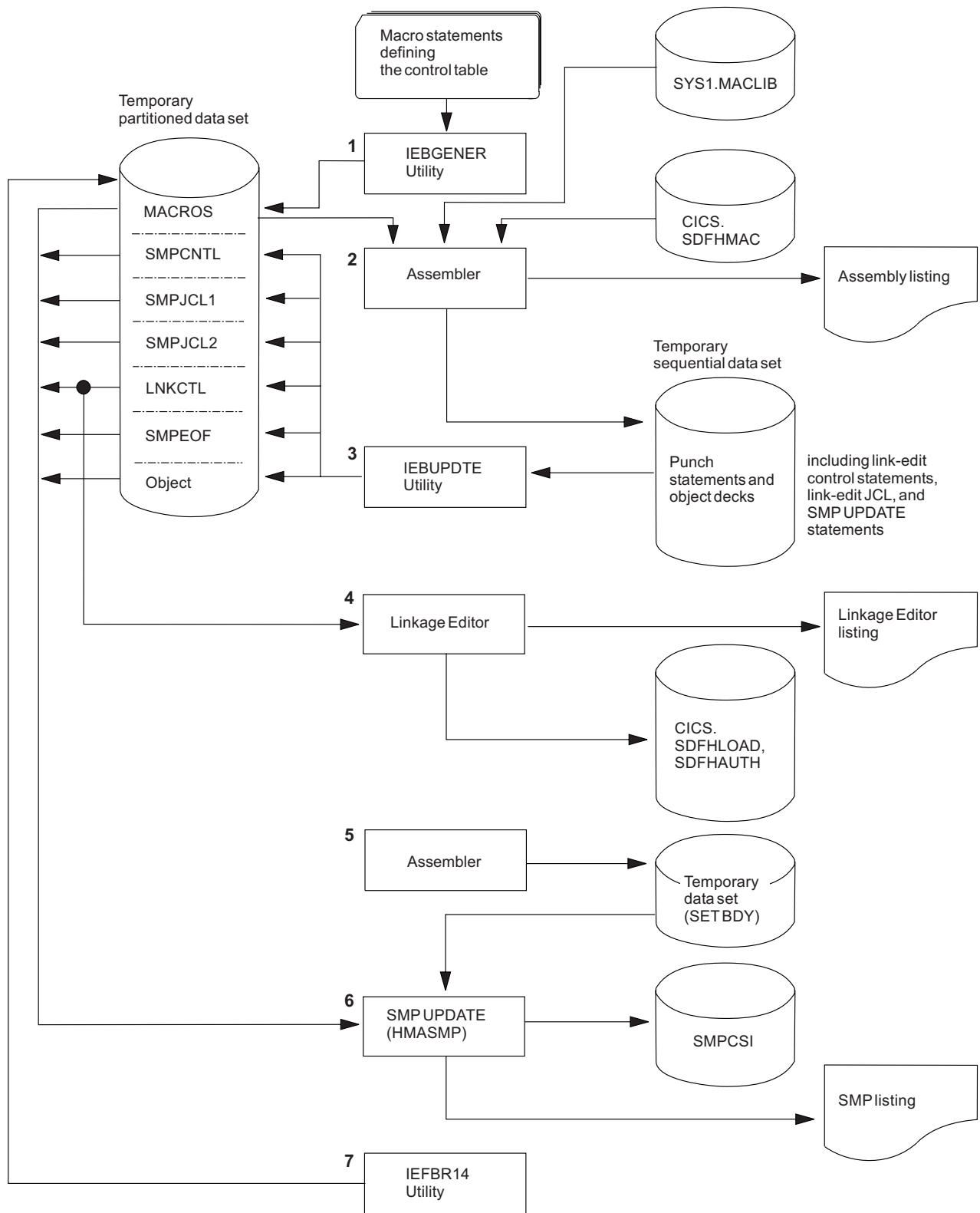
Figure 39. Assembling and link-editing the control tables using the DFHAUPLE procedure
