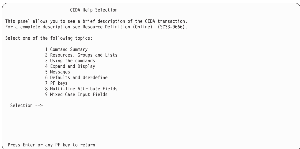
Figure 21. CEDA transaction: initial HELP panel
