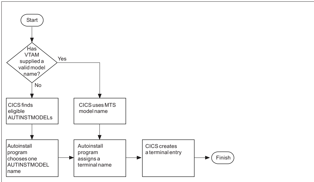
Figure 36. How CICS autoinstalls a terminal.
