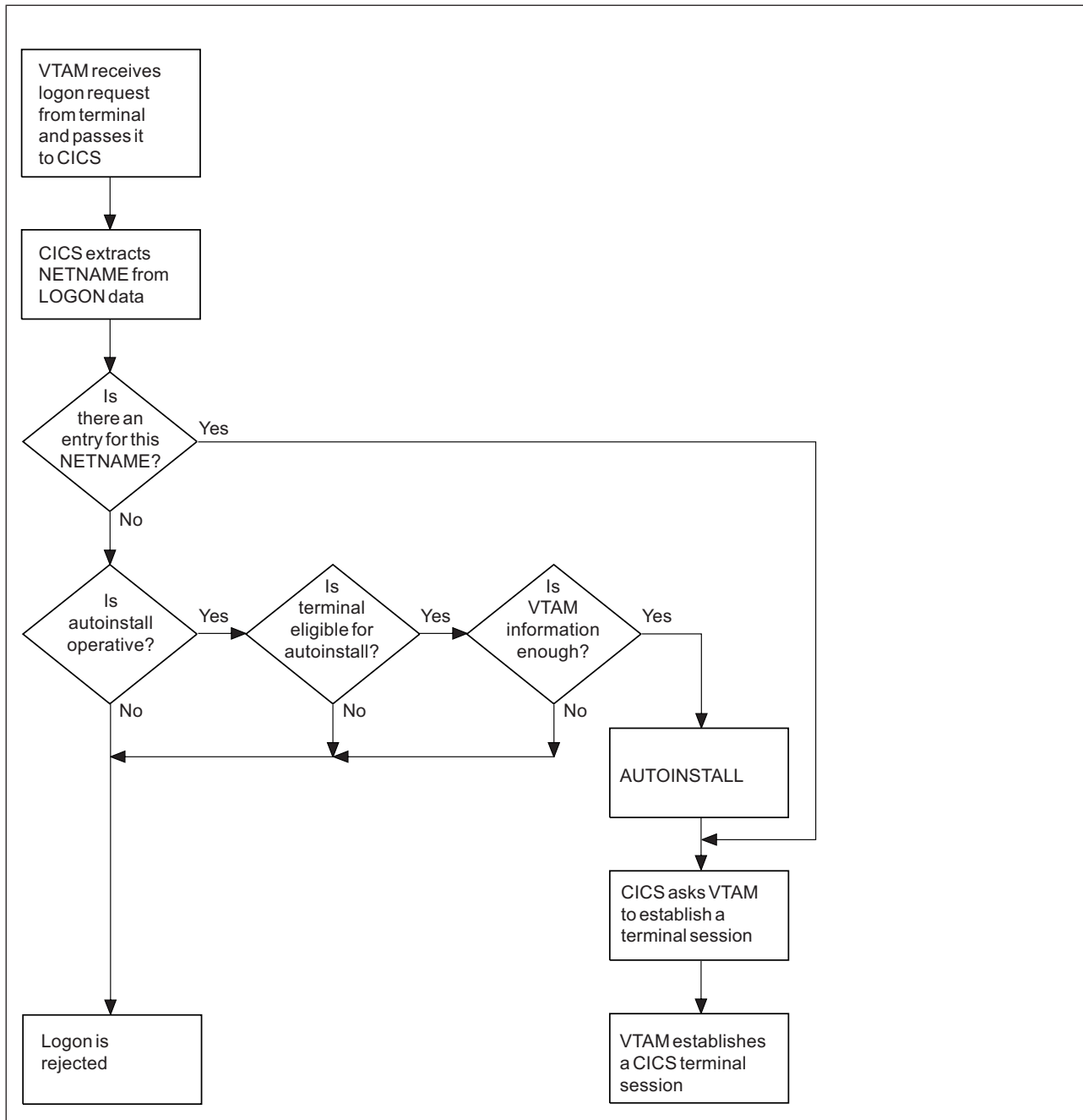
Figure 35. The process of logging on to CICS using autoinstall.
