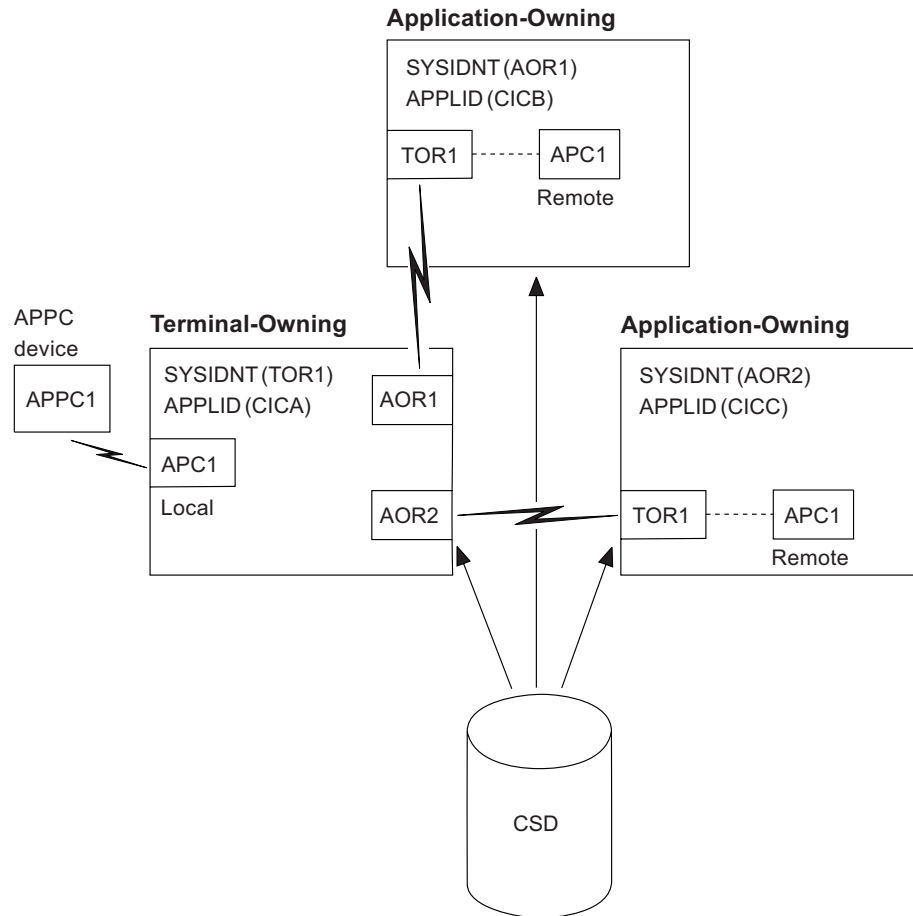
Figure 8. Sharing dual-purpose definitions.
