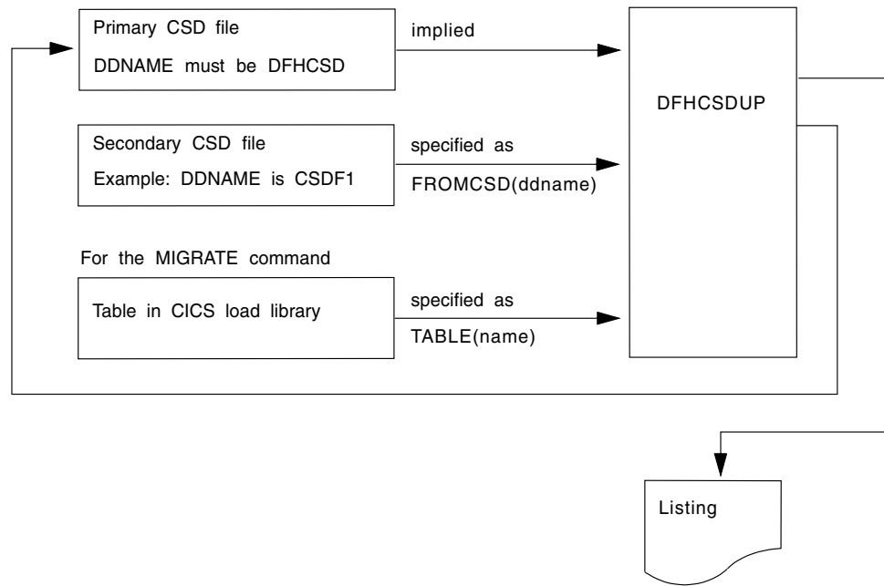
Figure 32. The DFHCSDUP offline utility program
