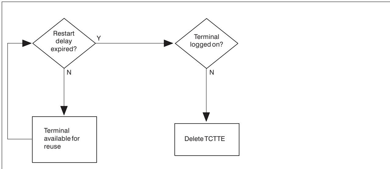
Figure 38. AUTOINSTALL—automatic logoff and TCTTE deletion after an emergency restart.
