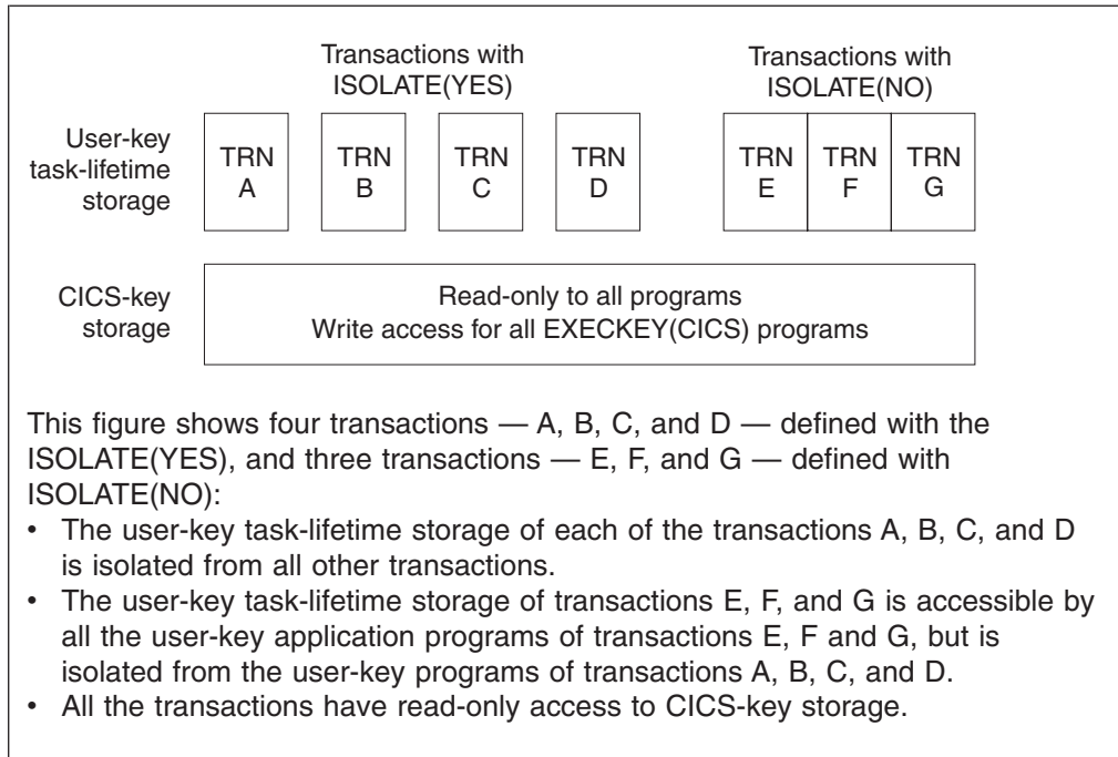
Figure 10. The effect of the ISOLATE attribute of storage access
