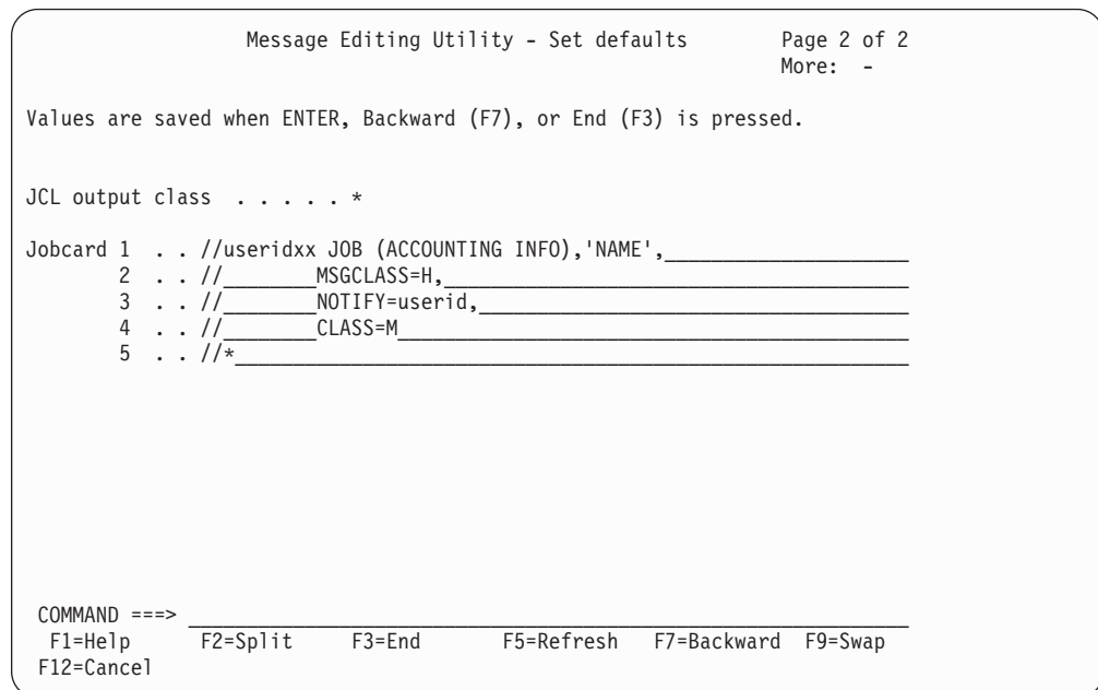
Figure 43. Message editing utility set defaults panel (2 of 2)
