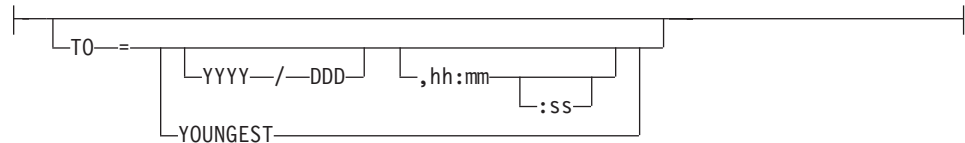
Figure 5. Log stream SUBSYS data set specification
