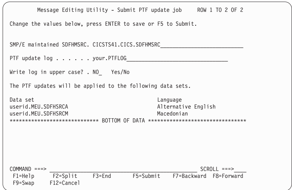
Figure 48. Message editing utility submit PTF update job panel
