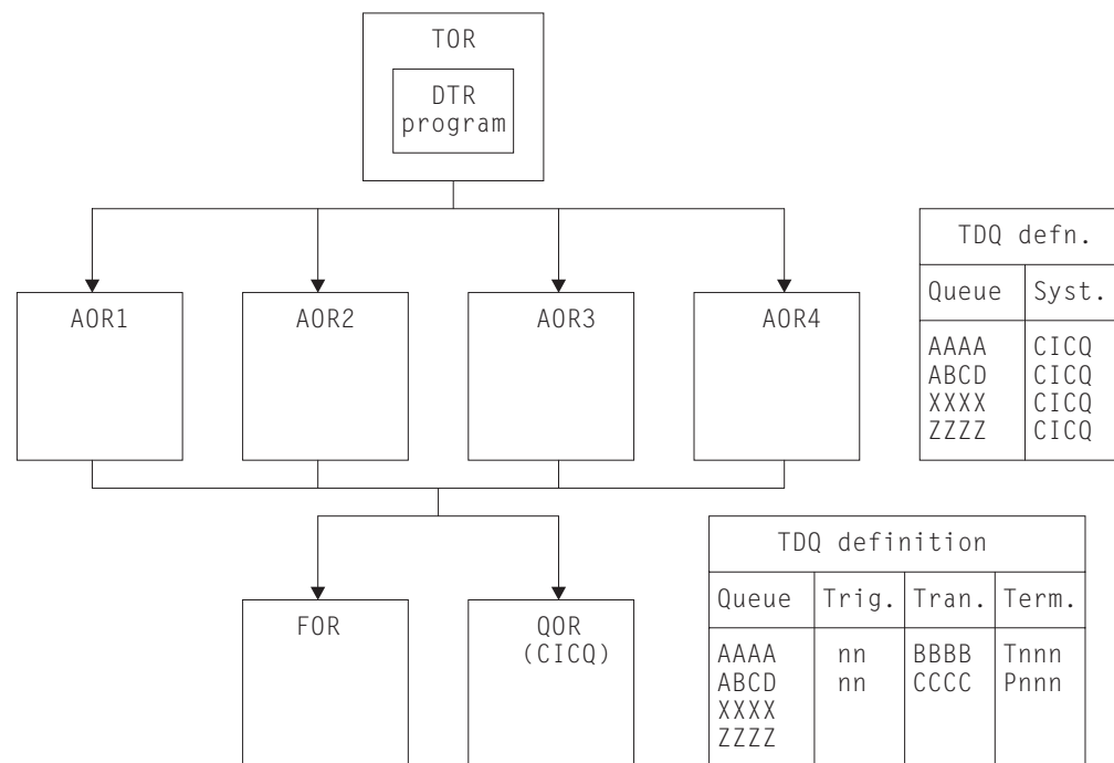
Figure 64. Using remote queues to avoid inter-transaction affinity relating to transient data. The transient data queue definitions installed in the target regions are defined as owned by the QOR (CICQ). All the transient data queue definitions installed in the QOR are local, some with trigger levels.
