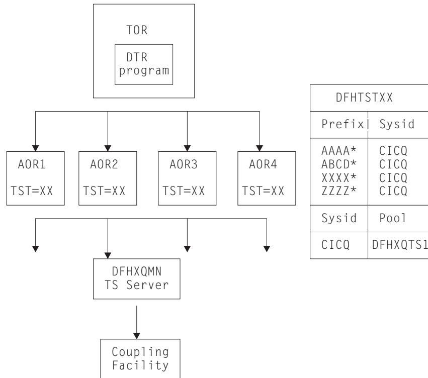
Figure 62. Example of the use of the temporary storage data-sharing server
