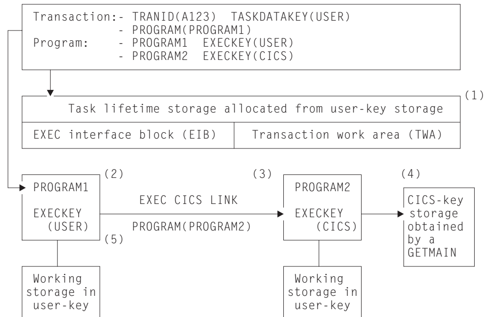
Figure 130. Illustration of the use of the TASKDATAKEY and EXECCKEY options
