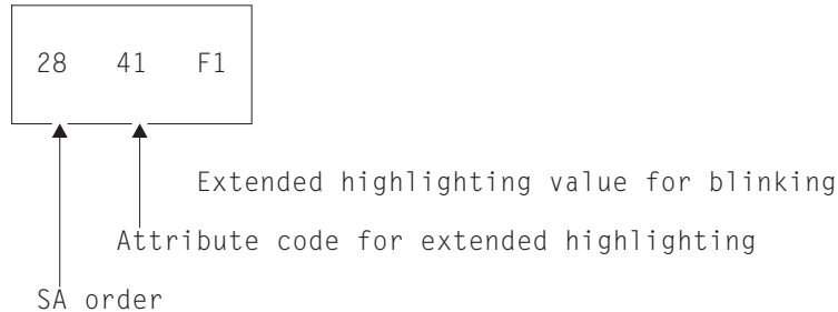
Figure 89. SA sequence to make a character blink
