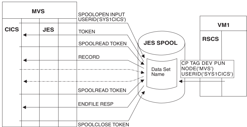
Figure 94. Retrieve data from the JES spool
