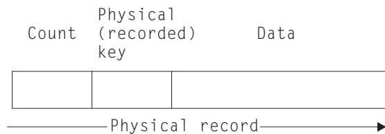
Figure 77. Format of unblocked records in a BDAM data set
