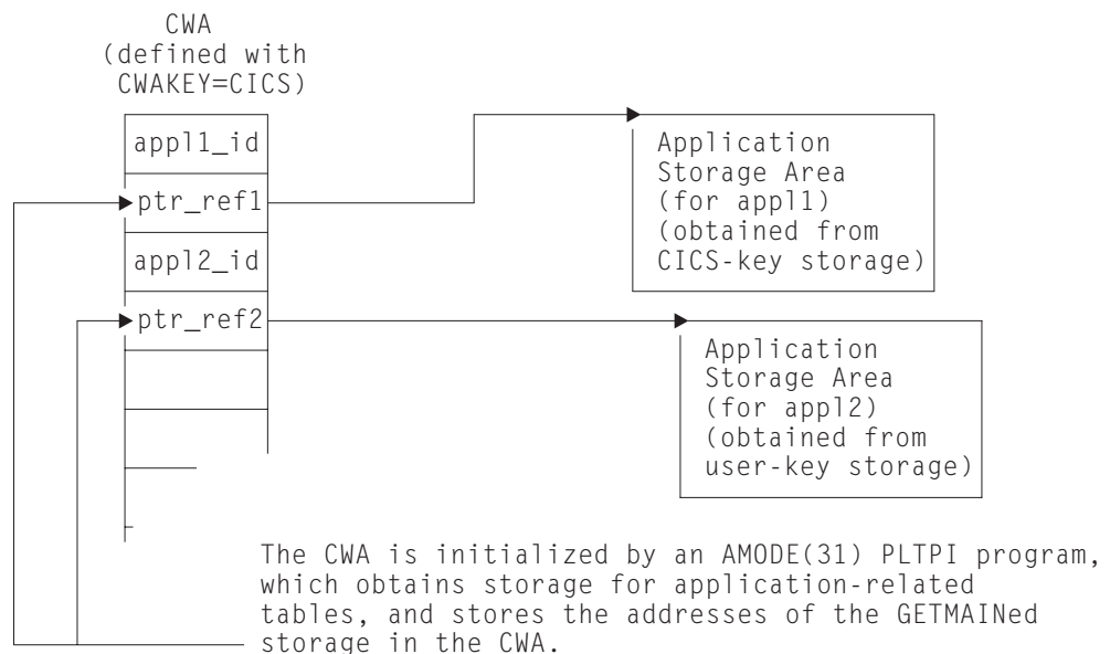
Figure 39. Example of use of CWA in CICS-key storage. This illustrates how the CWA can be used to reference storage that is obtained in user-key or CICS-key storage for use by application programs, while the CWA itself is protected by being in CICS-key storage.
