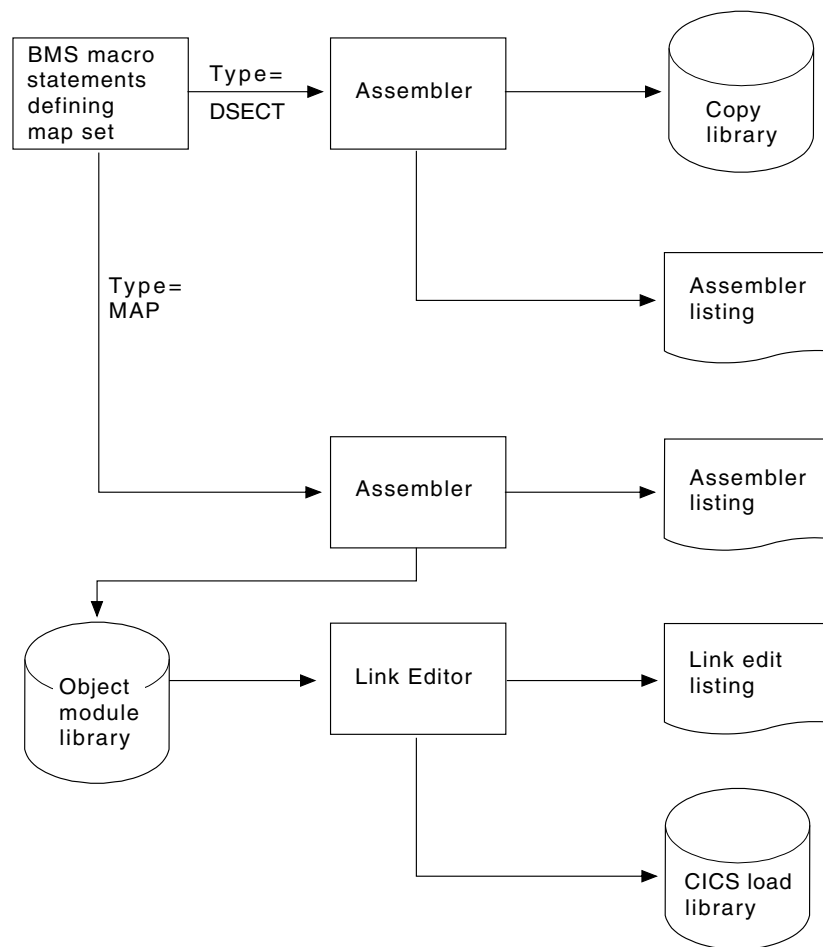
Figure 26. Preparing a map
