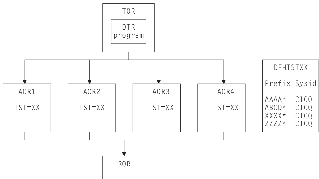
Figure 97. Using remote queues to avoid inter-transaction affinity relating to temporary storage. This example shows a combined file-owning and queue-owning region. Separate regions can be used, but these require special care during recovery operations because of 'indoubt' windows that can occur when recovering data managed independently by file control and temporary storage control.
