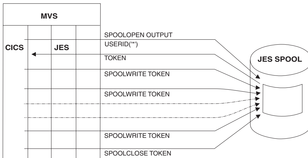
Figure 137. Create a file and write it to the JES spool
