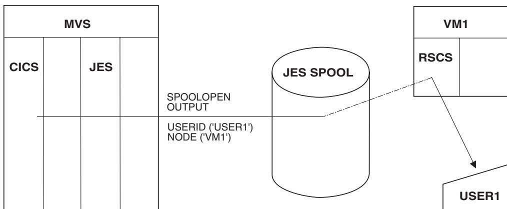
Figure 139. Send a written file to a remote destination
