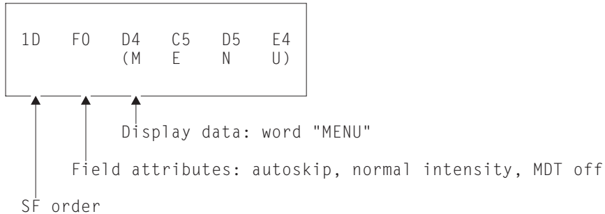
Figure 121. Field definition using SF order
