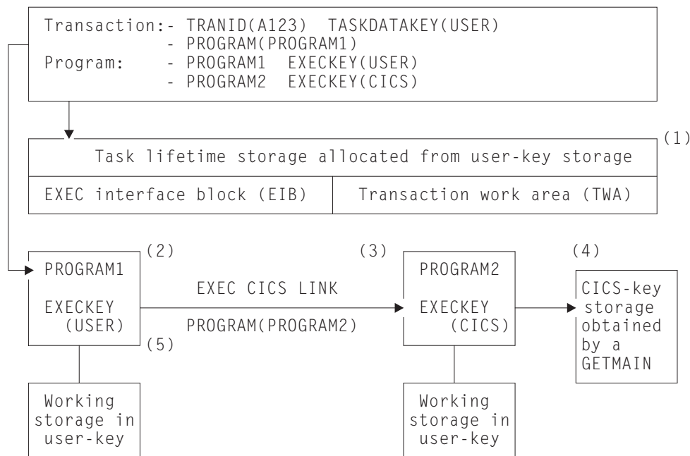
Figure 130. Illustration of the use of the TASKDATAKEY and EXECCKEY options
