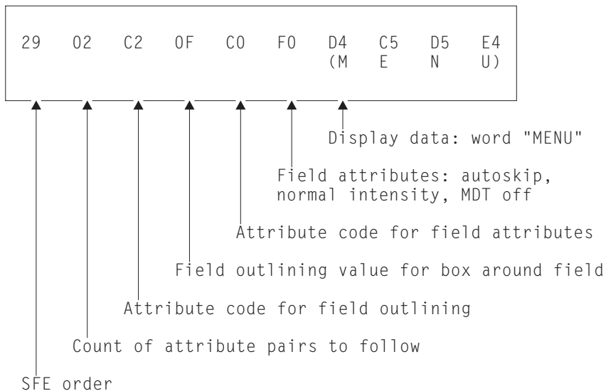
Figure 122. Field definition using SFE order
