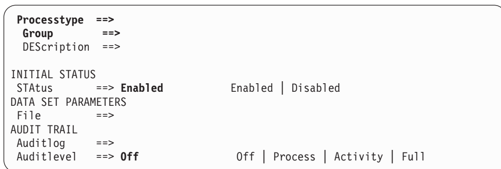
Figure 38. The DEFINE panel for PROCESSTYPE
