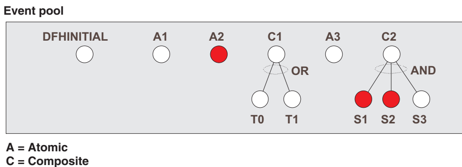
Figure 7. An event pool
