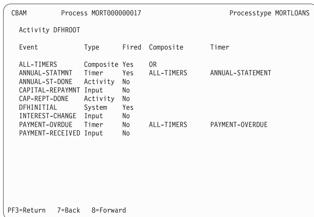
Figure 45. CBAM transaction: events screen
