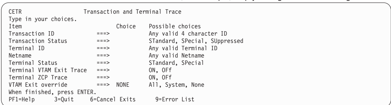
Figure 20. CETR screen for specifying standard and special task tracing
