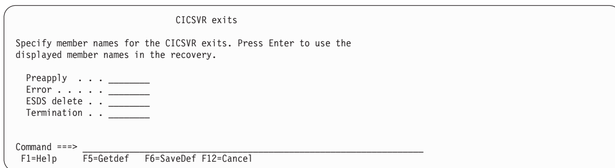
Figure 29. CICSVR exits
