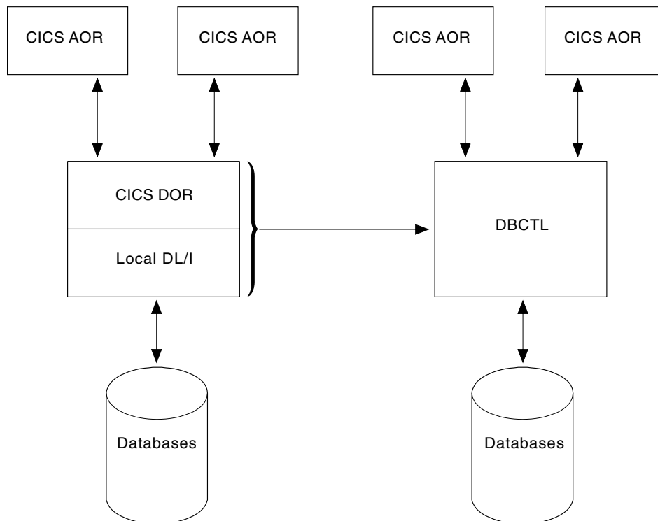
Figure 48. MRO installation with CICS DOR with DBCTL replacing local DL/I
