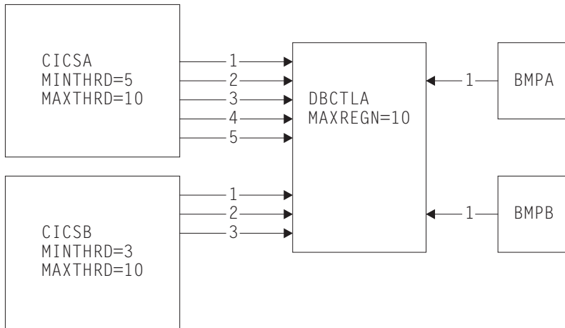
Figure 62. Interaction of MAXREGN, MINTHRD, and MAXTHRD
