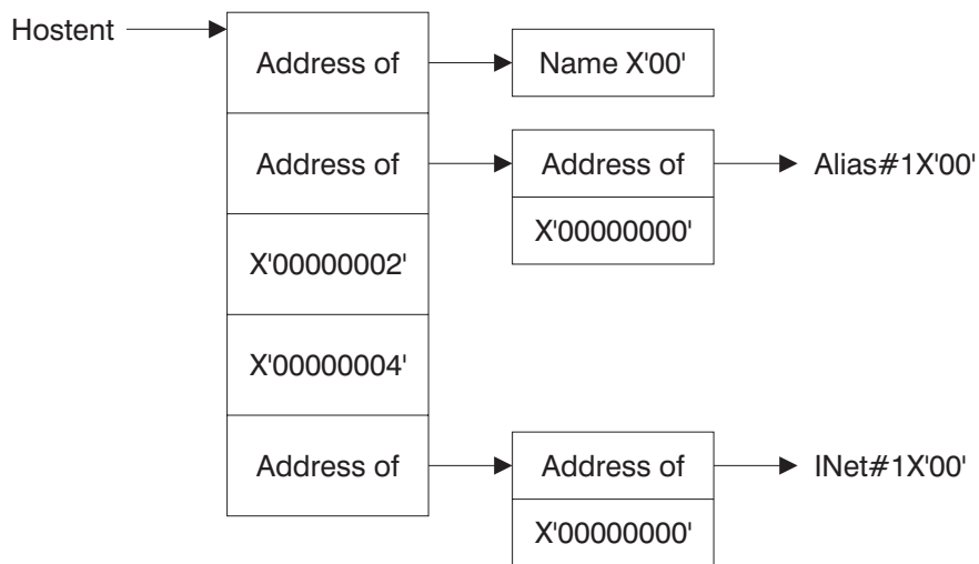
Figure 2. HOSTENT structure returned by the GETHOSTBYNAME call
