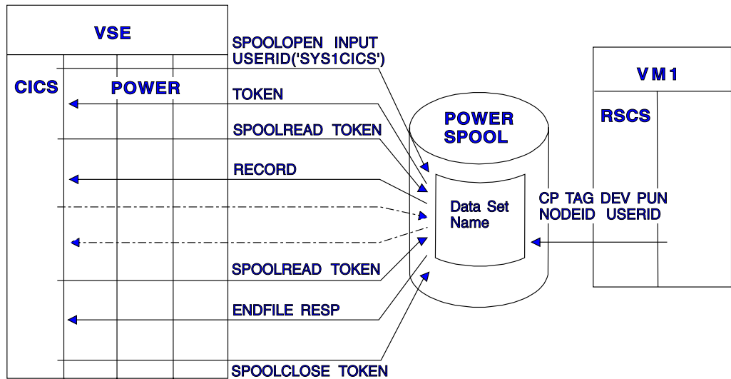
Figure 61. Retrieve data from the VSE/POWER spool
