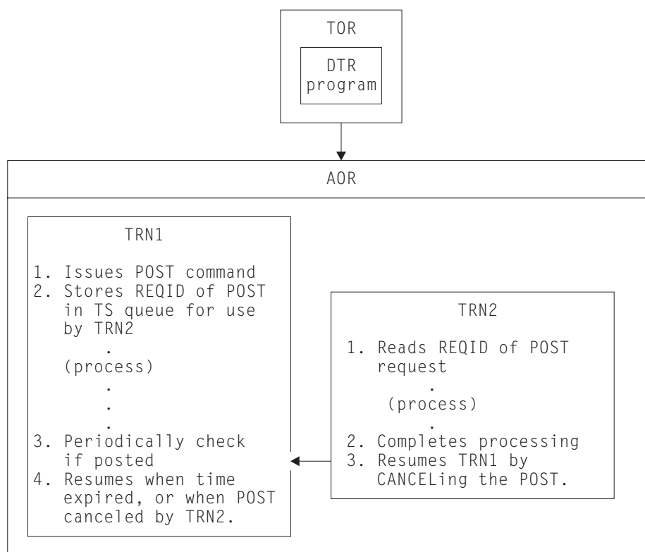
Figure 23. Illustration of the use of the EXEC CICS POST command
