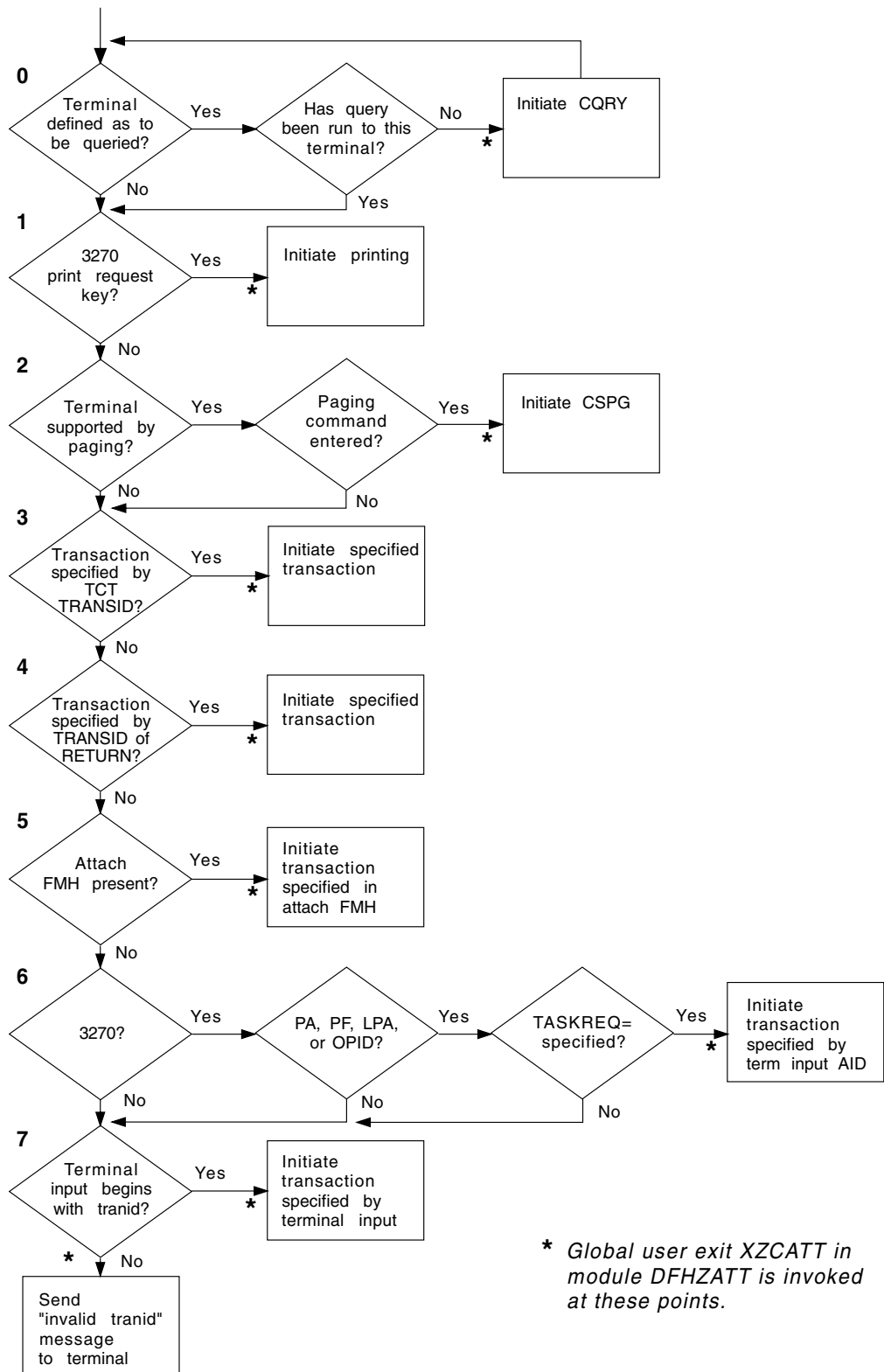
Figure 41. Determining which transaction to execute
