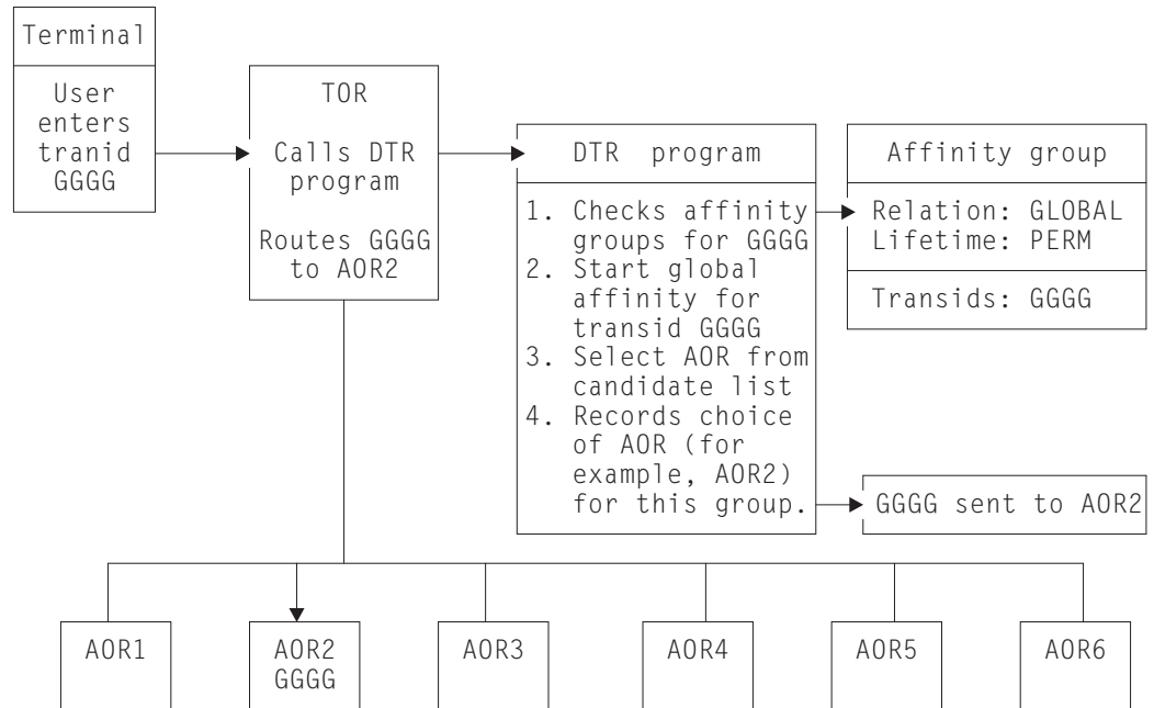
Figure 24. Managing intertransaction affinity with global relation and permanent lifetime. In this example, the first instance of tranid GGGG, from any terminal, starts a permanent-lifetime affinity. The first instance of GGGG can be routed to any suitable AOR (AOR1 thru AOR6), but all other instances, from any terminal, must be routed to whichever AOR is selected for GGGG.
