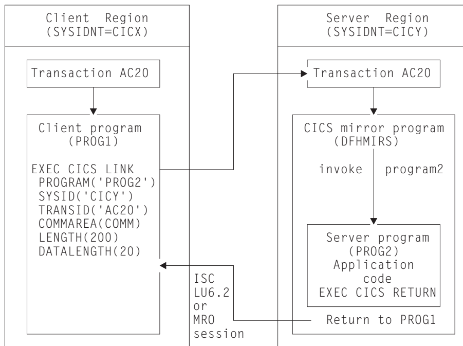
Figure 27. Illustration of distributed program link
