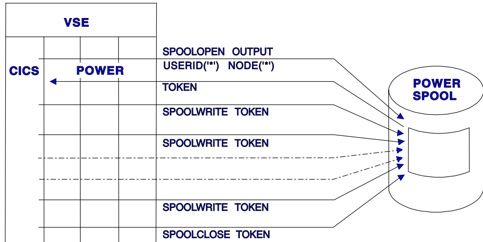
Figure 62. Create a file and write directly to the VSE/POWER spool. See also Figure 63 on page 359
