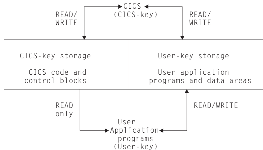
Figure 76. Protecting CICS code and control blocks from user application programs
