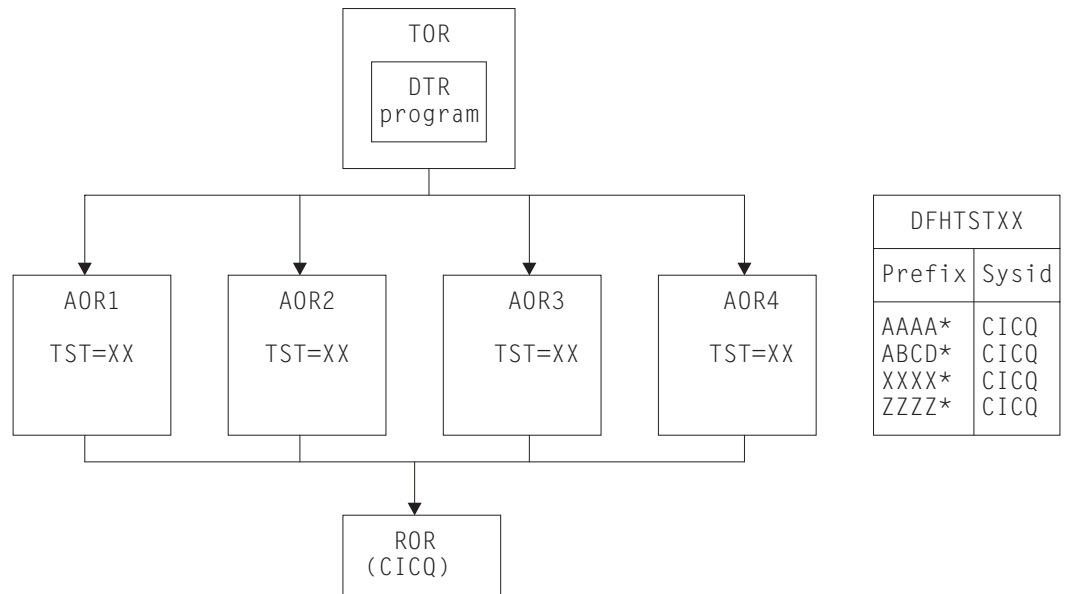
Figure 18. Using remote queues to avoid intertransaction affinity relating to temporary storage. This example shows a combined file-owning and queue-owning region. Separate regions can be used, but these require special care during recovery operations because of 'in-doubt' windows that can occur when recovering data managed independently by file control and temporary storage control.
