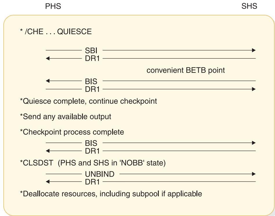
Figure 98. Example of PHS shutdown using SBI/BIS
