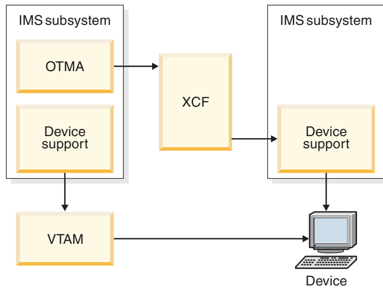
Figure 126. IMS communicates with a device using device support implemented within an OTMA client
