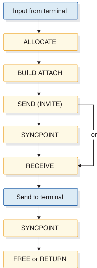
Figure 82. Application program flow using SEND/RECEIVE from CICS to IMS
