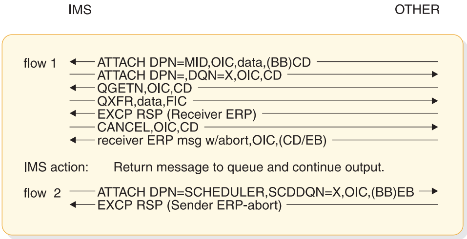
Figure 108. Example of demand-paged output with receiver-detected error
