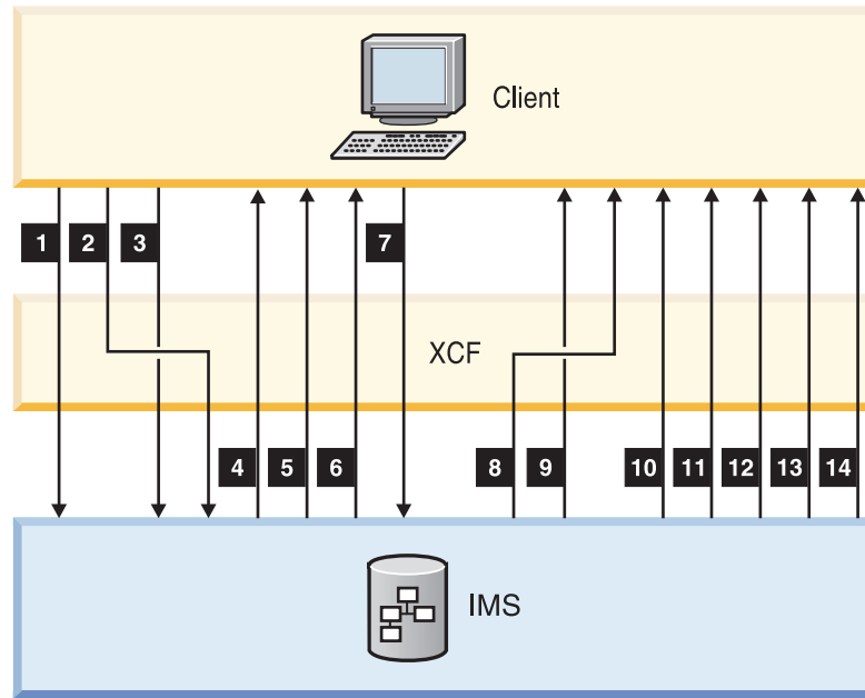
Figure 143. Sample message flow for send-then-commit flow
