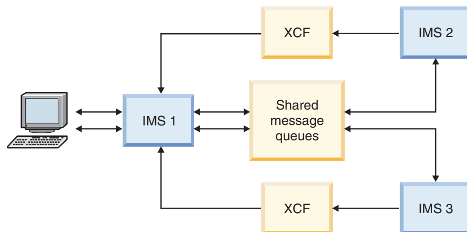
Figure 135. OTMA messages being processed on multiple IMS systems in a shared-queues group
