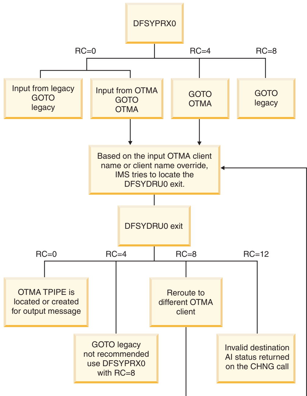
Figure 134. How DFSYPRX0 and DFSYDRU0 determine message destination
