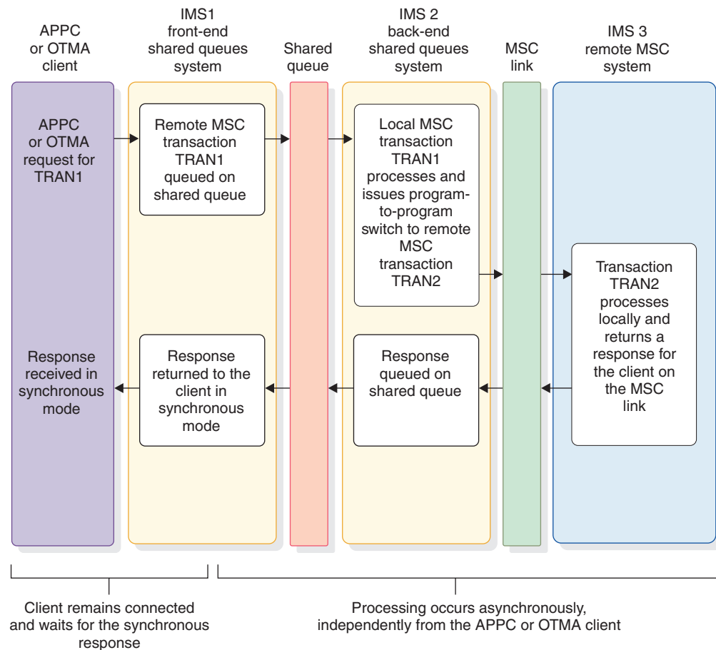
Figure 124. APPC or OTMA transaction routed using MSC and shared queues with a program-to-program switch
