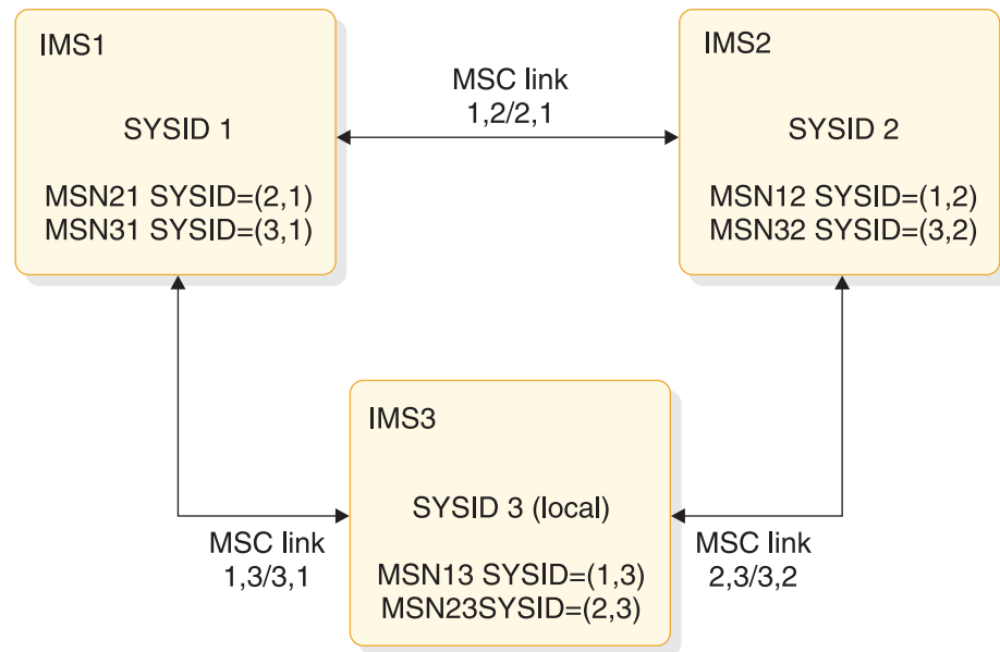
Figure 119. MSC network without an IMSplex
