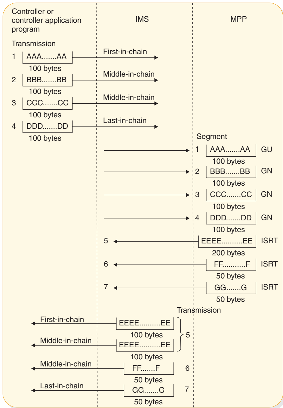
Figure 153. Chained message interaction between a Finance Communication system and an IMS MPP
