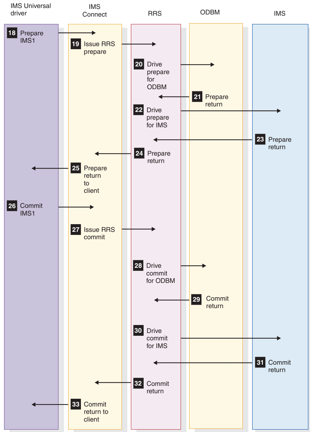
Figure 34. Distributed two-phase commit global transaction client flow for IMS Universal drivers (2 of 2)
