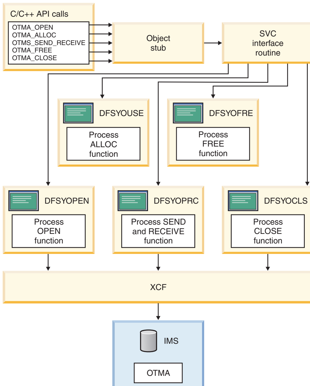
Figure 151. OTMA Callable Interface overview
