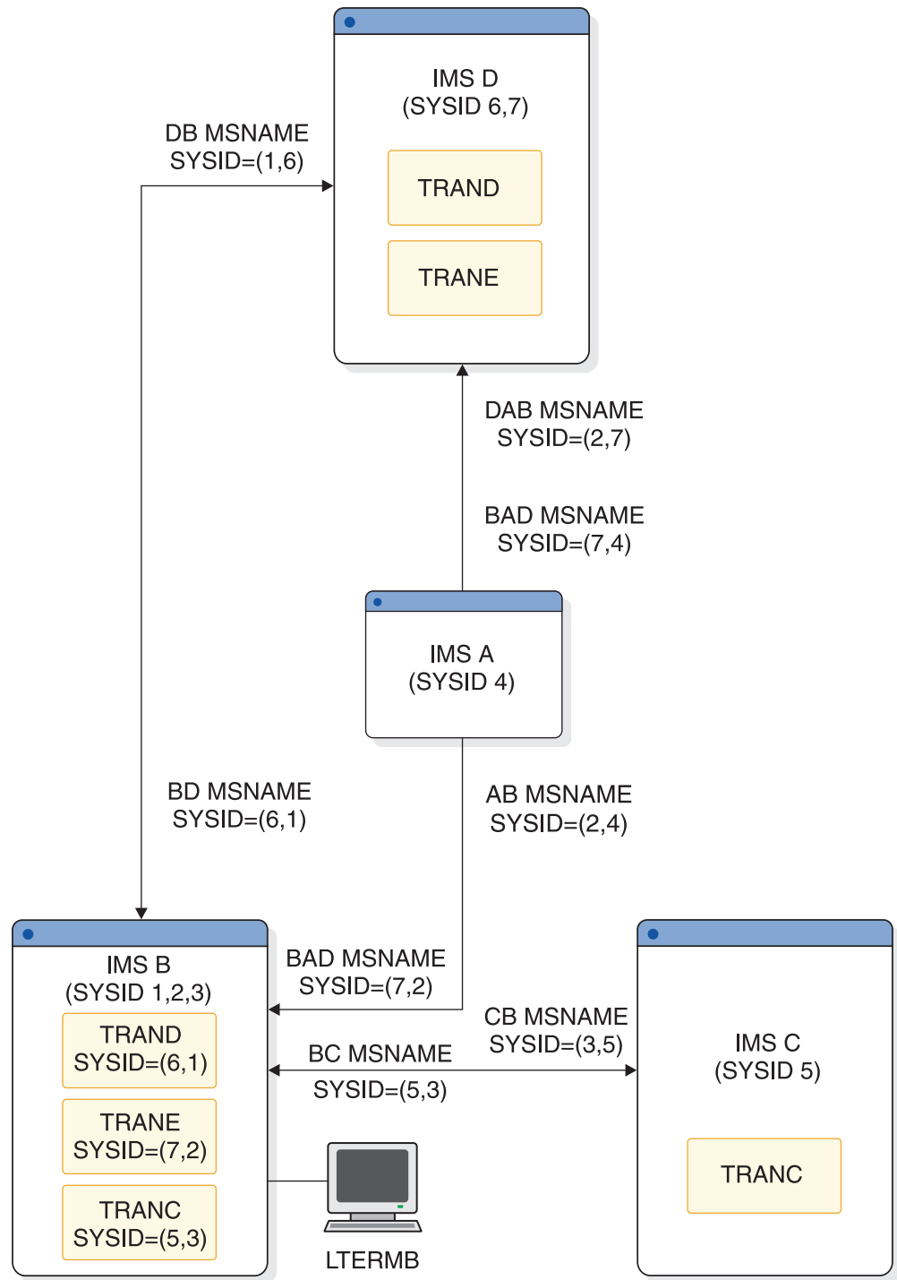
Figure 115. System identifiers (SYSIDs)
