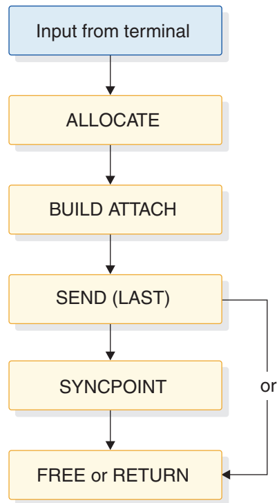
Figure 83. Application program flow using SEND LAST from CICS to IMS
