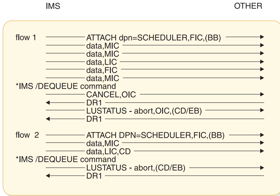
Figure 103. Example of sender-detected error while sending autopaged output message
