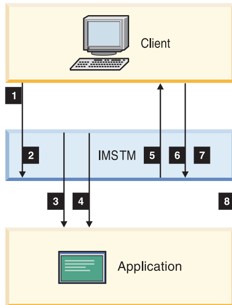
Figure 144. Send-then-commit with confirm flow
