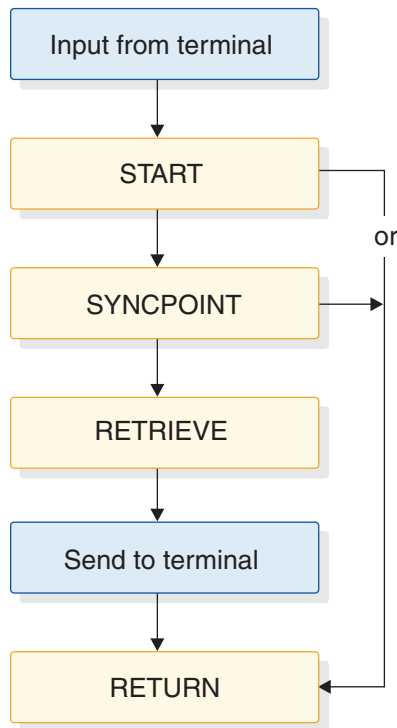
Figure 85. Application program flow using START/RETRIEVE from CICS to IMS
