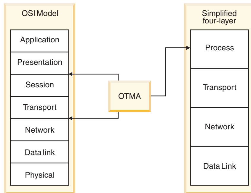
Figure 125. Network architecture models
