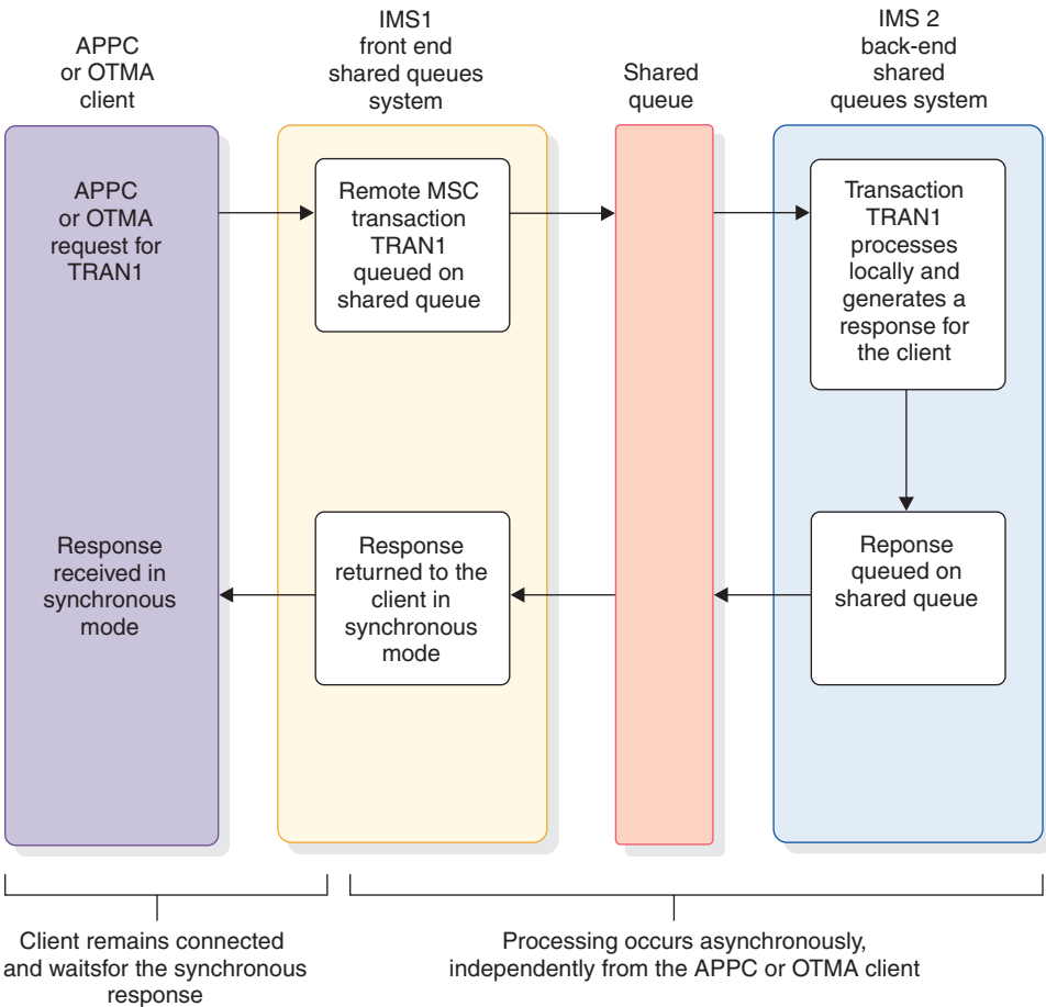
Figure 121. Using a remote MSC transaction to route an APPC or OTMA transactions to a back-end IMS system
