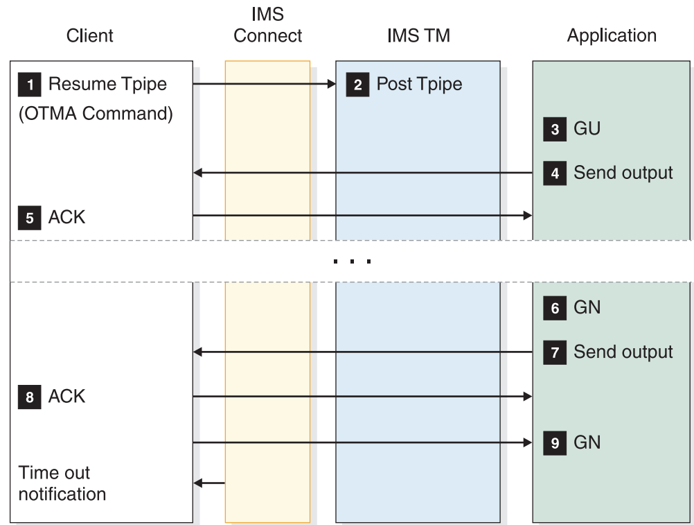
Figure 31. Commit-then-send, receive asynchronous output (client waits for output) flow
