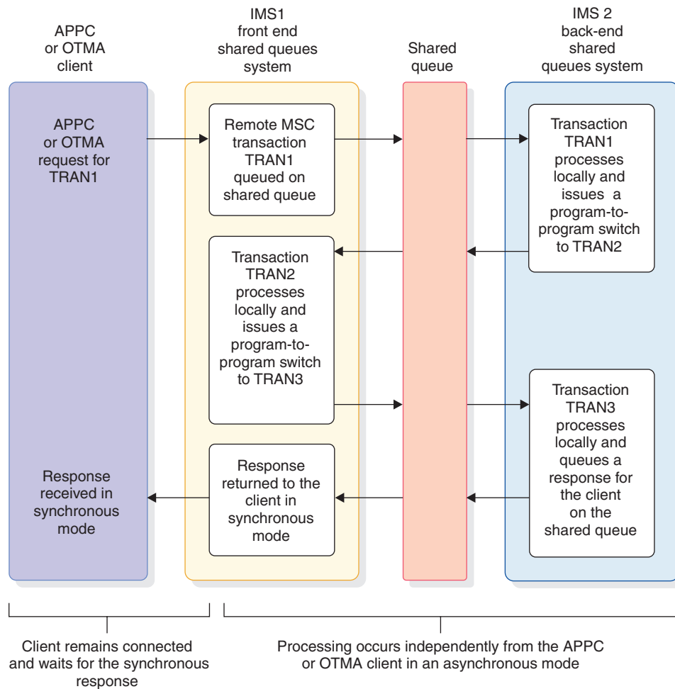
Figure 123. Routing an APPC or OTMA transaction by using a remote MSC transaction and shared queues with multiple program-to-program switches
