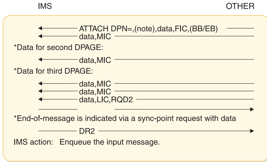
Figure 97. Example of autopaged input, single transmission chain
