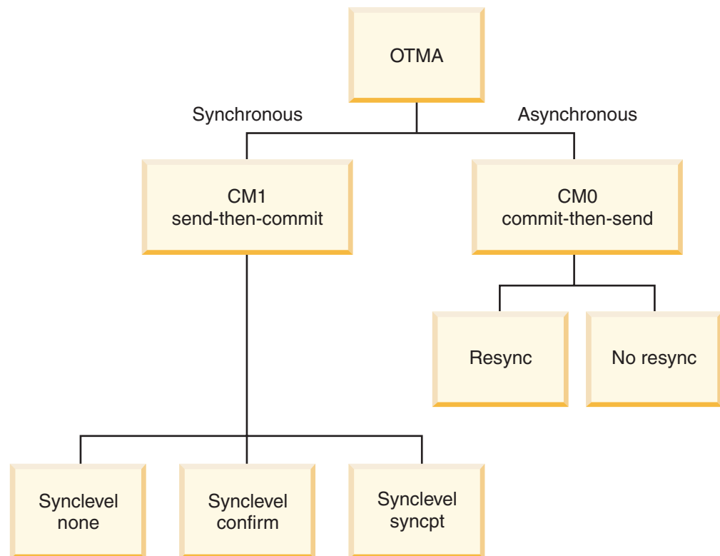
Figure 136. Synchronous and asynchronous transactions and their respective commit levels
