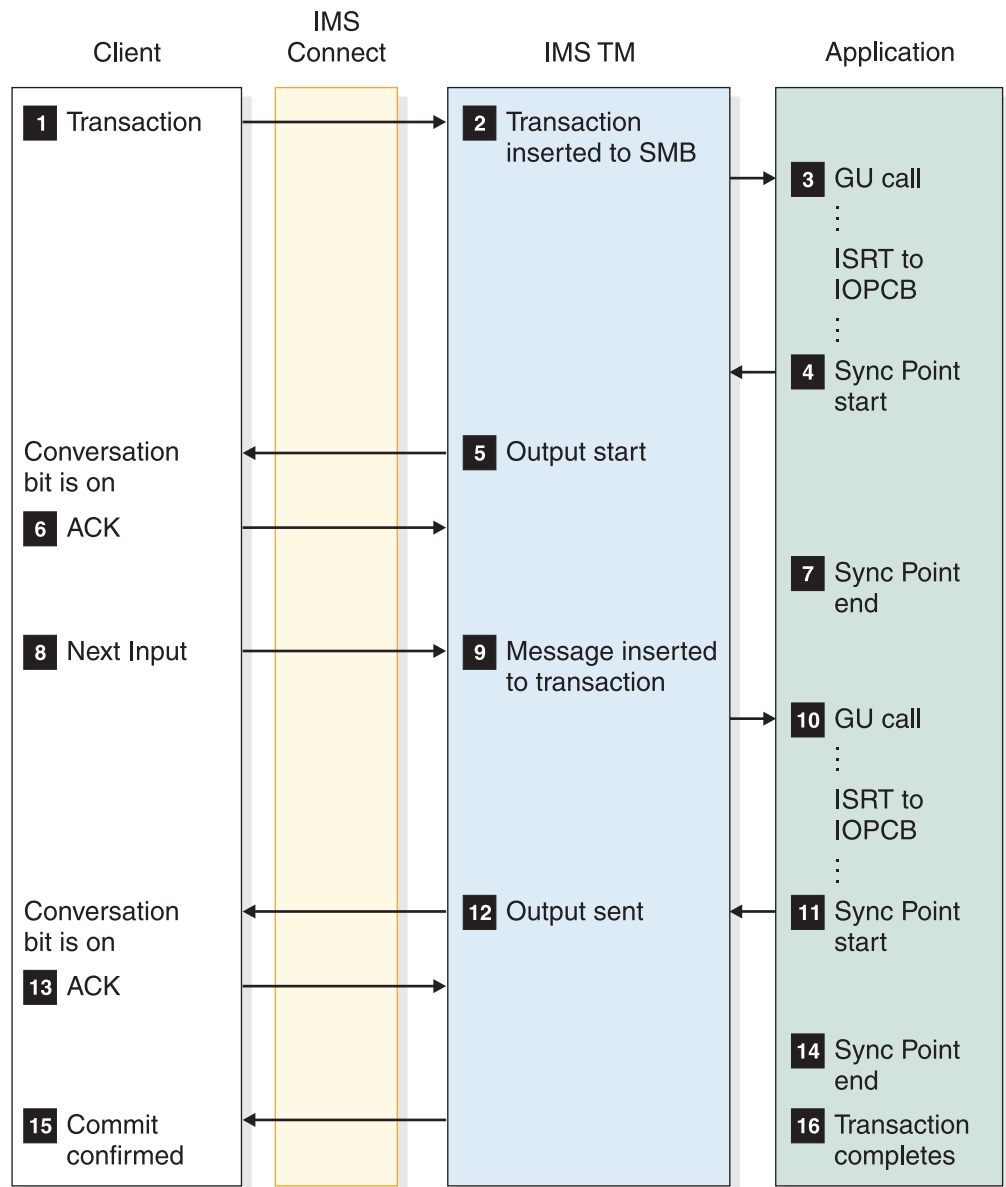
Figure 28. Send-then-commit, sync level=confirm (ACK response) flow
