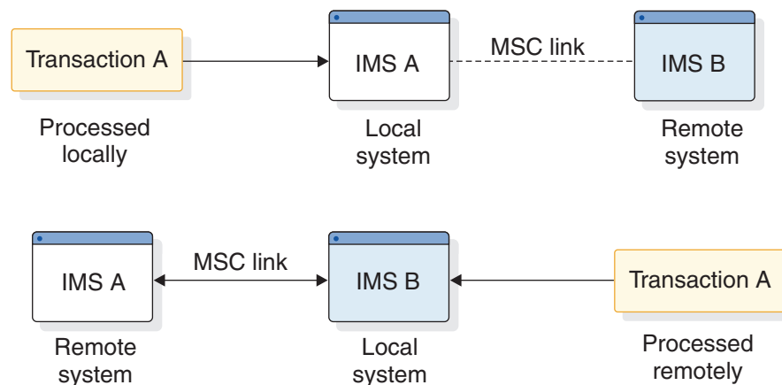
Figure 110. Remote and local transactions and systems
