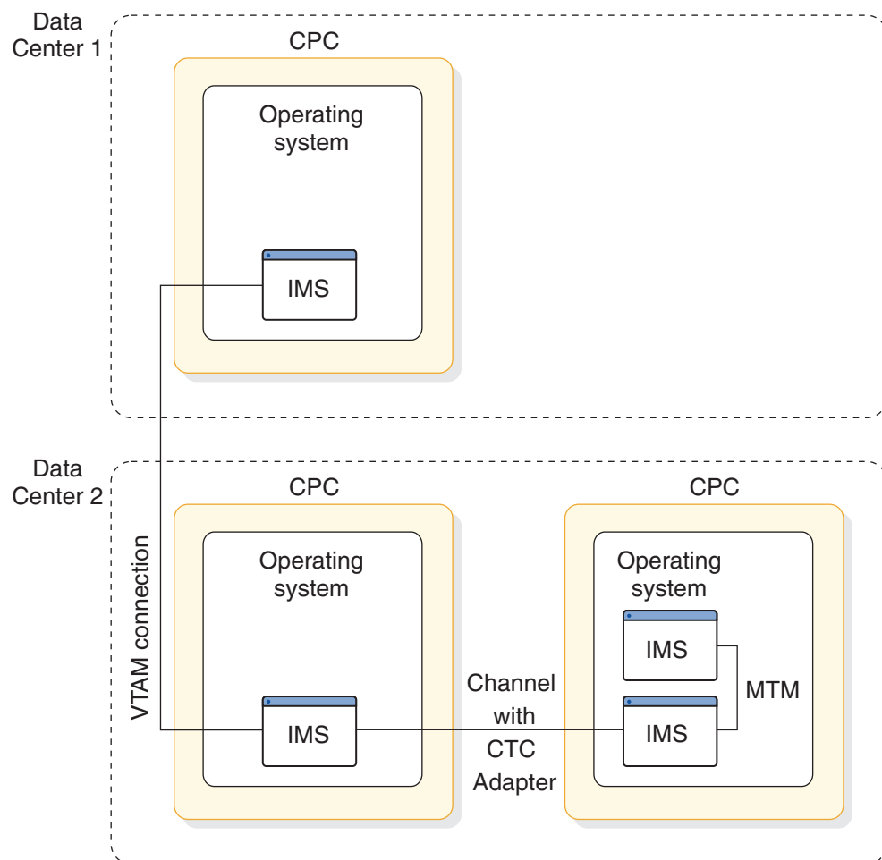
Figure 109. MSC physical link types
