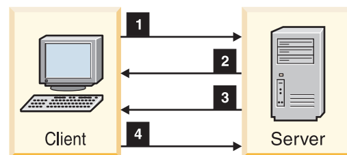
Figure 147. Commit-then-send transaction flow
