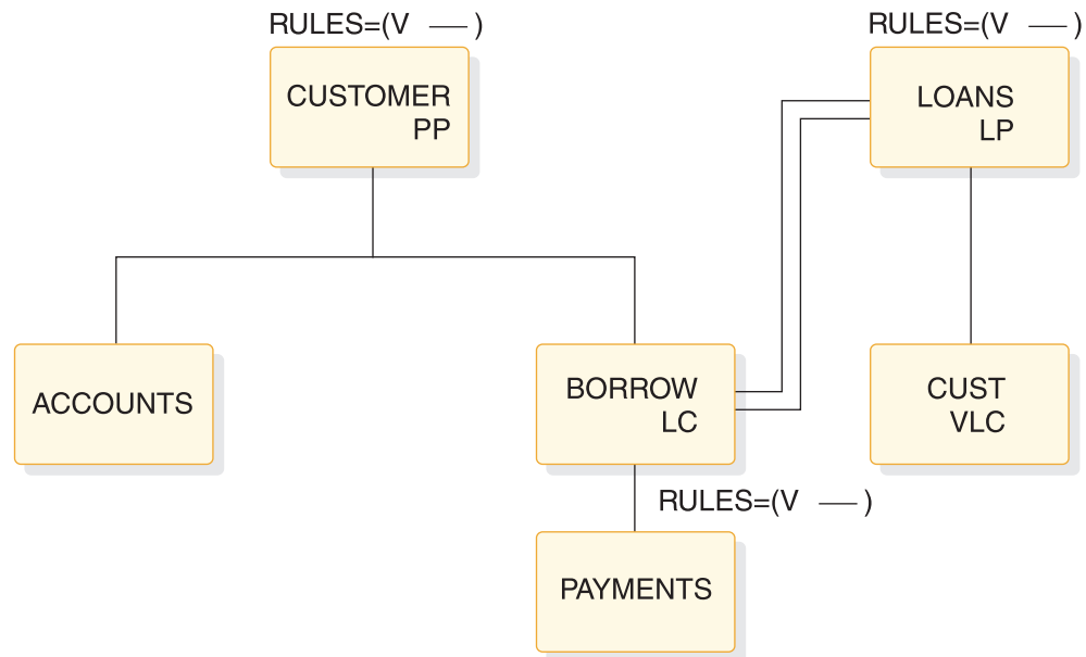
Figure 105. Virtual insert rule example
