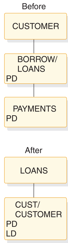
Figure 144. Logical child, physical pairing—physical or logical delete rule example: before and after
