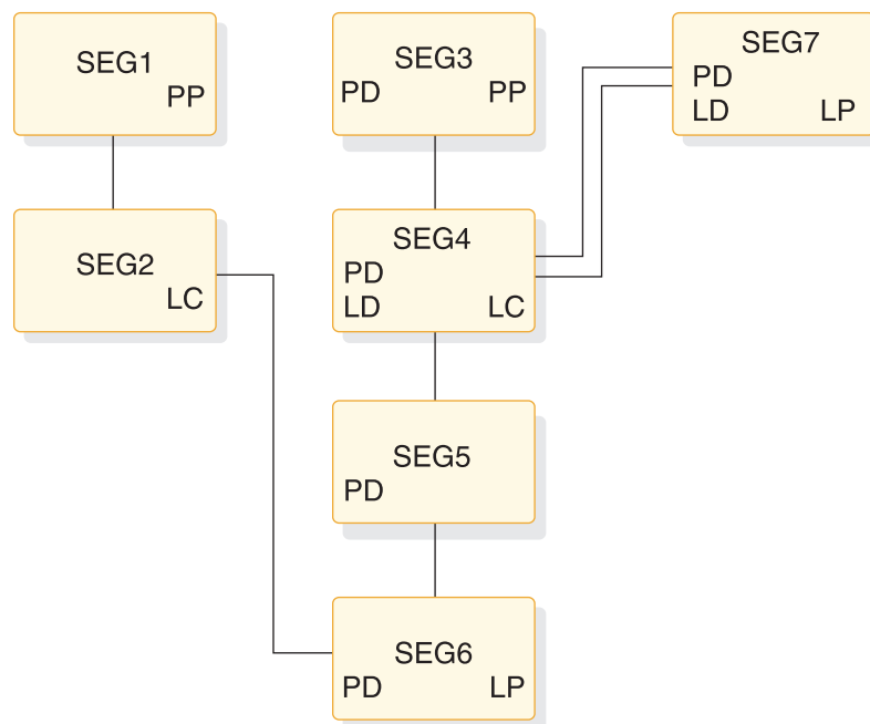
Figure 156. Example of abnormal termination
