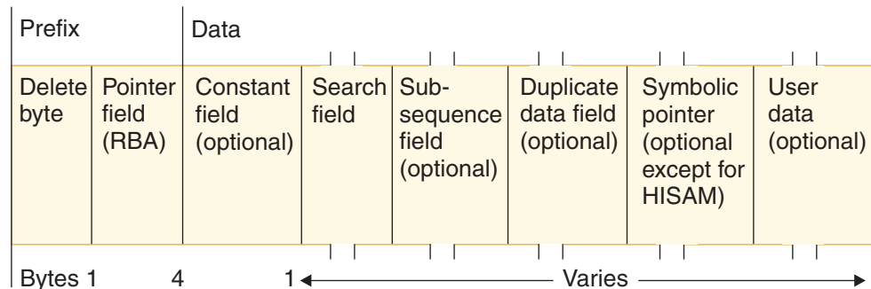
Figure 177. Fields of a pointer segment in a secondary index
