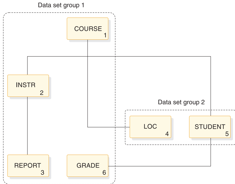
Figure 206. Second example of data set groups
