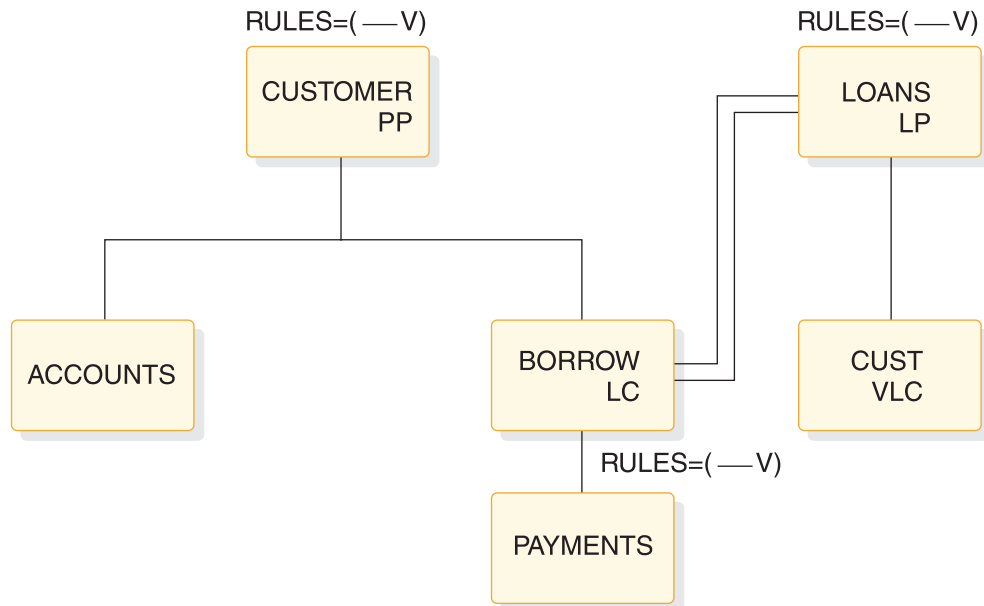
Figure 113. Virtual replace rule example
