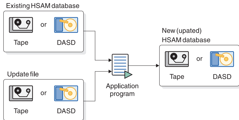
Figure 20. Updating an HSAM database
