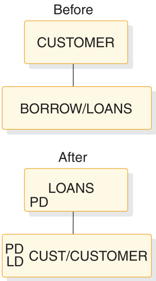
Figure 128. Logical parent, virtual pairing—virtual delete rule example: before and after
