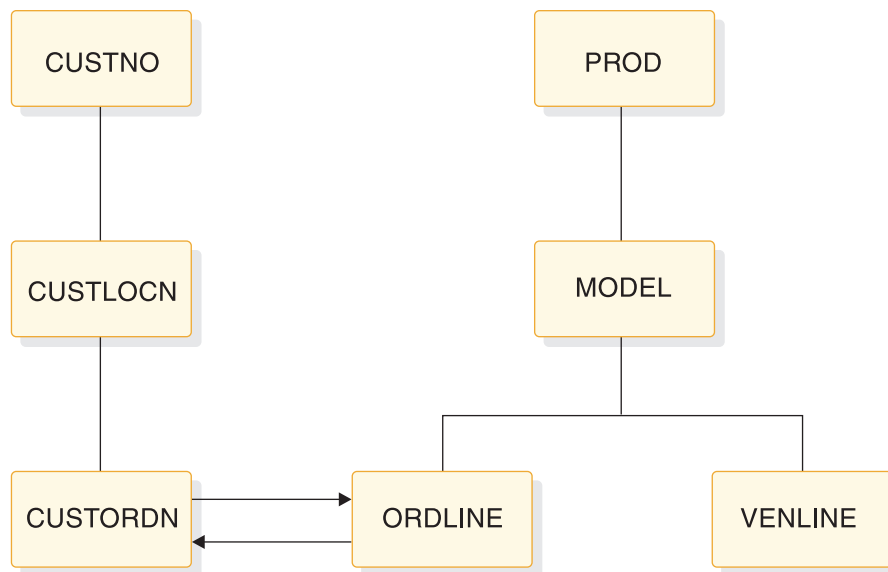
Figure 70. Example of a segment that appears to have two parents
