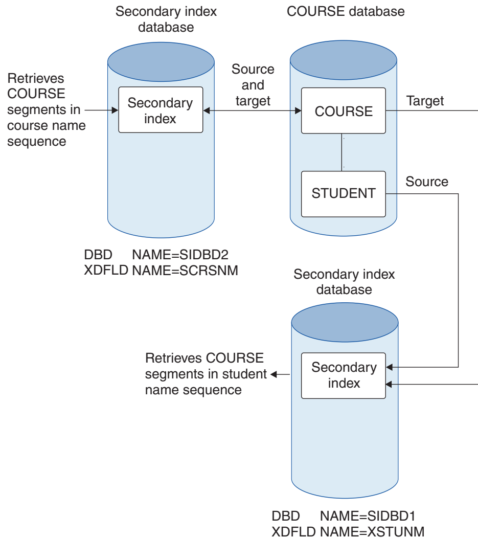
Figure 183. Databases for second example of the INDICES= parameter
