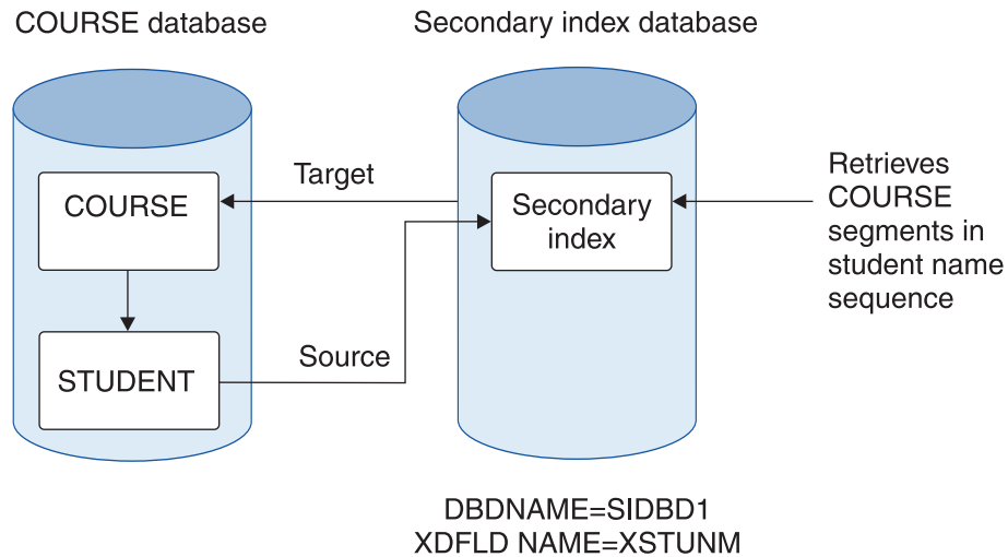
Figure 180. Databases for first example of the INDICES= parameter
