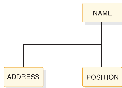
Figure 16. Payroll database record with SALARY segment masked
