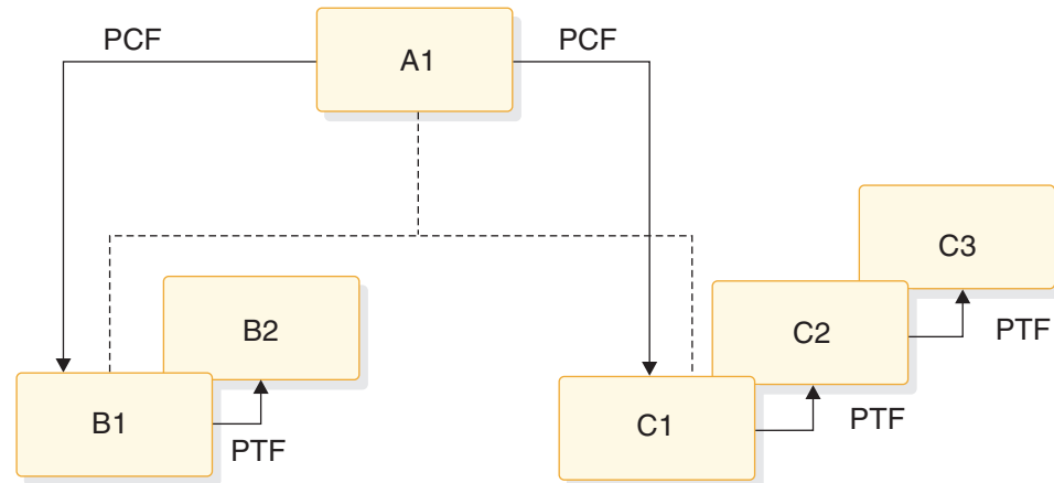
Figure 53. How dependent segments are found using PCF and PTF pointers
