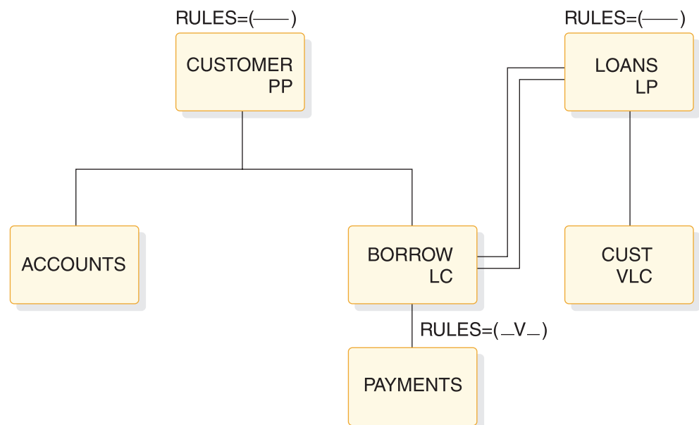
Figure 145. Logical child, virtual pairing—virtual delete rule example
