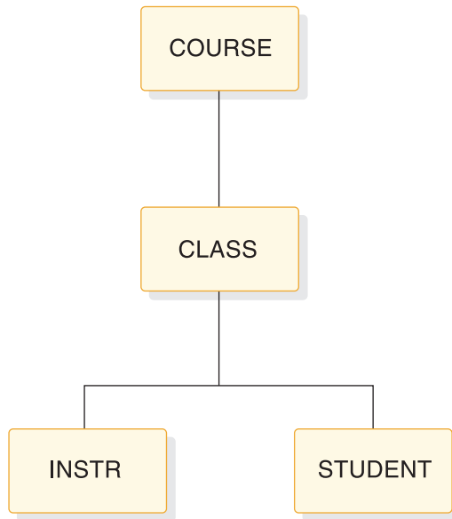
Figure 170. Education database record
