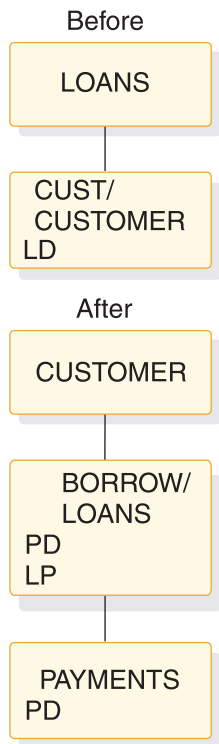
Figure 138. Logical child, virtual pairing—physical delete rule example: before and after
