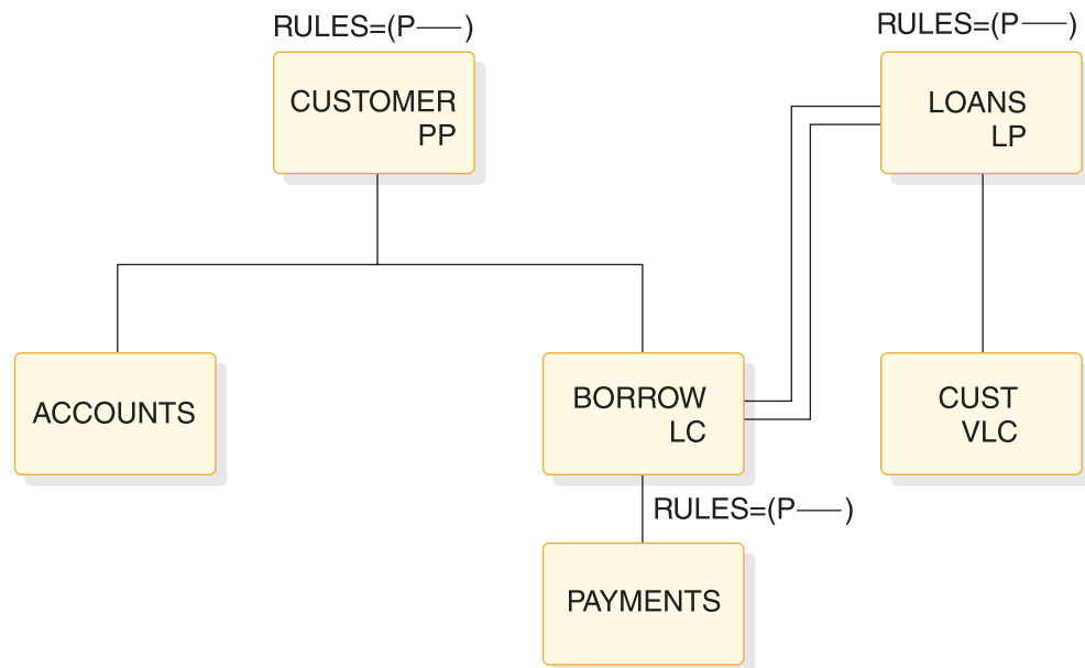
Figure 100. Physical insert rule example
