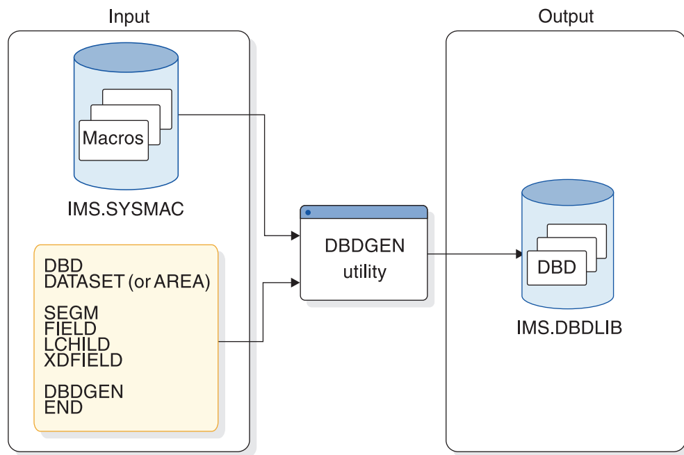
Figure 228. The DBD generation process
