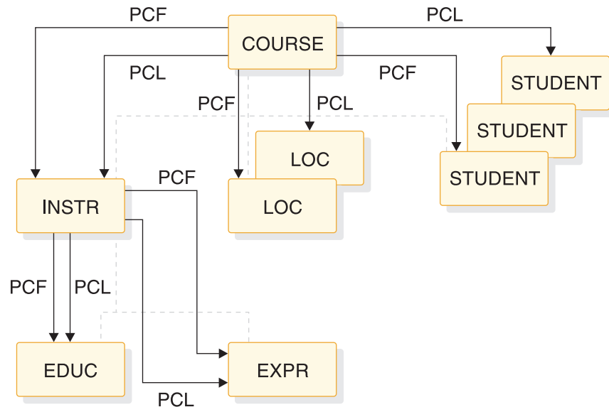
Figure 37. Physical child first and last pointers
