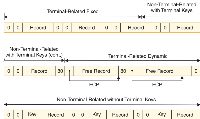
Figure 65. Sequence of the four MSDB organizations
