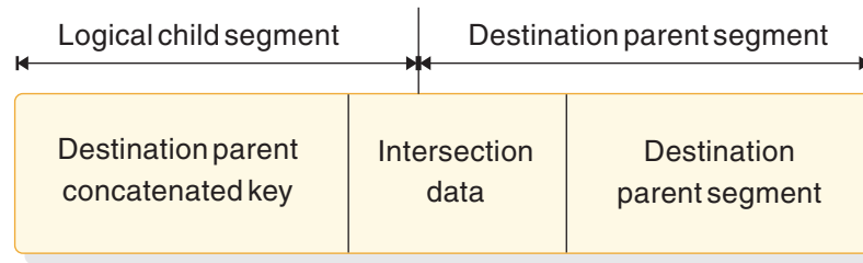
Figure 83. Format of a concatenated segment returned to user I/O area
