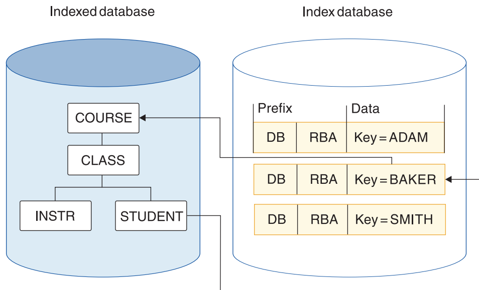
Figure 171. How a segment is accessed using a secondary index
