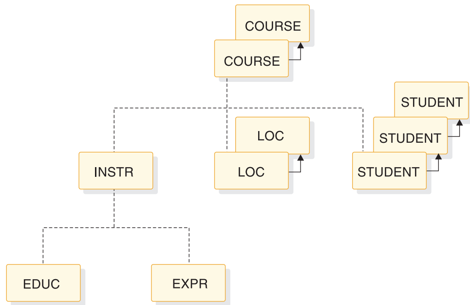
Figure 39. Physical twin forward pointers
