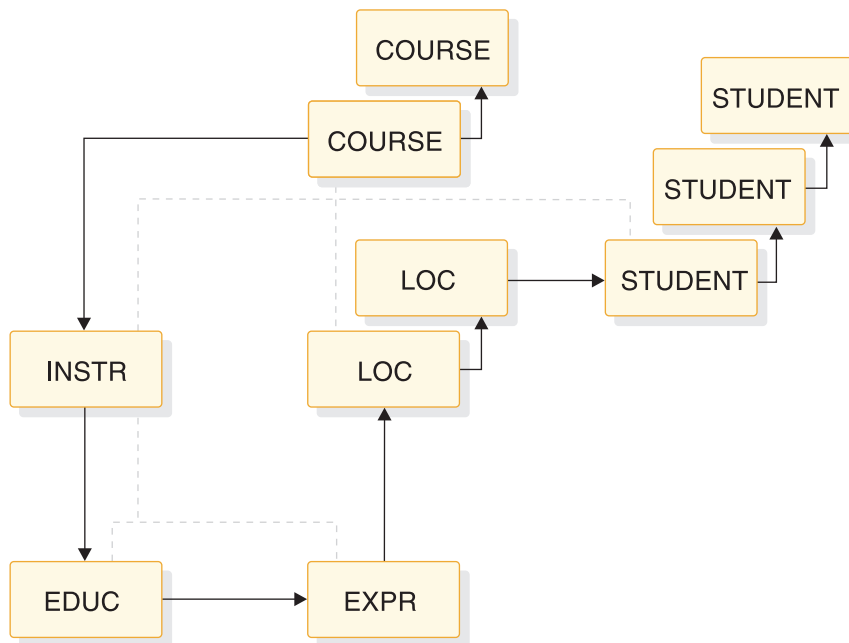
Figure 34. Hierarchical forward pointers
