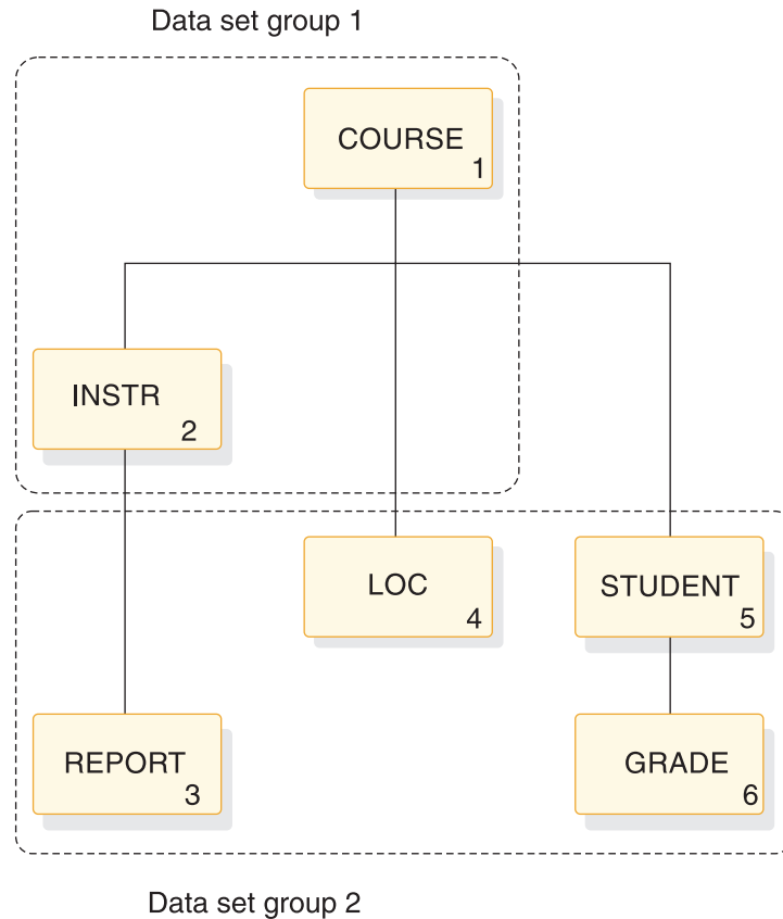
Figure 205. First example of data set groups
