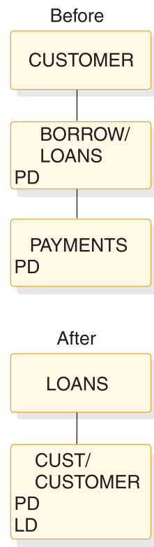
Figure 141. Logical child, virtual pairing—logical delete rule example: before and after
