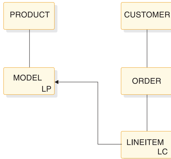
Figure 164. Example of a unidirectional logical relationship
