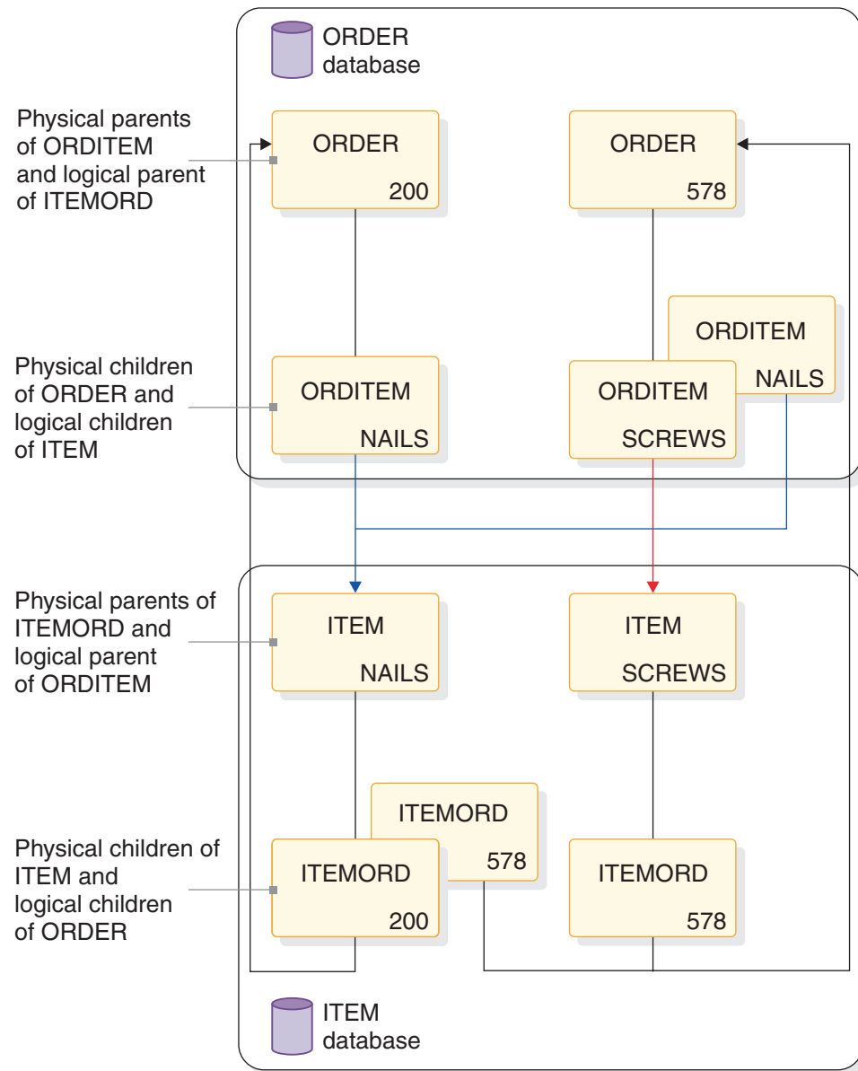
Figure 72. Two unidirectional logical relationships
