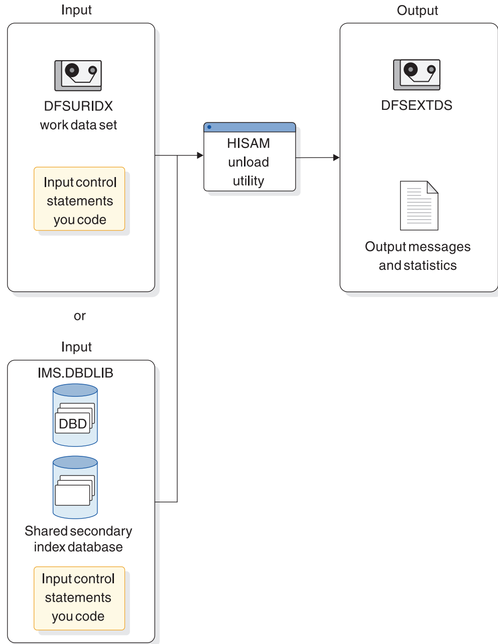
Figure 256. HISAM Reorganization Unload utility used for extract secondary indexing operations
