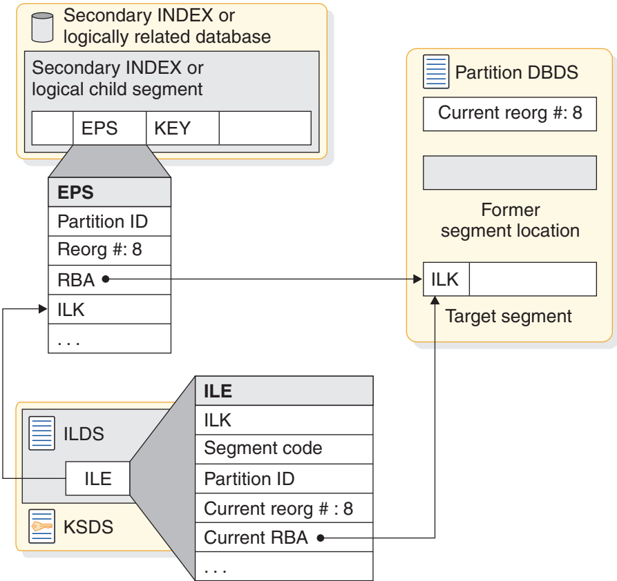
Figure 266. HALDB pointer after the self-healing process
