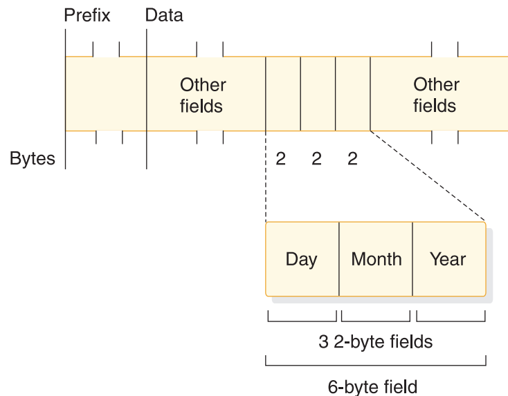
Figure 229. Example of a date field within a segment defined as three 2-byte fields and one 6-byte field
