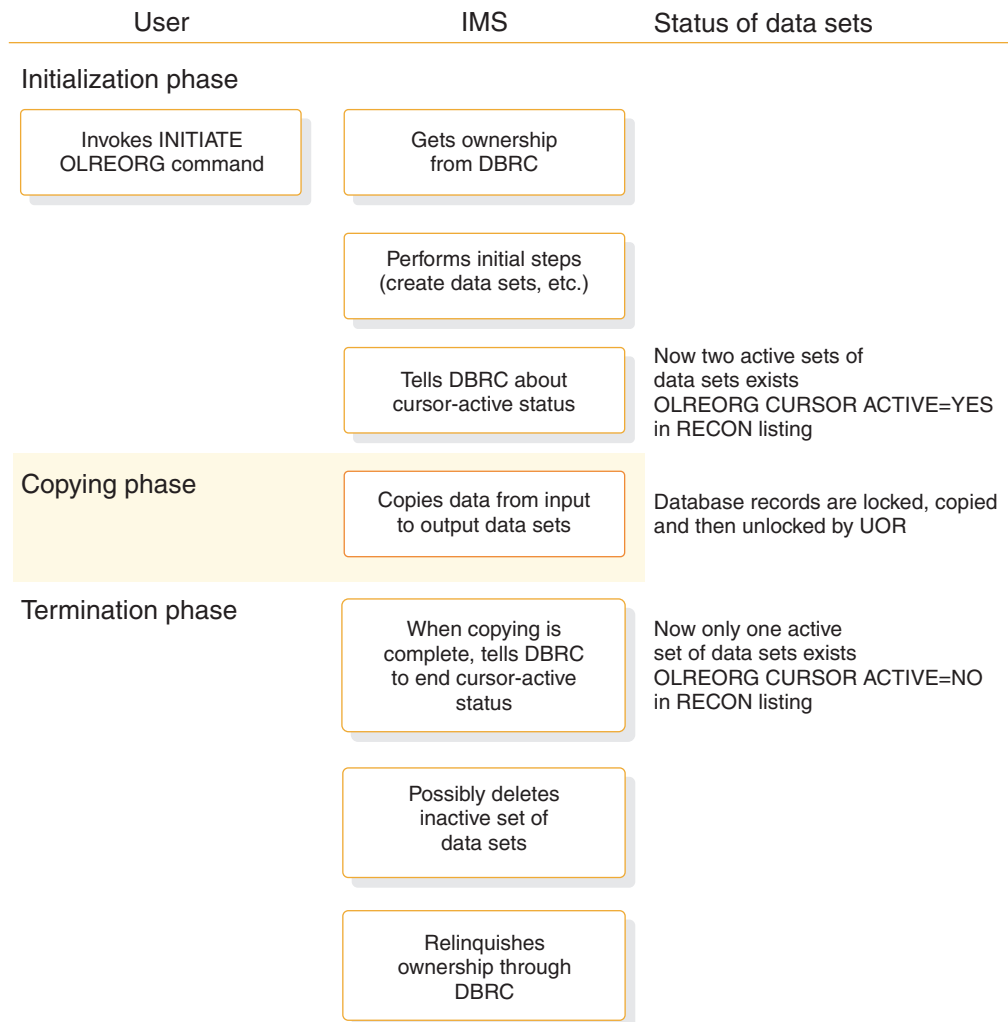
Figure 261. Normal processing steps of HALDB Online Reorganization
