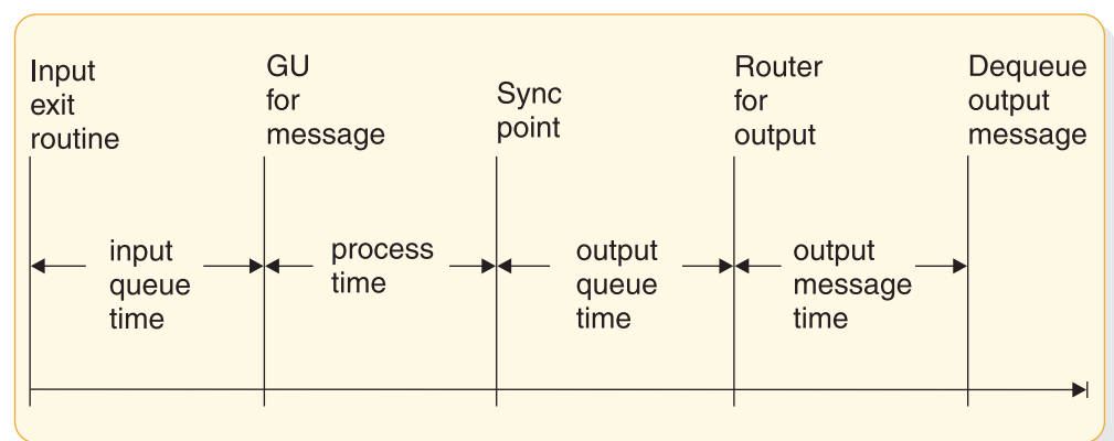
Figure 244. Fast Path transaction event timings
