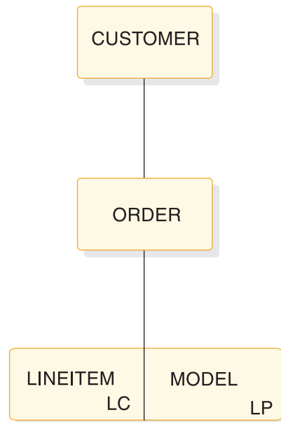
Figure 165. Example of a logical structure
