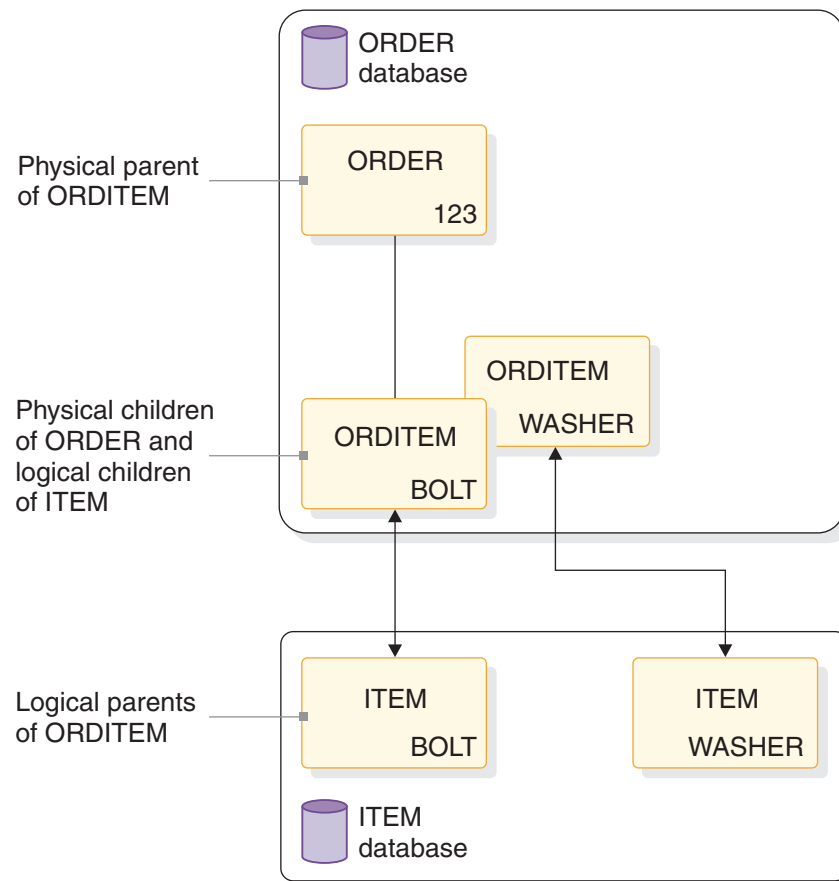
Figure 74. Bidirectionally virtually paired logical relationship
