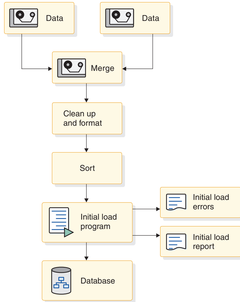
Figure 237. Loading a database using existing files
