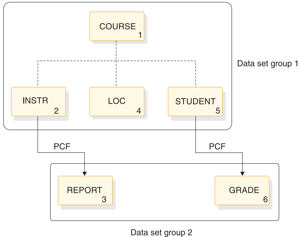
Figure 203. Connecting segments in multiple data set groups using physical child first pointers
