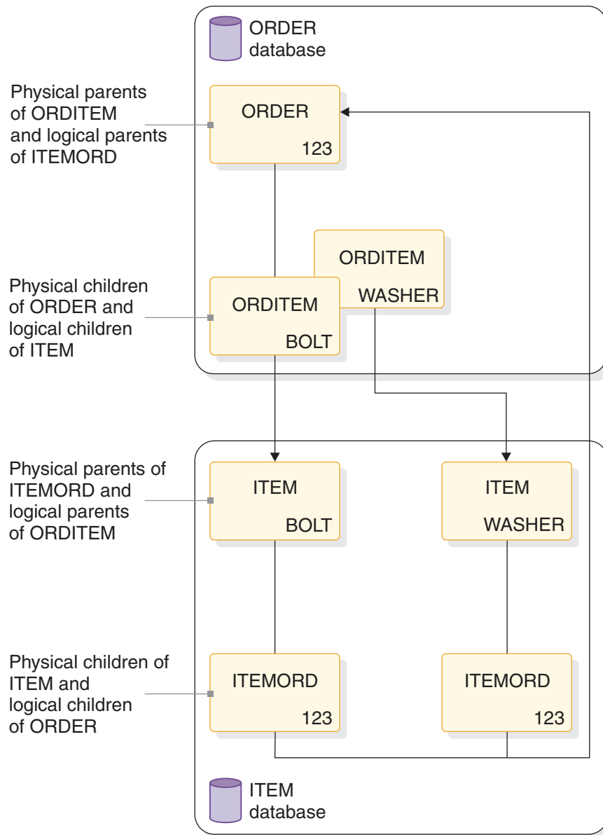
Figure 73. Bidirectional physically paired logical relationship
