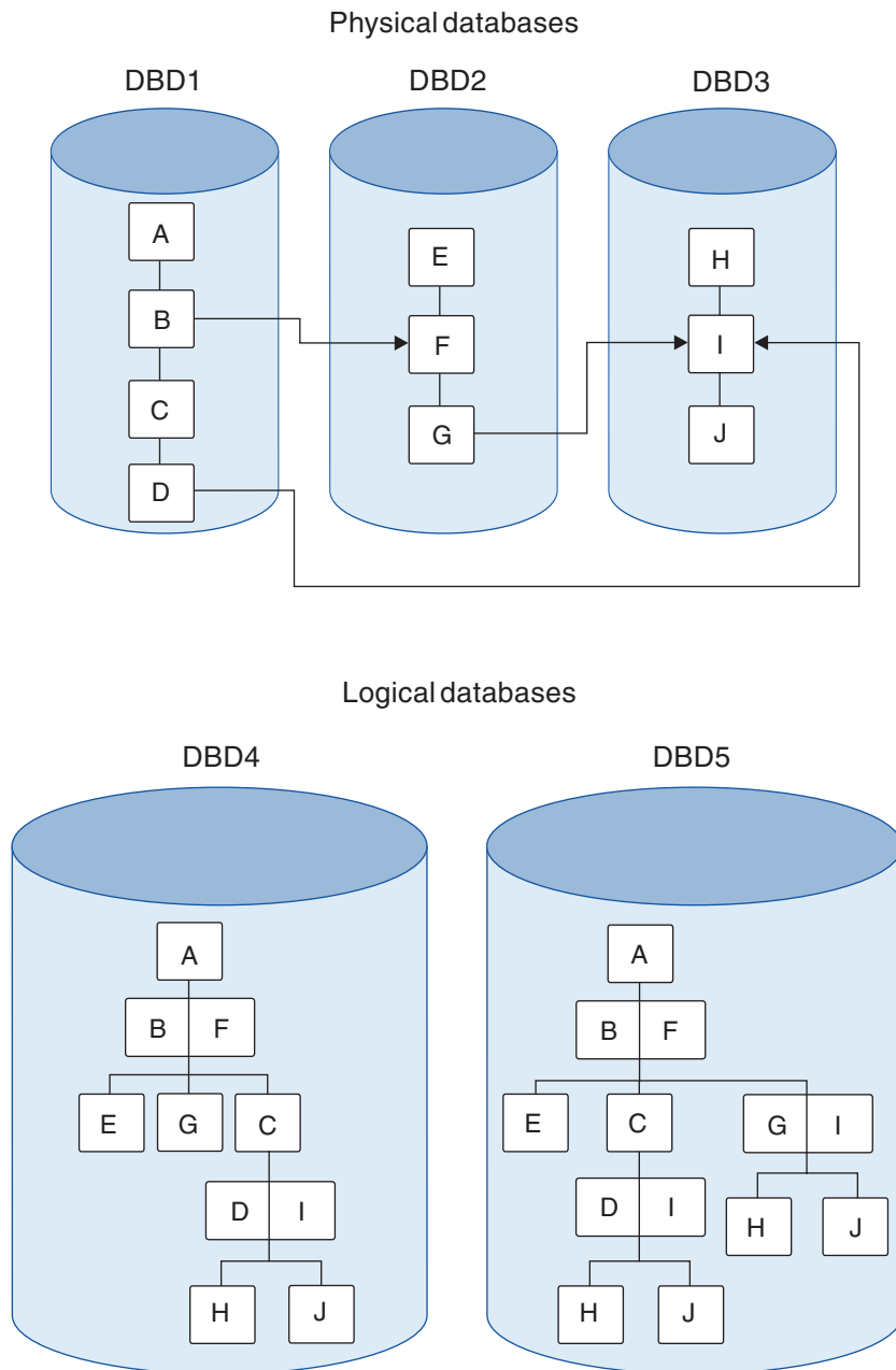
Figure 94. The first logical relationship crossed in a hierarchical path of a logical database
