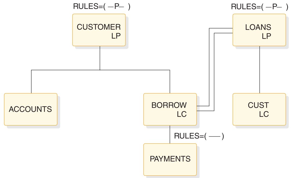
Figure 118. Logical parent, physical pairing—physical delete rule example
