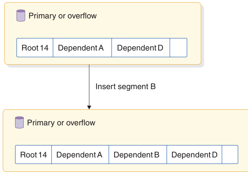
Figure 26. Inserting a dependent segment into a HISAM database (space exists in the logical record)
