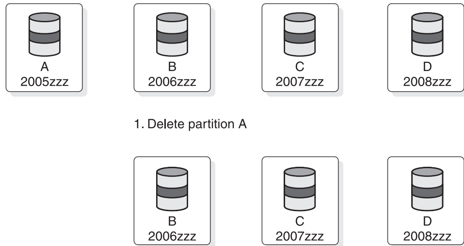
Figure 294. Deleting the partition with the lowest key in a HALDB that uses key range partitioning
