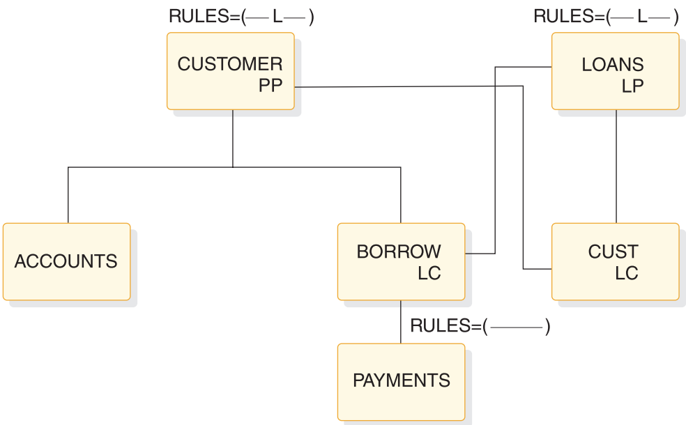
Figure 124. Logical parent, physical pairing—logical delete rule example
