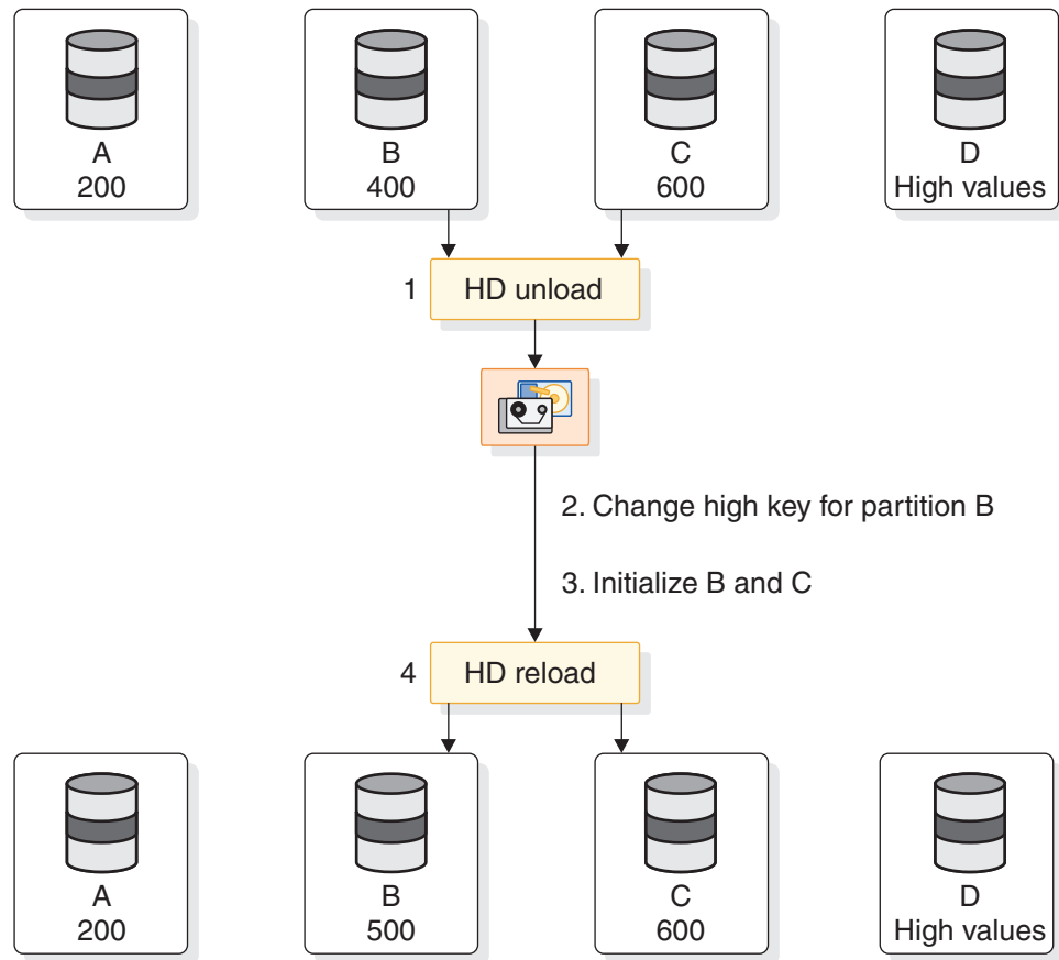
Figure 287. Changing a high key with key range partitioning
