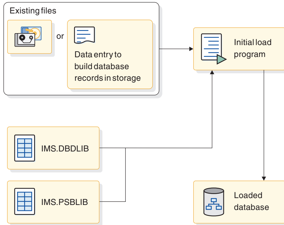
Figure 236. The load process
