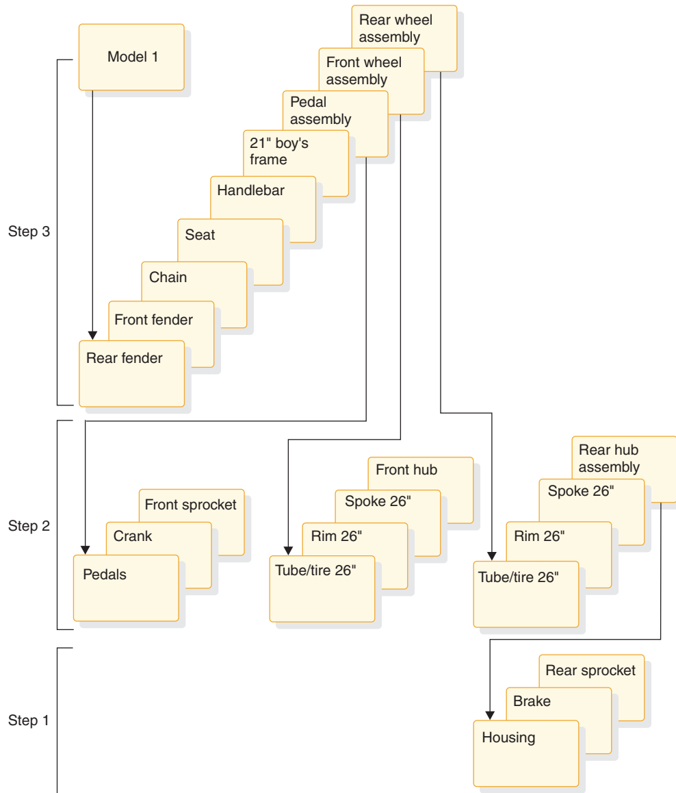
Figure 86. Model 1 components and subassemblies
