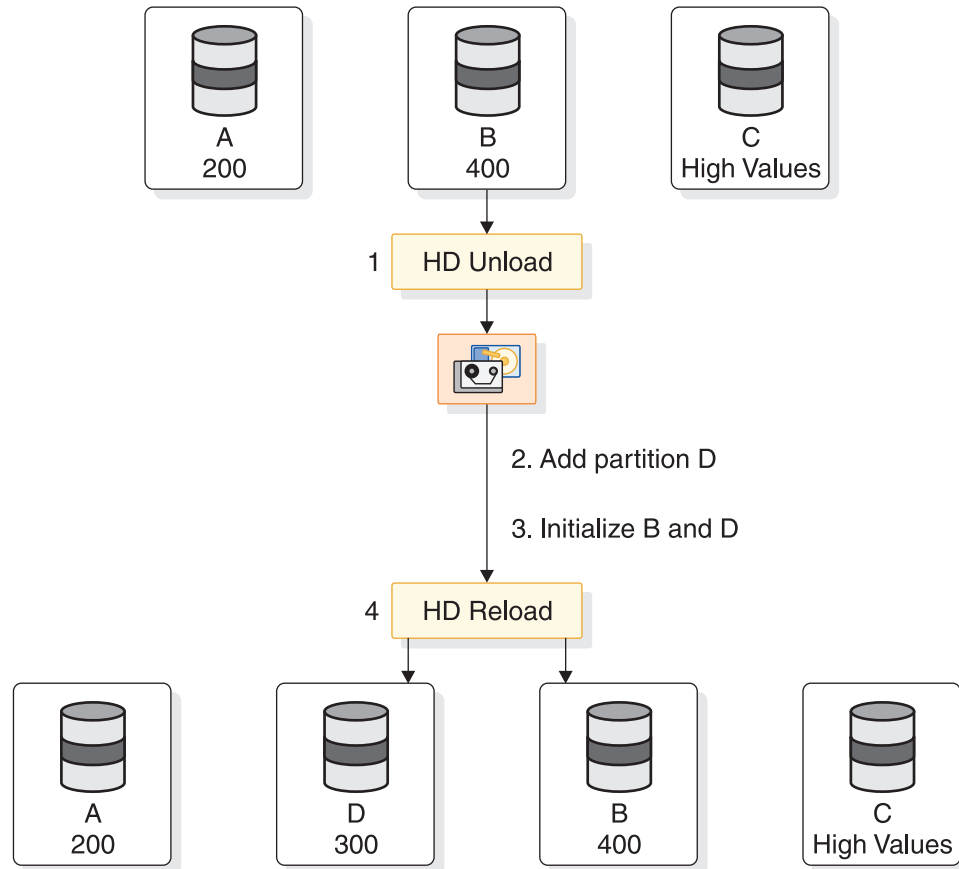
Figure 291. Adding a partition with key range partitioning
