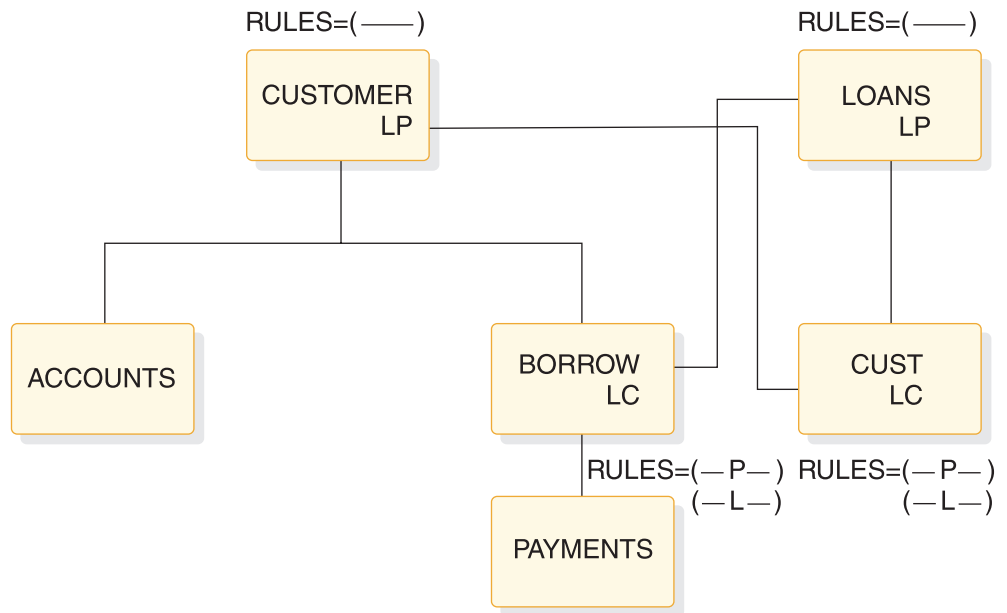
Figure 142. Logical child, physical pairing—physical or logical delete rule example
