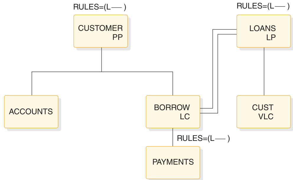
Figure 103. Logical insert rule example
