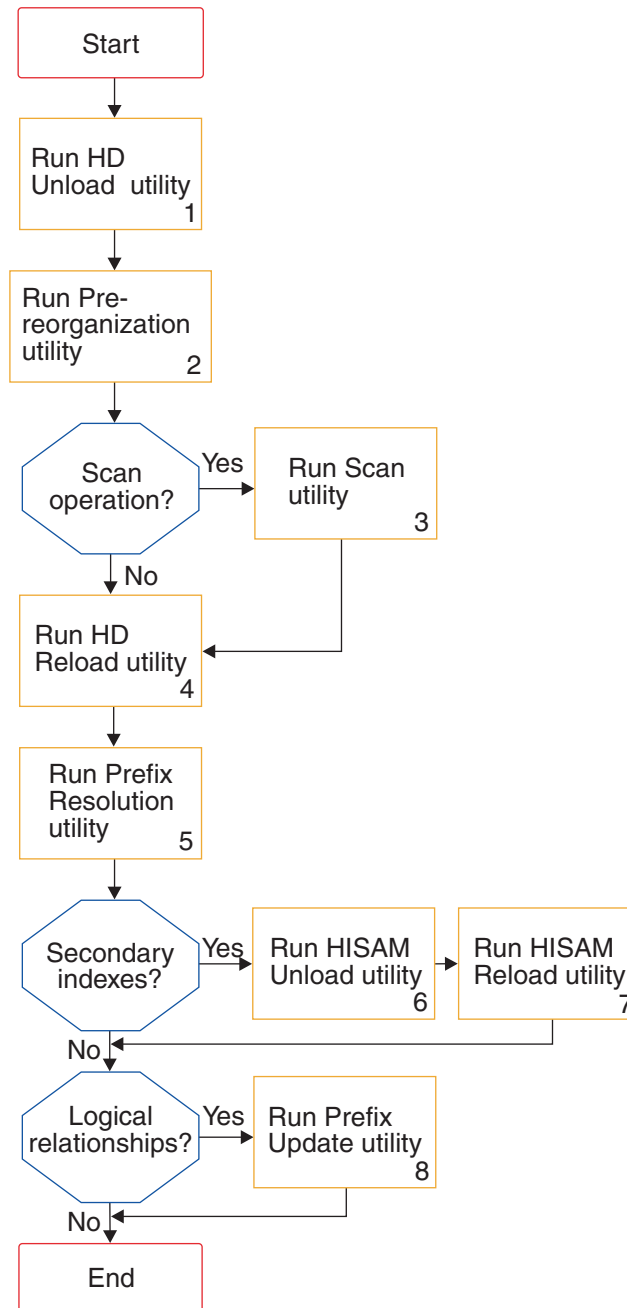
Figure 245. Steps in reorganizing when logical relationships or secondary indexes exist
