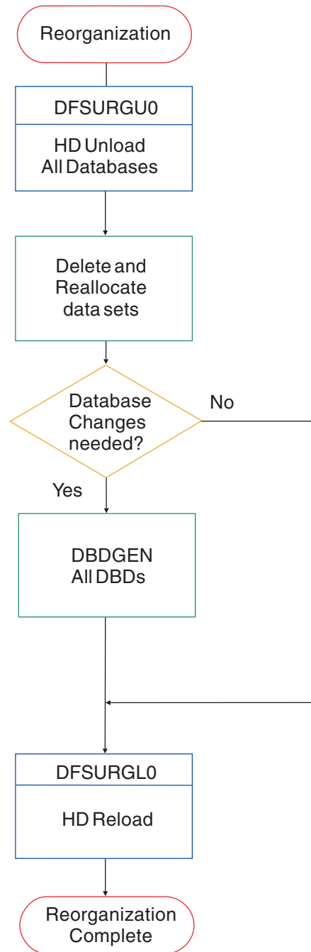
Figure 283. Flow chart of process for modifying a database to use multiple data set groups
