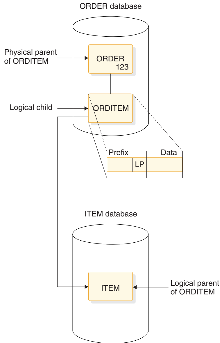
Figure 75. Direct logical parent (LP) pointer
