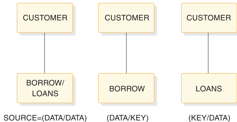
Figure 161. Concatenated segment relationships
