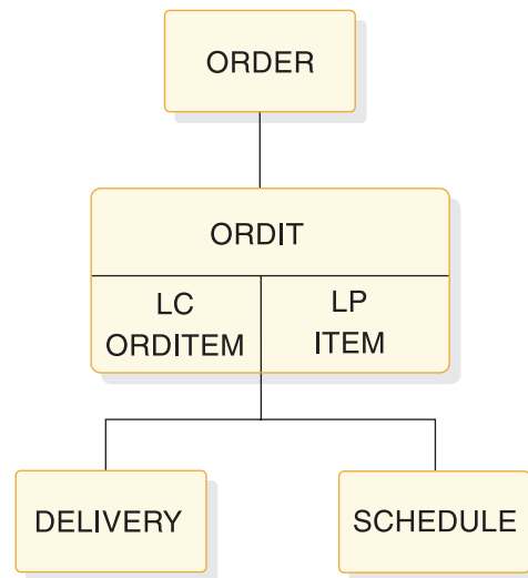
Figure 92. Logical data structure for a unidirectional relationship using symbolic pointing
