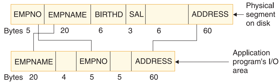
Figure 190. DBD and PSB coding for field-level sensitivity
