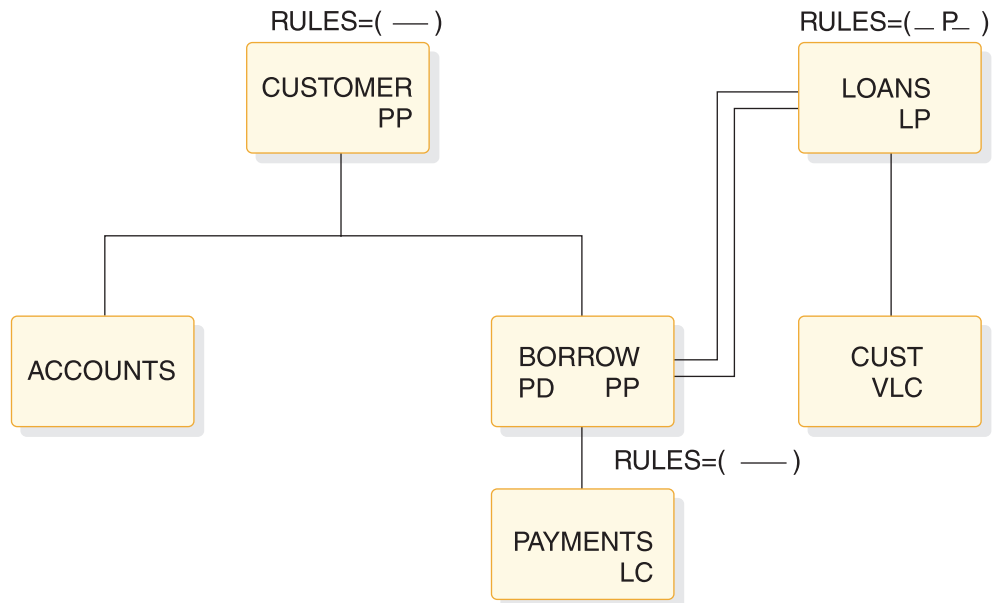
Figure 115. Logical parent, virtual pairing—physical delete rule example
