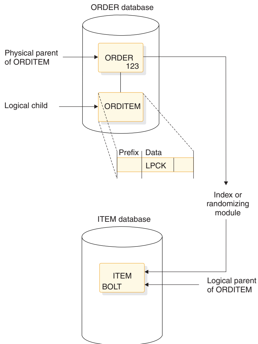
Figure 76. Symbolic logical parent (LP) pointer
