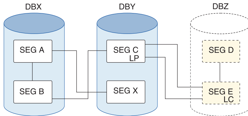
Figure 275. DBX and DBY exist, DBZ is to be added
