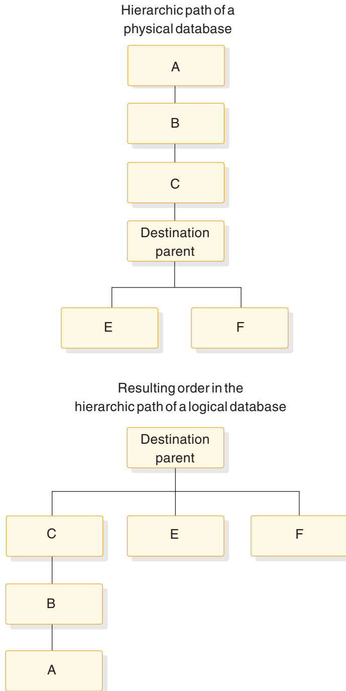
Figure 95. Logical database hierarchy enabled by crossing the first logical relationship
