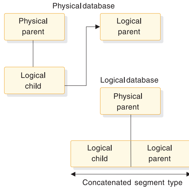
Figure 81. Defining a physical parent to logical parent path in a logical database
