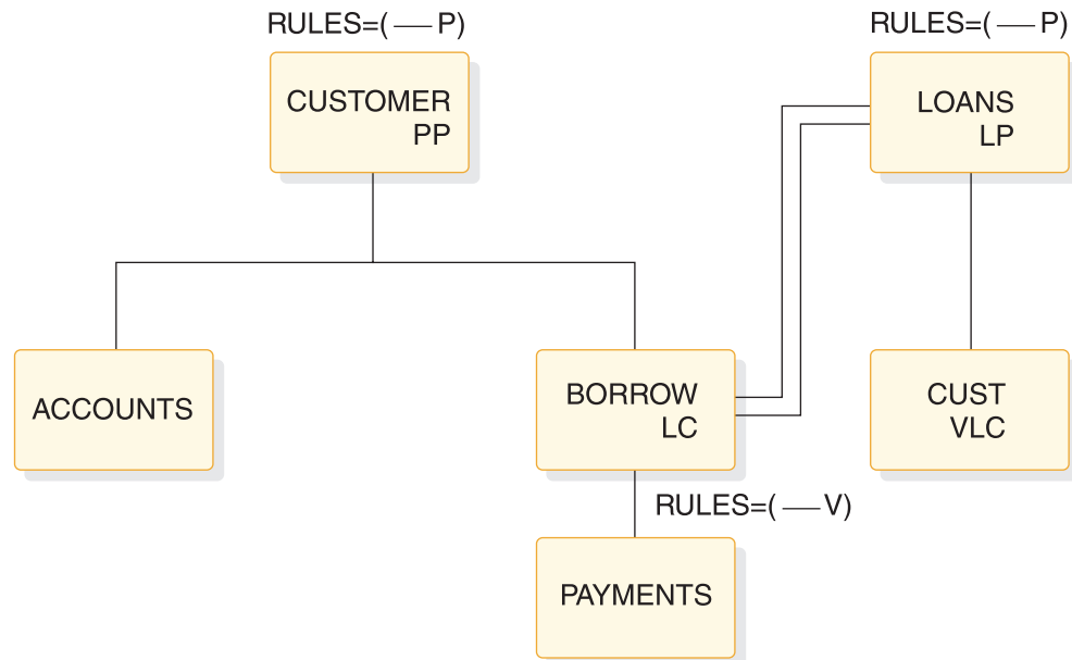
Figure 109. Physical replace rule example
