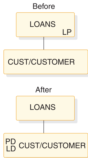
Figure 116. Logical parent, physical pairing—physical delete rule example: before and after
