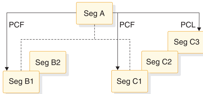
Figure 38. Specifying PCF and PCL pointers
