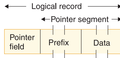
Figure 175. Example of a logical record containing a pointer segment
