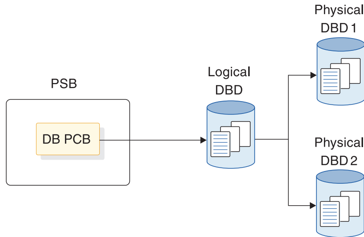
Figure 89. Relationship of control blocks when a logical relationship is used
