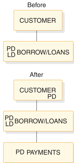
Figure 119. Logical Parent, physical pairing—physical delete rule example: before and after
