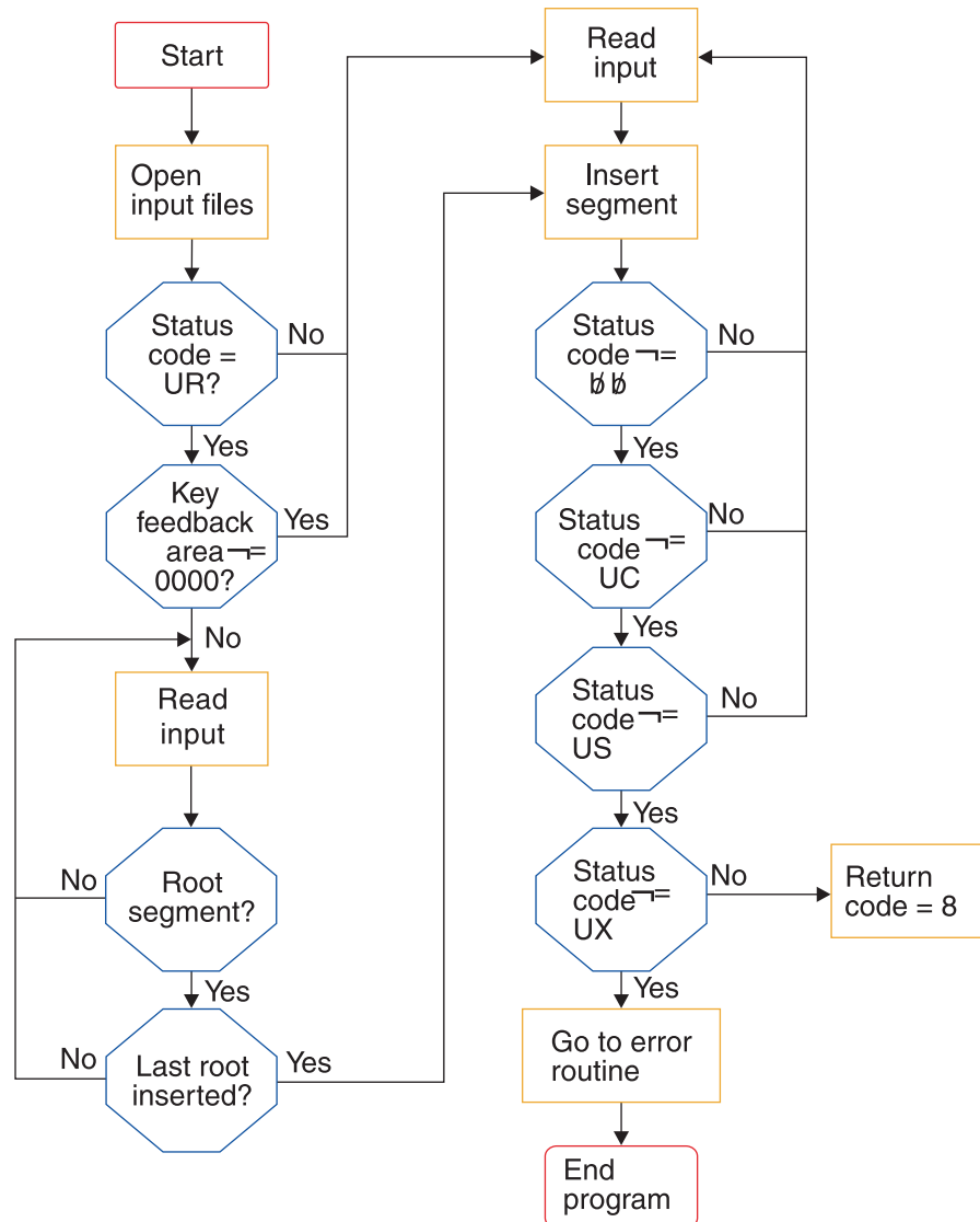
Figure 239. Restartable initial load program logic
