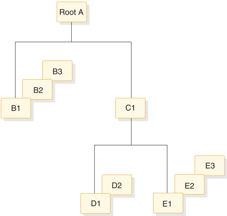
Figure 224. Database record for logical records example
