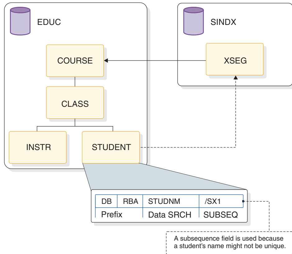
Figure 186. Databases for secondary indexing example
