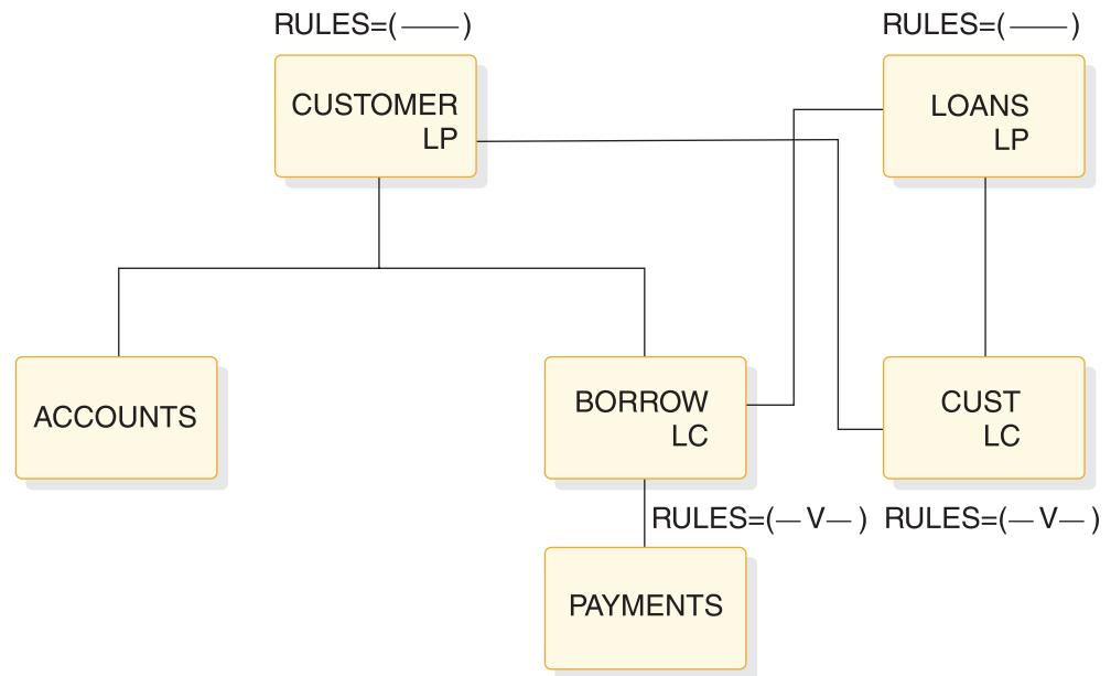
Figure 148. Logical child, physical pairing—virtual delete rule example
