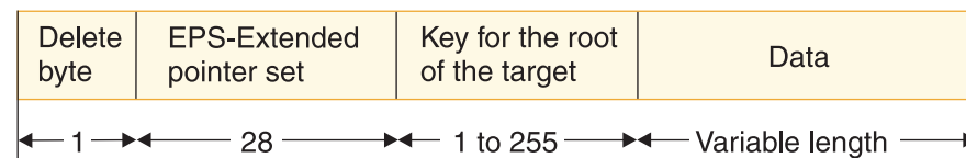
Figure 176. Secondary index entry for HALDB
