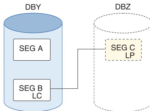
Figure 276. DBY exists, DBZ is to be added
