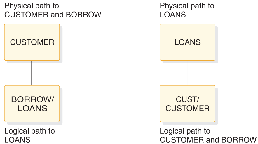
Figure 101. Paths for physical insert rule example
