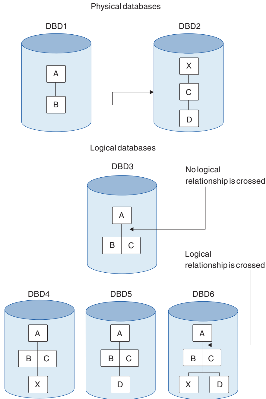
Figure 93. Definition of crossing a logical relationship
