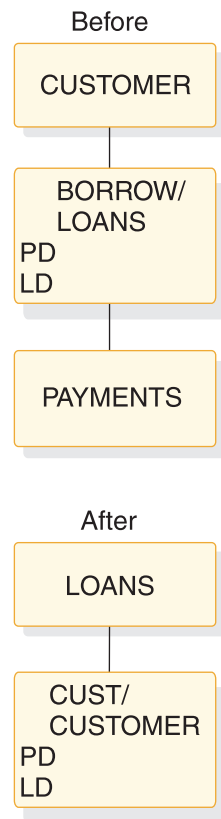
Figure 147. Logical child, virtual pairing—virtual delete rule example: before and after
