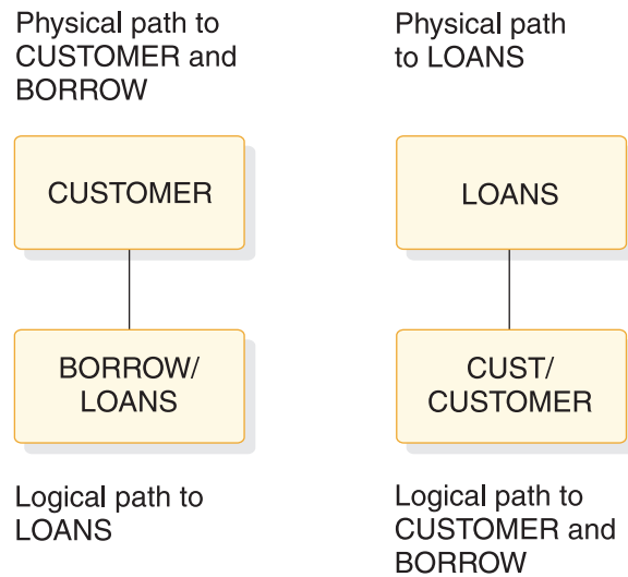
Figure 98. Example of the replace, insert, and delete rules: before and after
