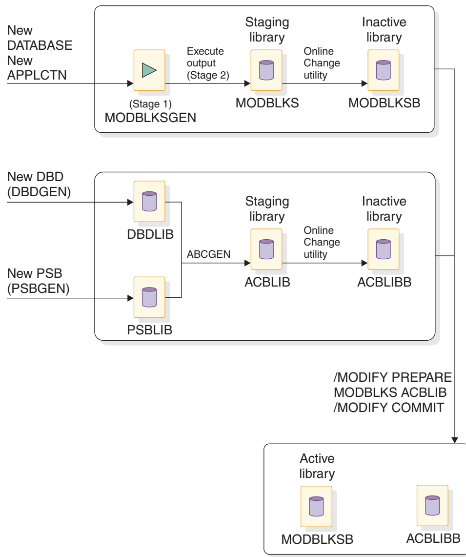
Figure 286. Adding a database using online change
