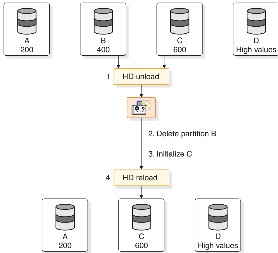
Figure 293. Deleting a partition with key range partitioning
