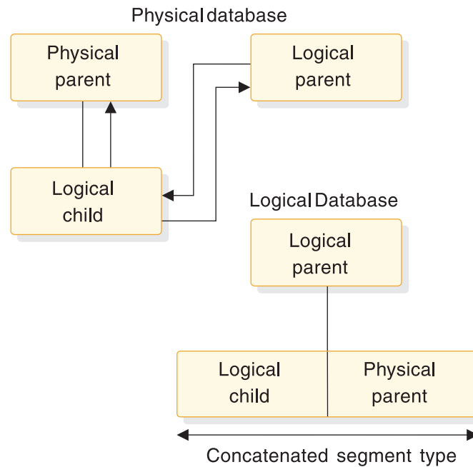
Figure 82. Defining a logical parent to physical parent path in a logical database
