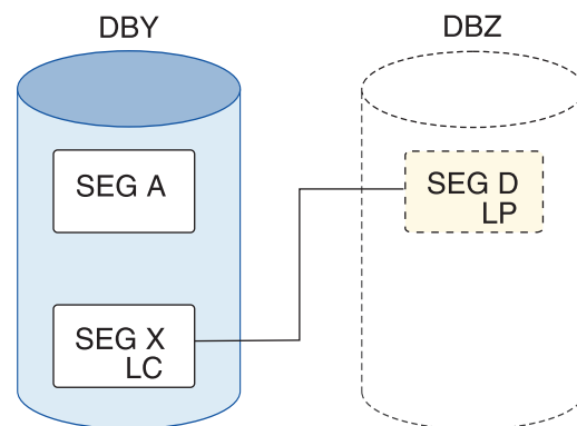
Figure 277. DBY exists, DBZ is to be added
