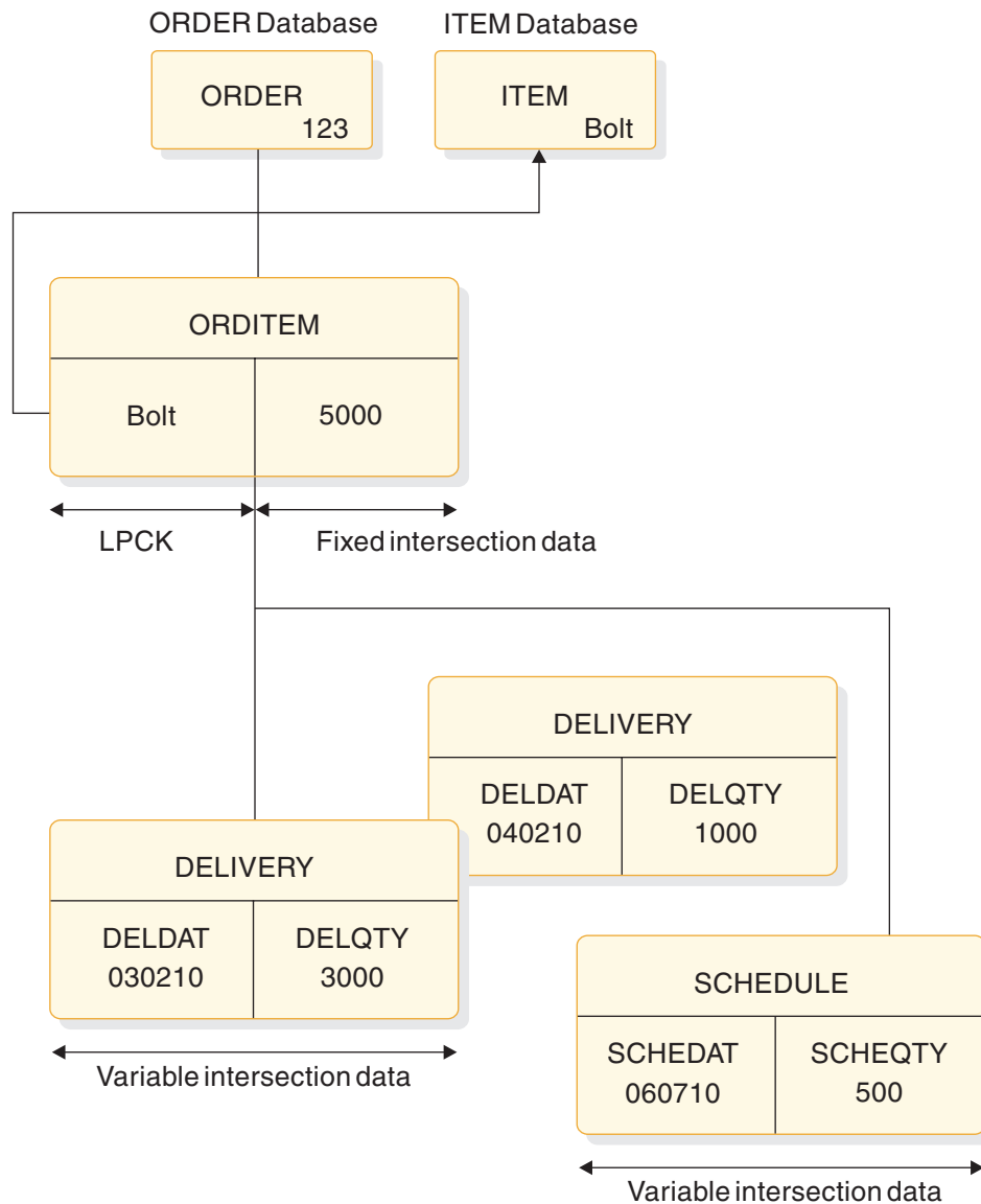
Figure 85. Variable intersection data
