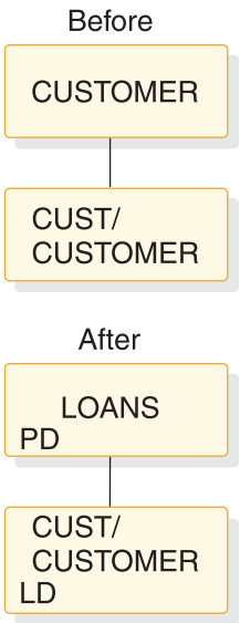
Figure 122. Logical parent, virtual pairing—logical delete rule example: before and after
