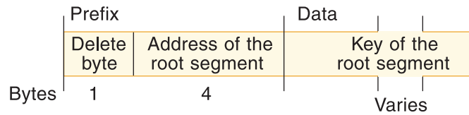
Figure 50. Format of an index segment
