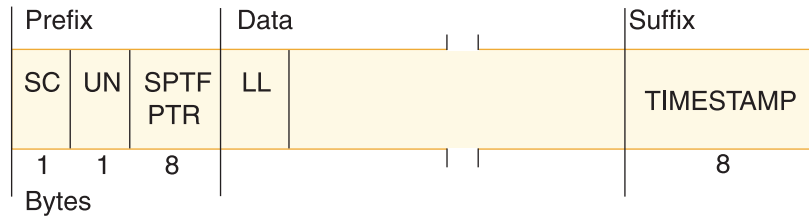
Figure 59. Sequential dependent segment format
