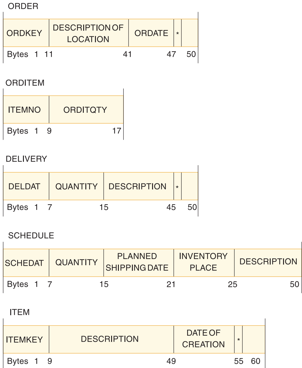
Figure 90. Layouts of segments used in the examples
