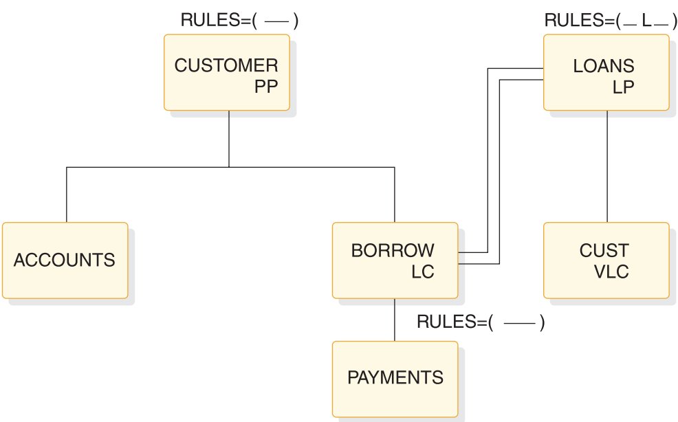
Figure 121. Logical parent, virtual pairing—logical delete rule example
