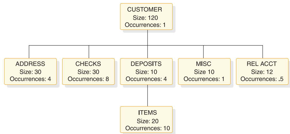
Figure 235. Segment sizes and average segment occurrences
