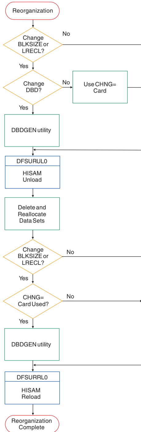
Figure 284. Flow chart of process for modifying a HISAM database to use multiple data set groups
