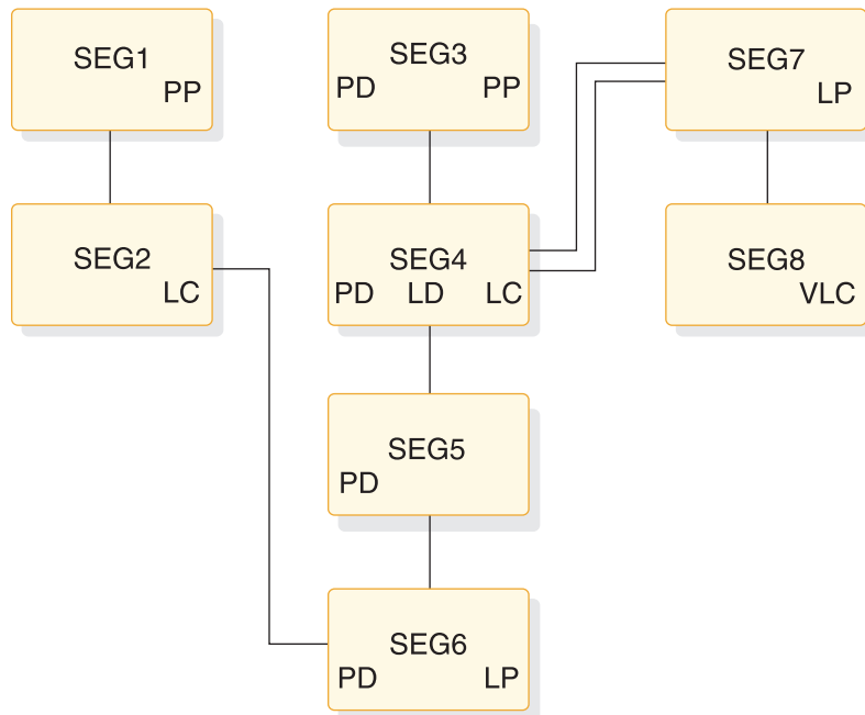
Figure 152. (Part 2 of 5). Example of deleted segments accessibility
