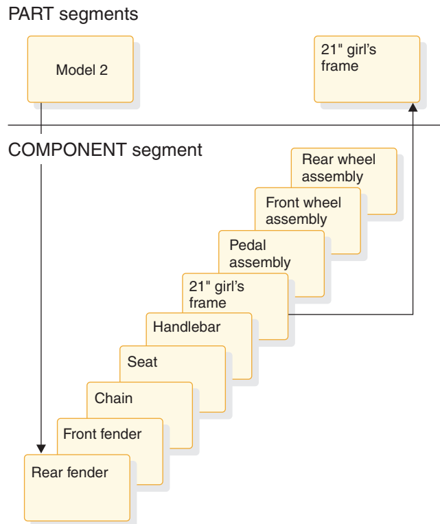
Figure 88. Extra database records required for the Model 2 bicycle
