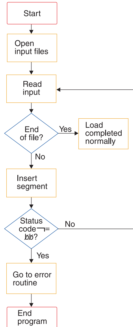
Figure 238. Basic initial load program logic
