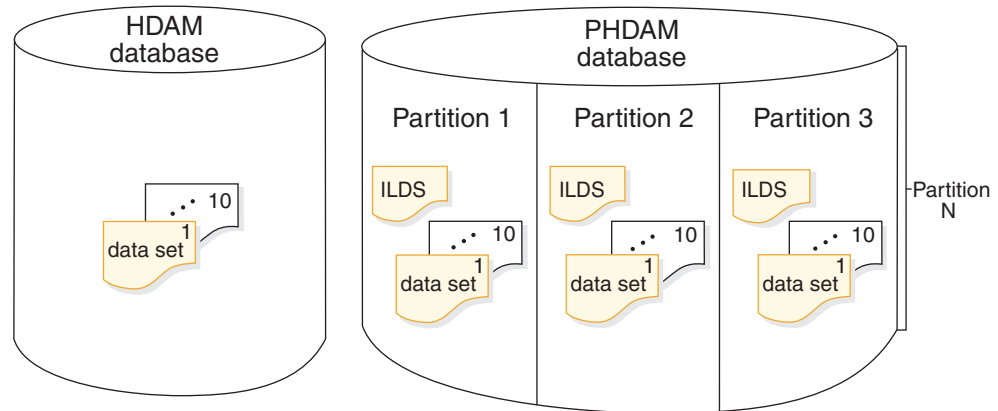
Figure 30. A comparison of the logical views of HDAM and PHDAM databases
