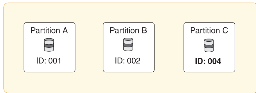
Figure 290. Partition IDs after deleting and redefining a partition
