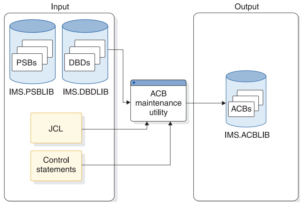
Figure 232. The ACB generation process
