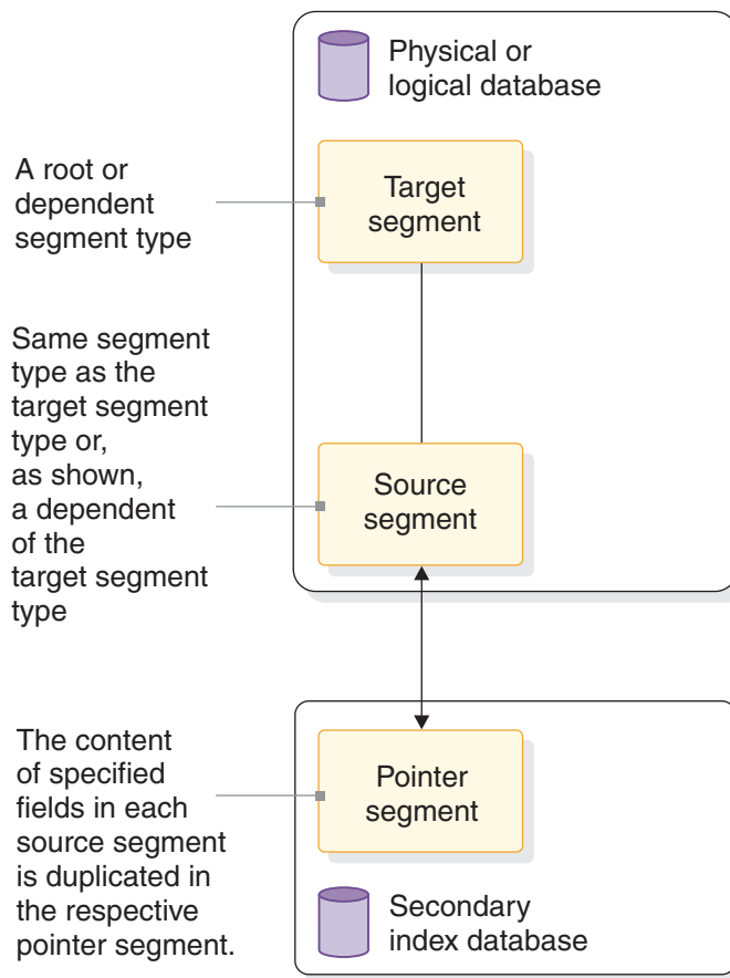
Figure 168. Segments used for secondary indexes
