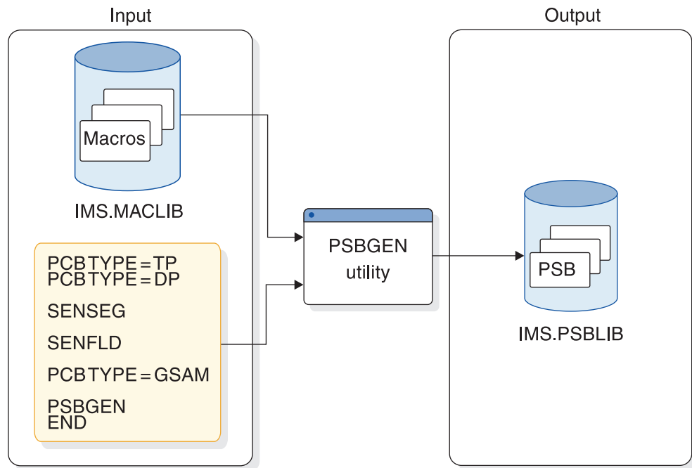
Figure 230. The PSB generation process
