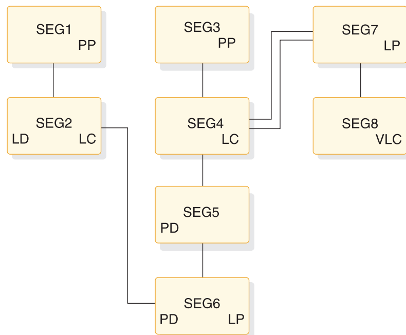
Figure 155. (Part 5 of 5). Example of deleted segments accessibility
