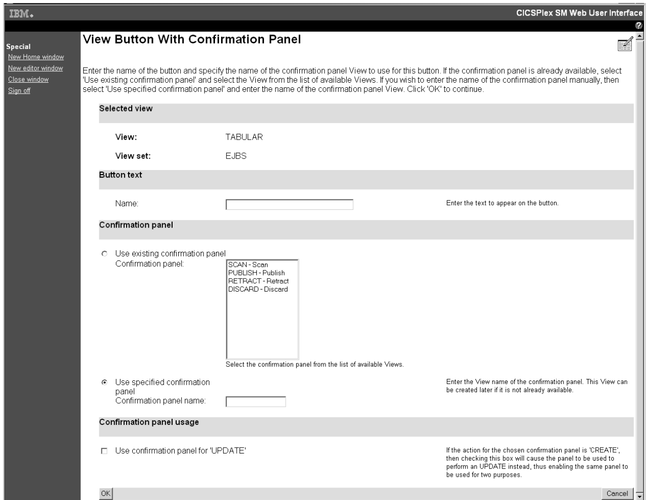
Figure 41. View Button With Confirmation screen
