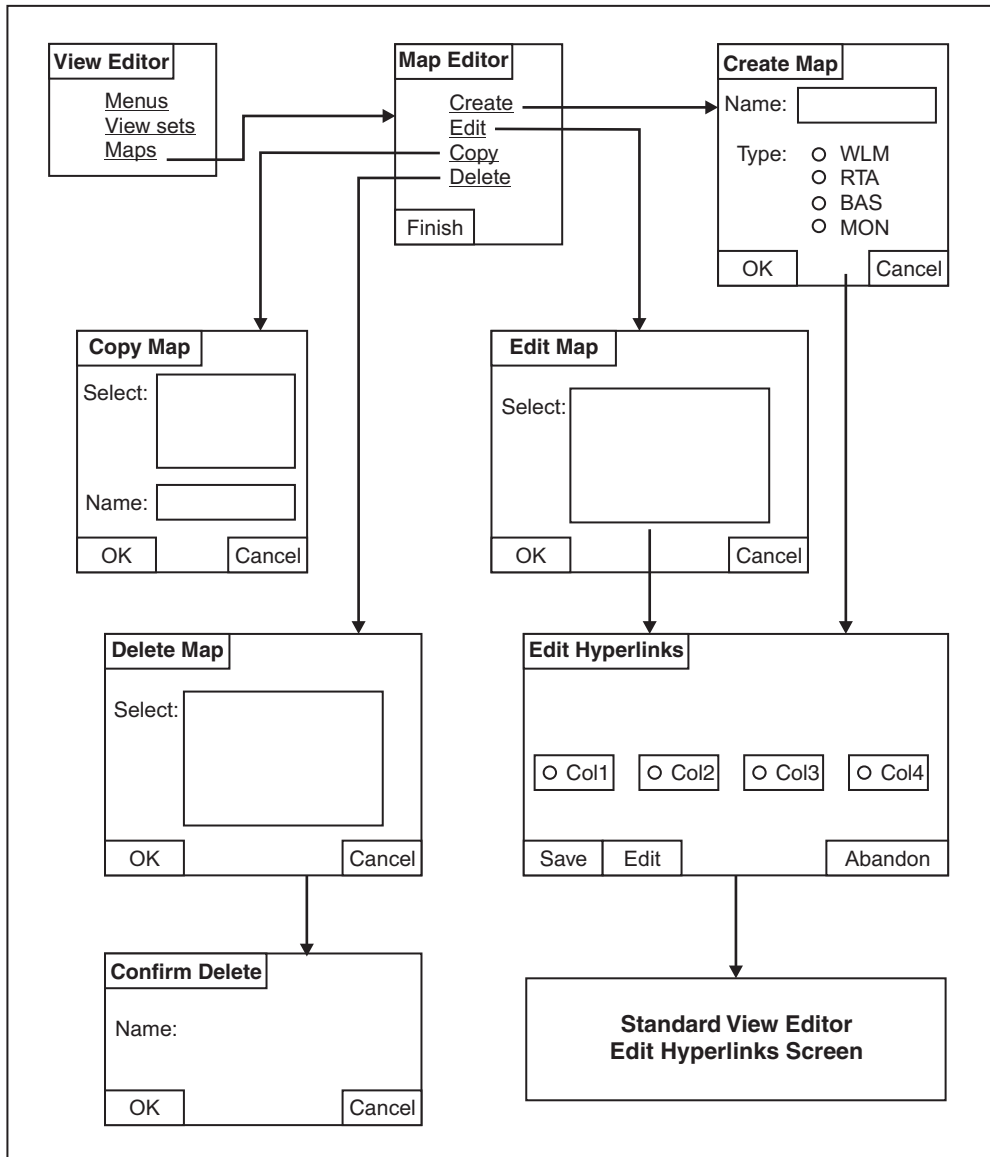
Figure 42. Map editing panels in the View Editor
