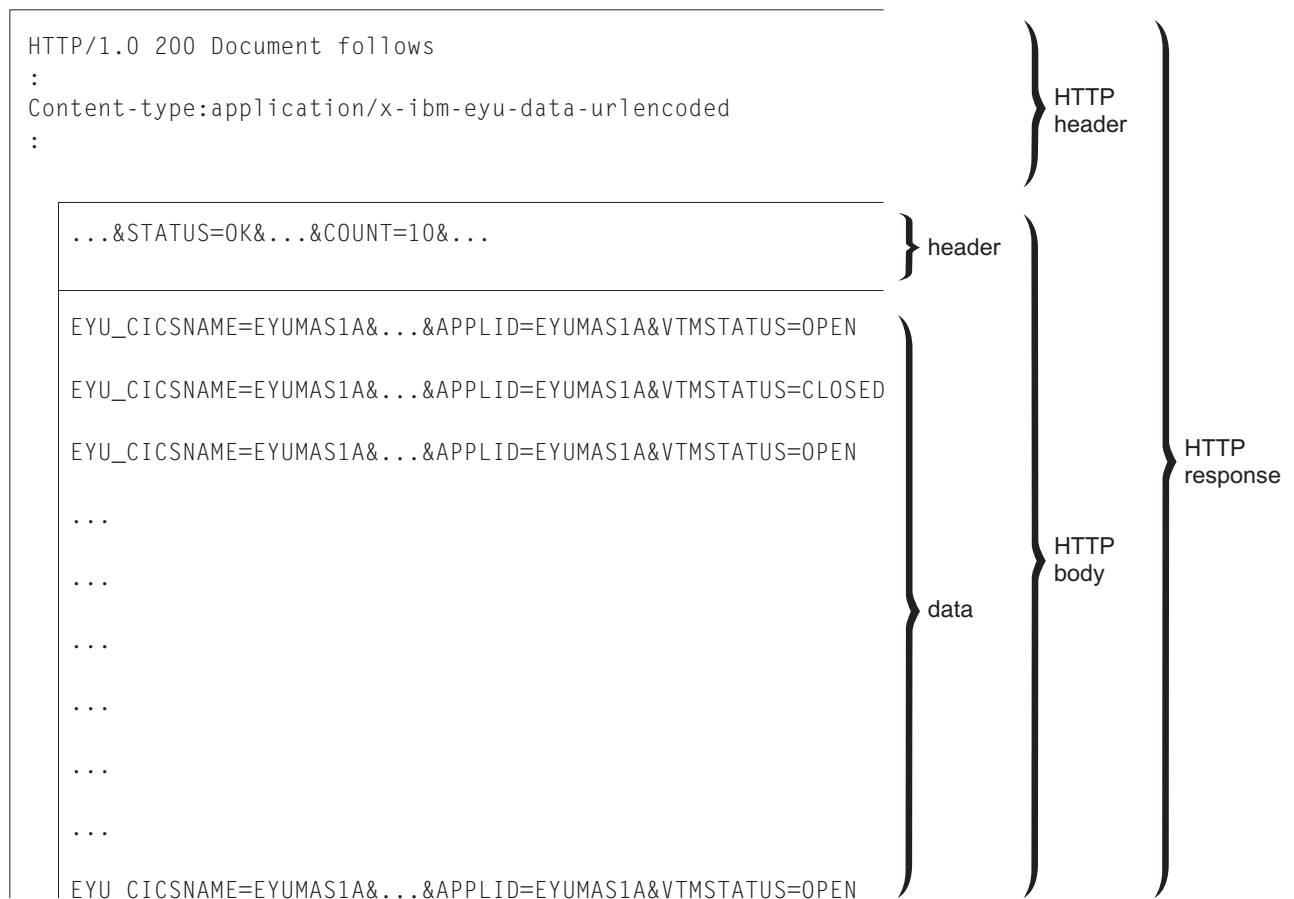
Figure 50. Structure of an HTTP response to a data interface request
