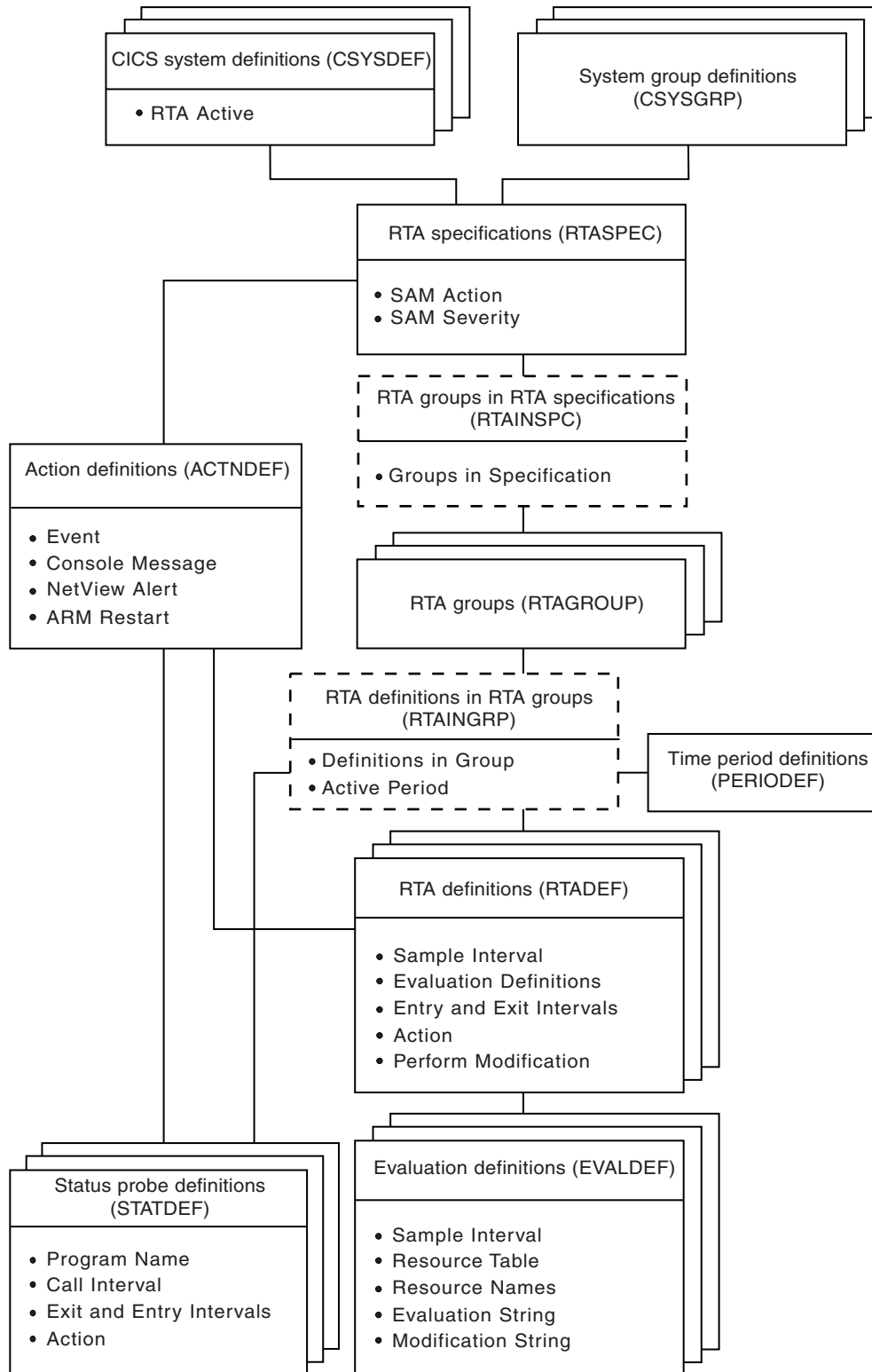
Figure 19. The real-time analysis object model
