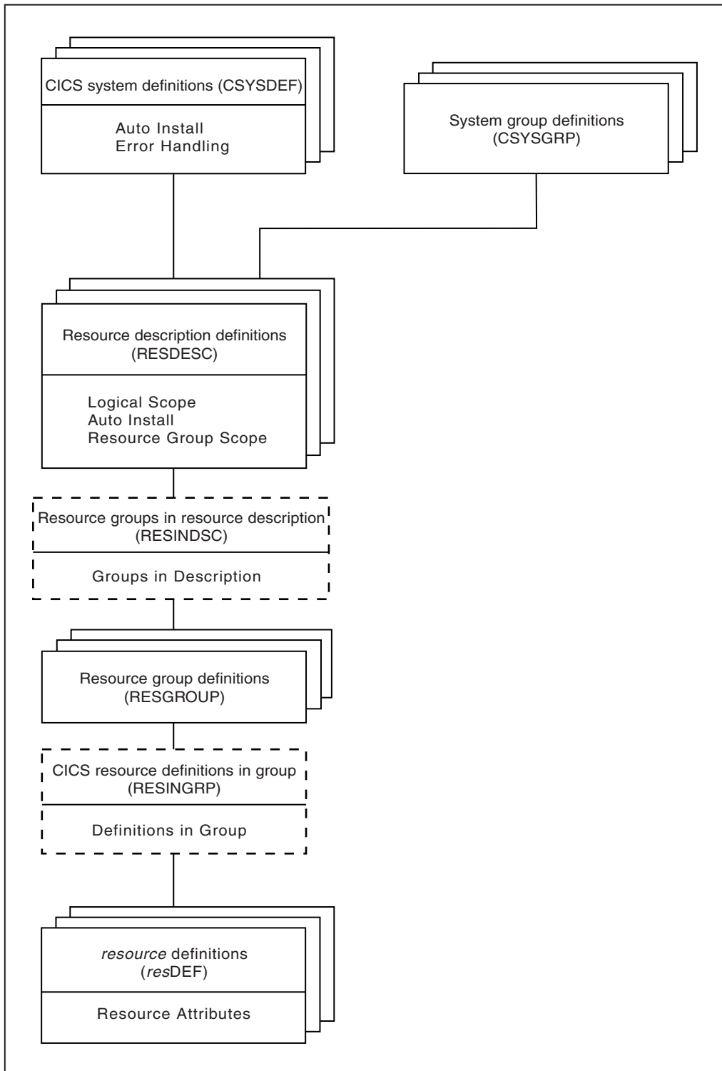
Figure 14. The migration from BAS object model
