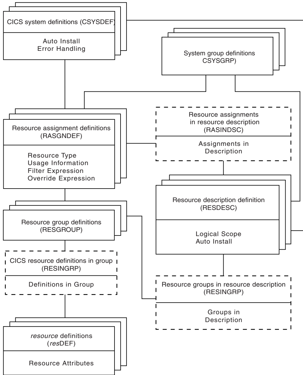
Figure 15. The full-function BAS object model
