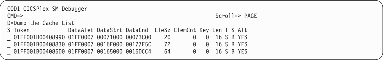
Figure 24. An example LIST CLIST display
