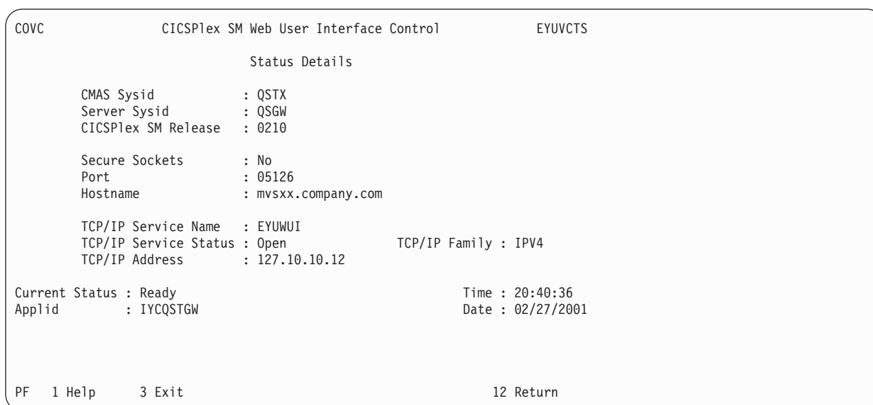
Figure 38. COVC status panel
