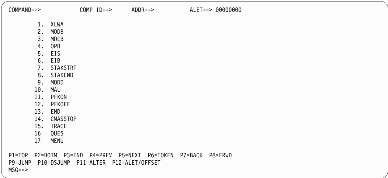
Figure 34. CODB debugging transaction menu
