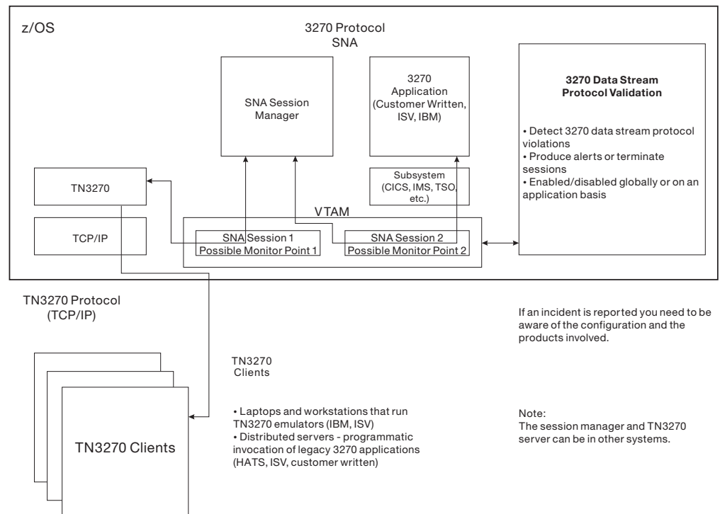
Figure 108. Sample of typical SNA 3270 network configuration
