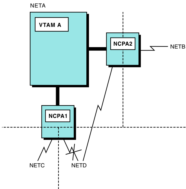
NCPA1 link to NETD goes down. NETD dials NCPA2 to connect to NETA. Figure 146. Backup of a gateway NCP - part 2
