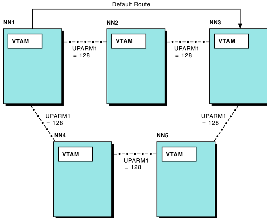
Figure 180. Sample network using default for UPARM1
