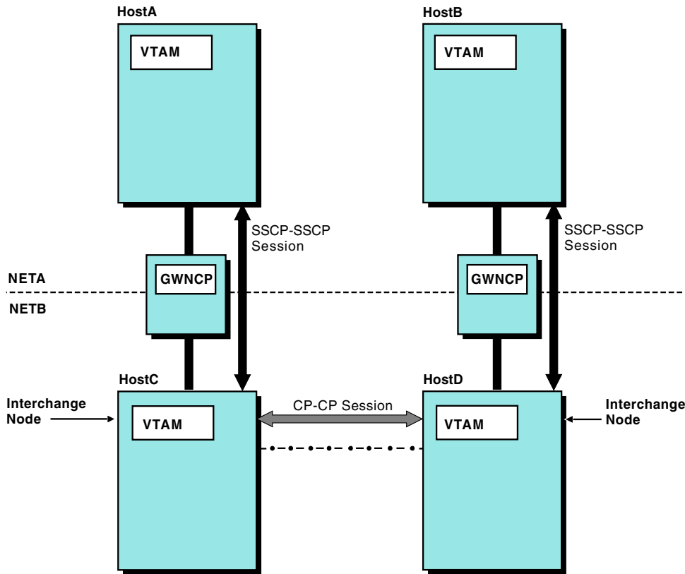
Figure 137. Disjoint hosts
