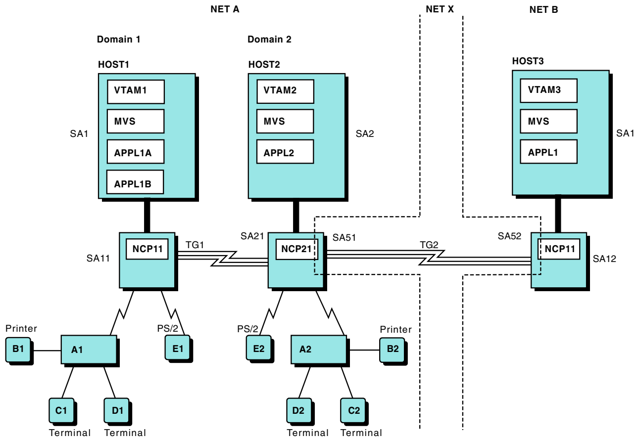
Figure 144. Multiple-network environment
