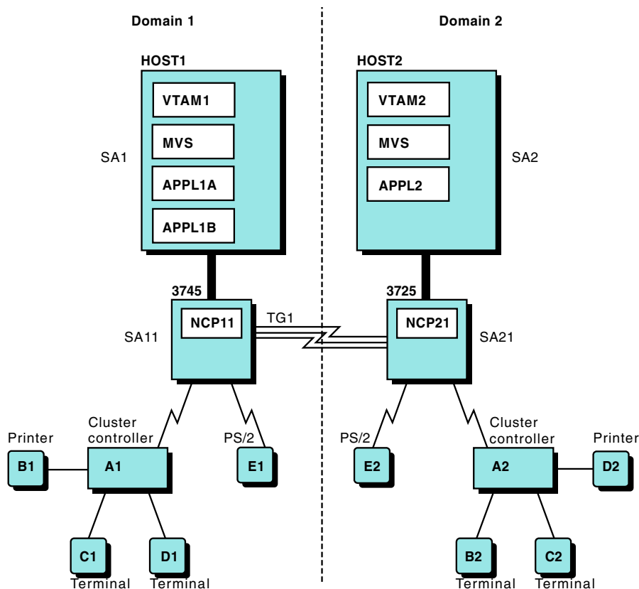
Figure 141. Multiple-domain network
