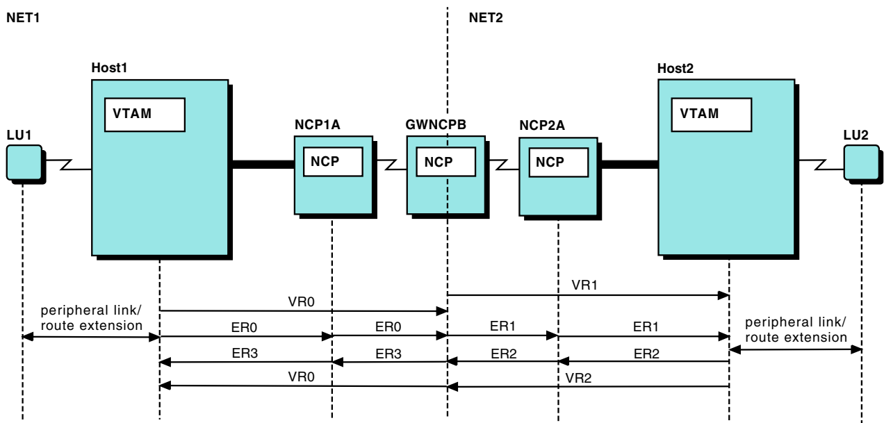
Figure 151. Multiple-network paths
