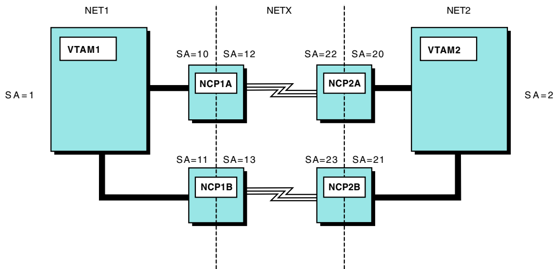
Figure 147. Multiple-network configuration: CDRM major nodes
