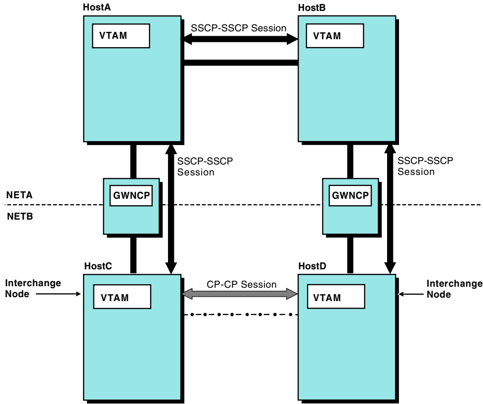
Figure 138. Hosts with subarea connection
