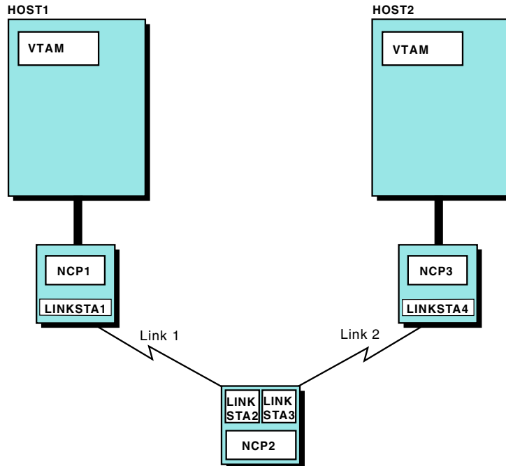
Figure 158. Effects of NCP deactivation on cross-subarea links and link stations
