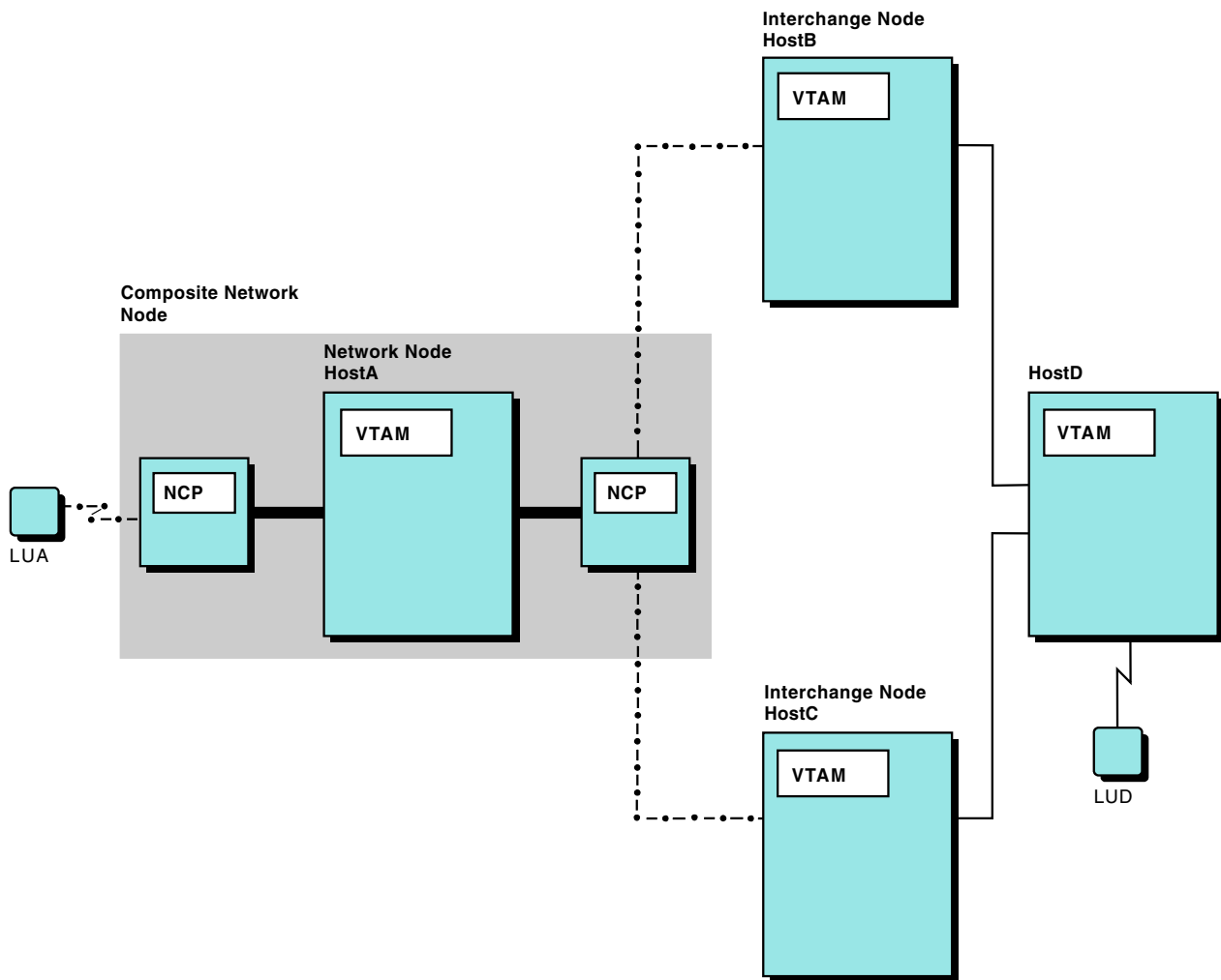
Figure 140. Class of Service resolution at multiple nodes
