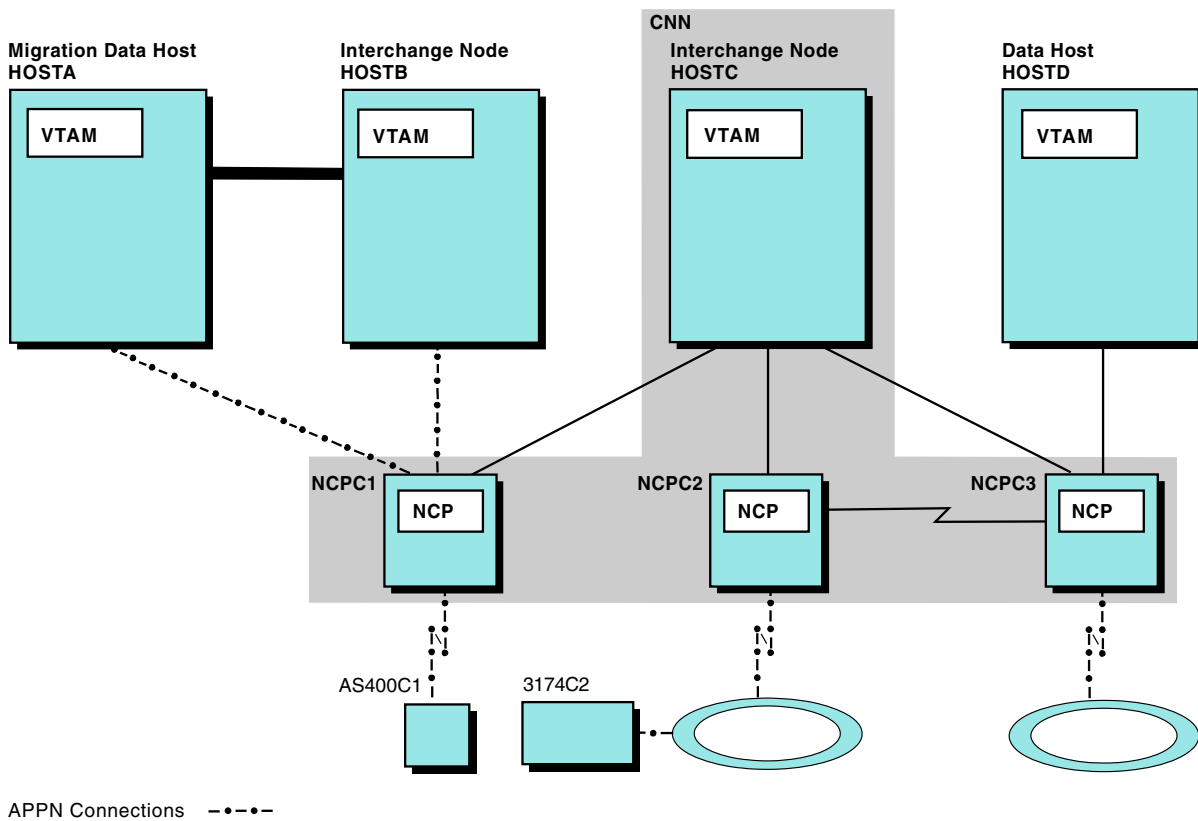
Figure 130. Communication management configuration after conversion
