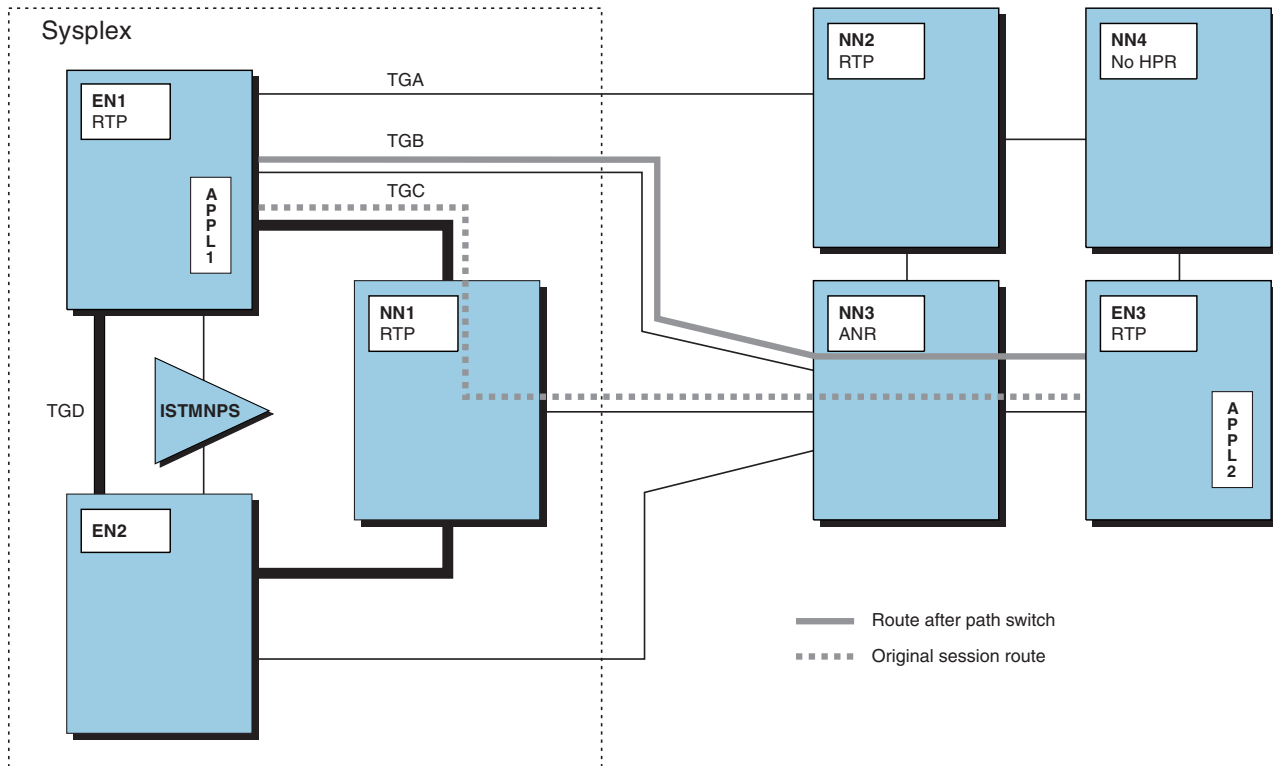
Figure 120. Path switch processing
