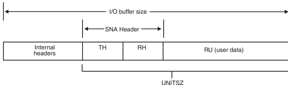
Figure 172. General I/O buffer format
