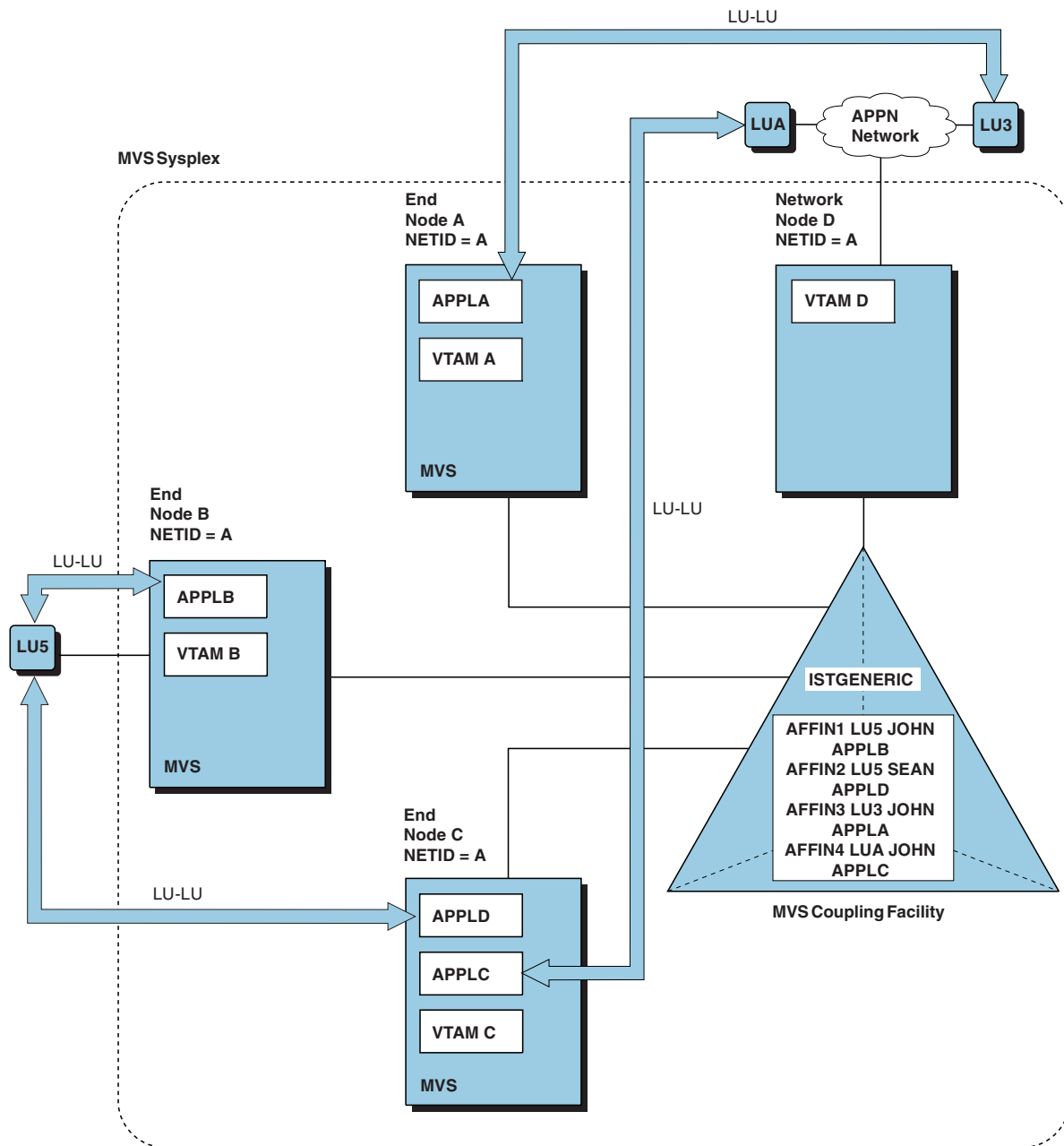
Figure 116. Session establishment with generic resource members
