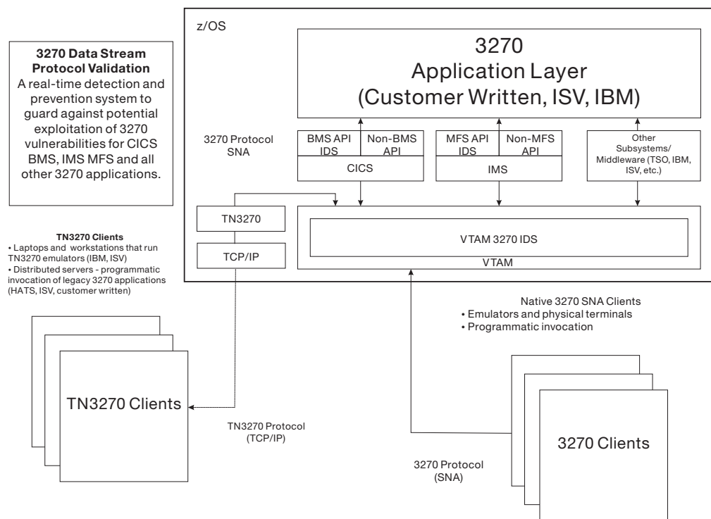
Figure 106. 3270 IDS protection overview
