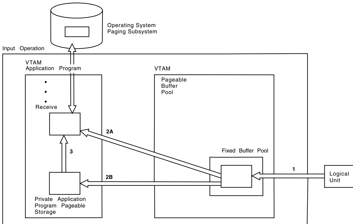
Figure 167. How VTAM uses input buffers
