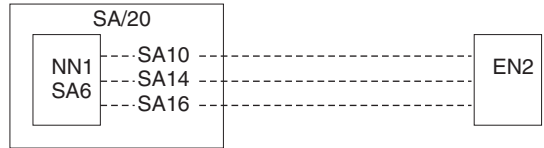
Figure 90. APPN view of CNN session path
