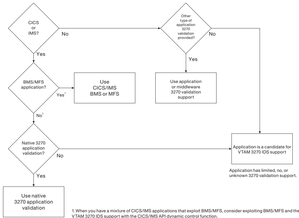
Figure 107. Candidate application assessment process
