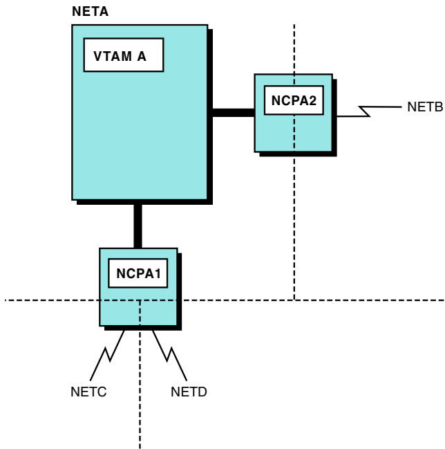
NCPA1 and NCPA2 are gateway NCPs. NCPA1 supports NETC and NETD; NCPA2 supports NETB. NCPA2 has an extra switched line defined. Figure 145. Backup of a gateway NCP - part 1
