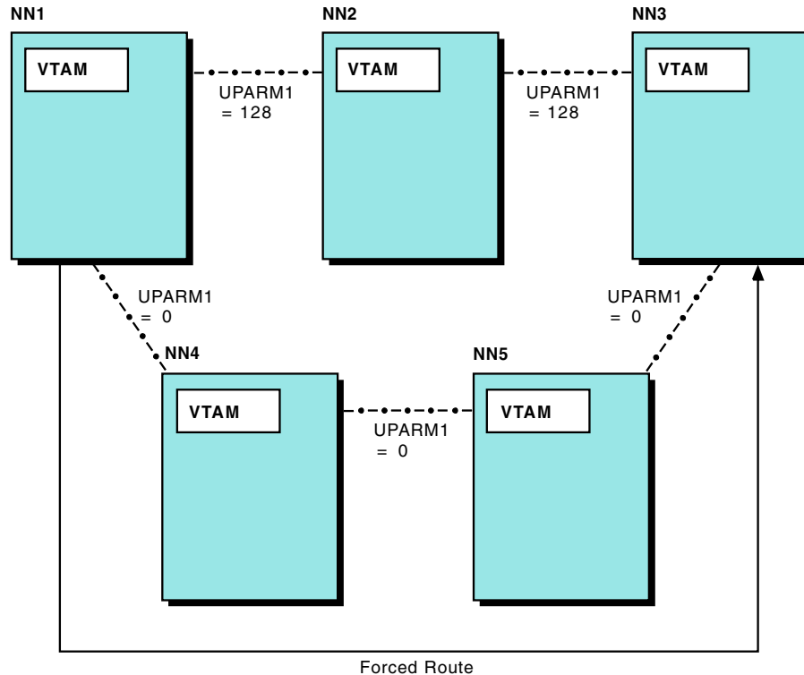
Figure 181. Sample network using TG profile on some links
