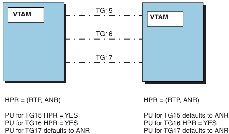
Figure 121. HPR=(RTP,ANR) and TG capabilities
