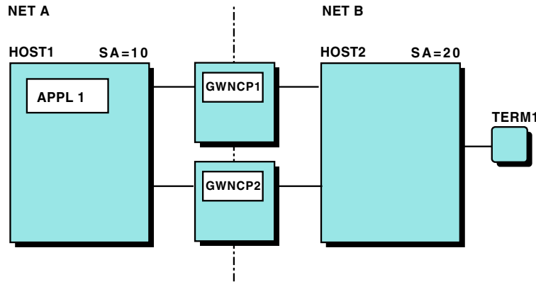
Figure 149. Example of two interconnected networks
