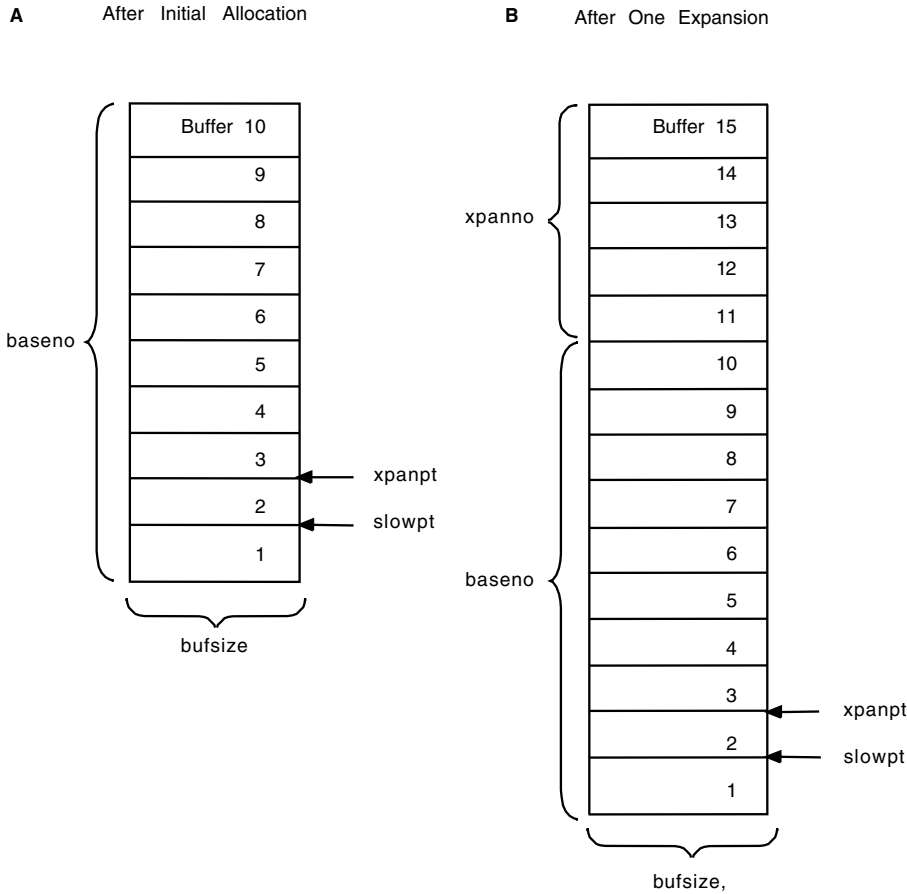
Figure 166. Buffer pool after initial allocation and after one expansion
