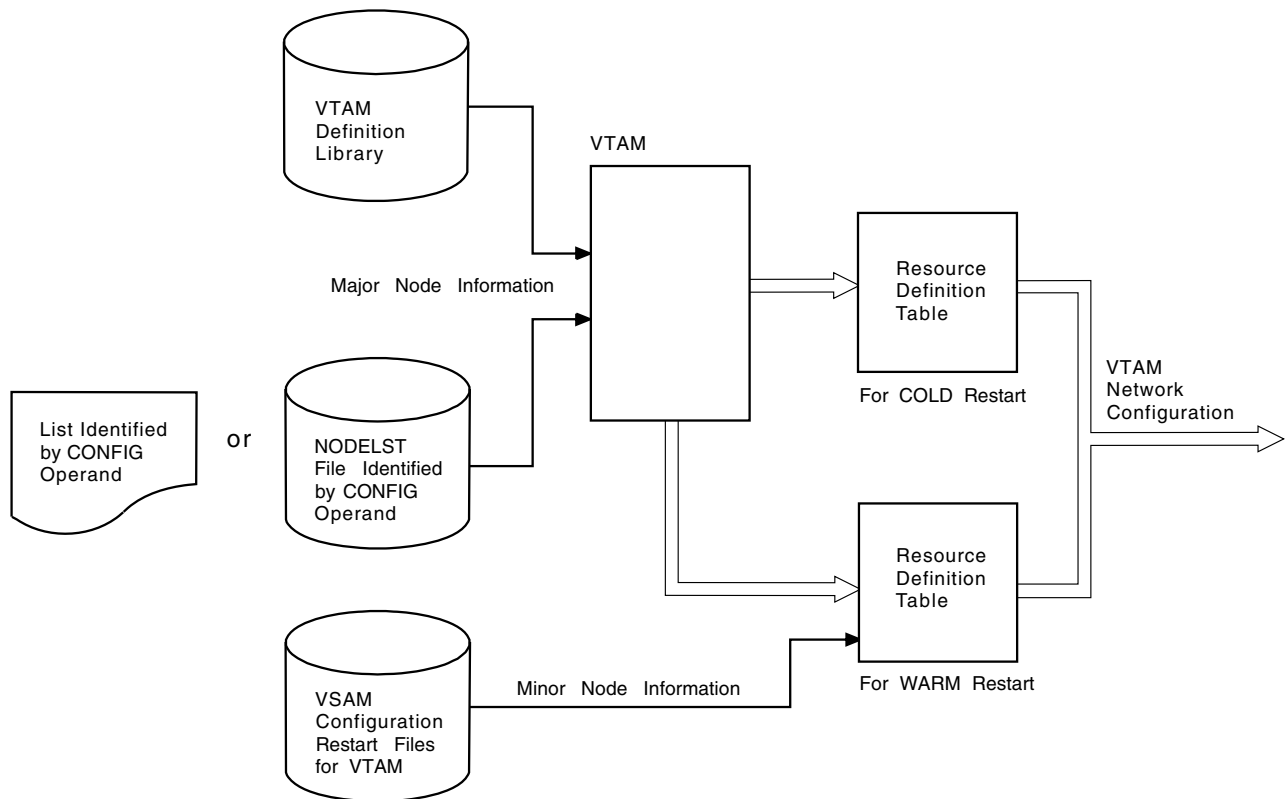
Figure 157. Restoring resource definitions with configuration restart and NODELST files
