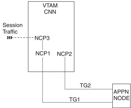
Figure 91. SAMAP session routing concept
