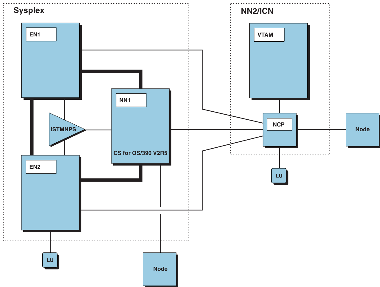
Figure 118. Multinode persistent session network example
