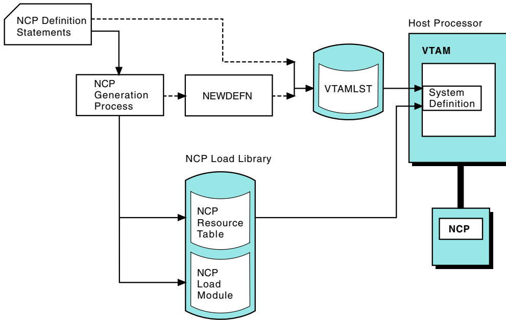
Figure 159. NCP generation
