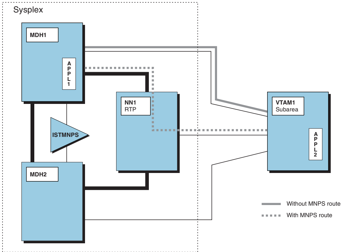
Figure 119. Session routes
