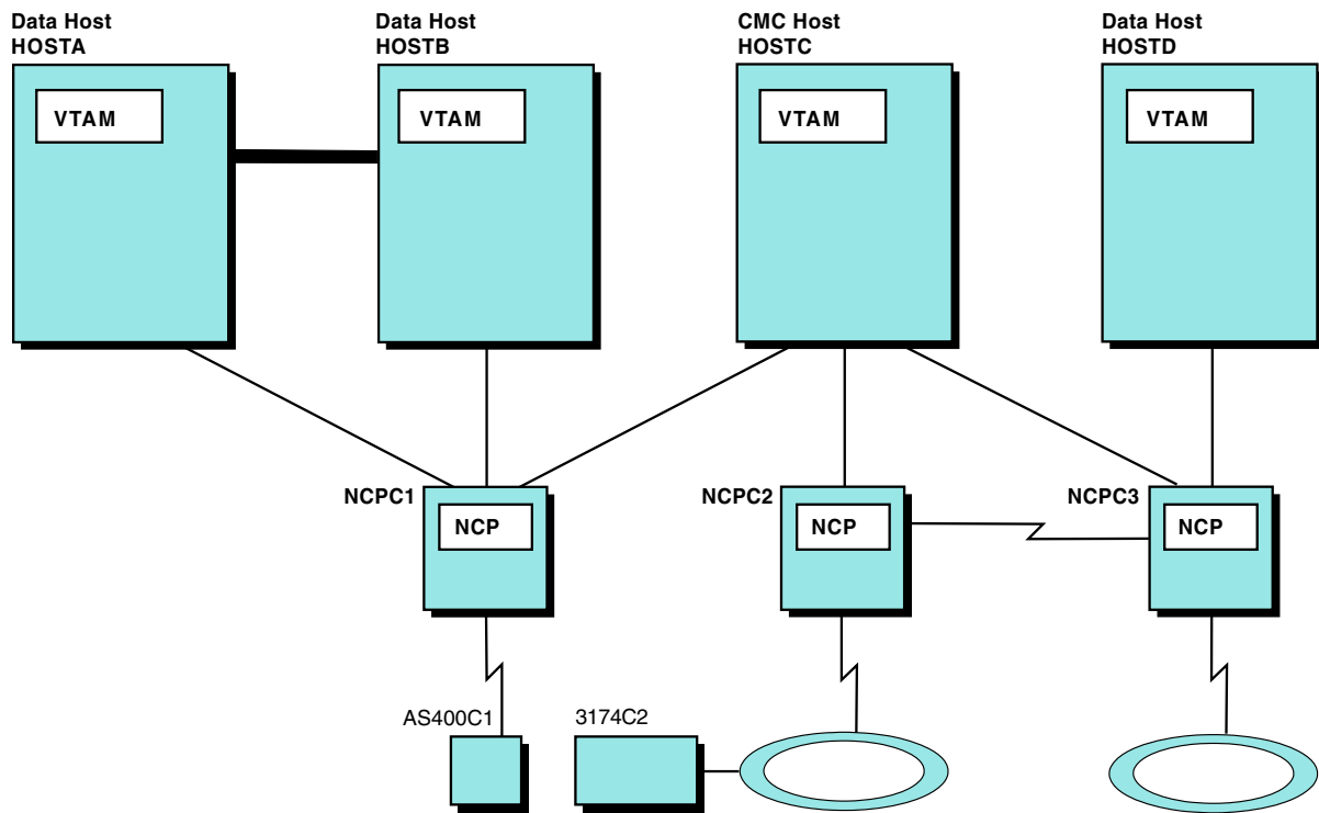
Figure 129. Example of communication management configuration
