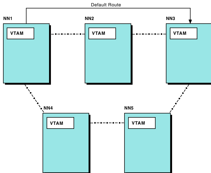
Figure 179. Sample network showing default route
