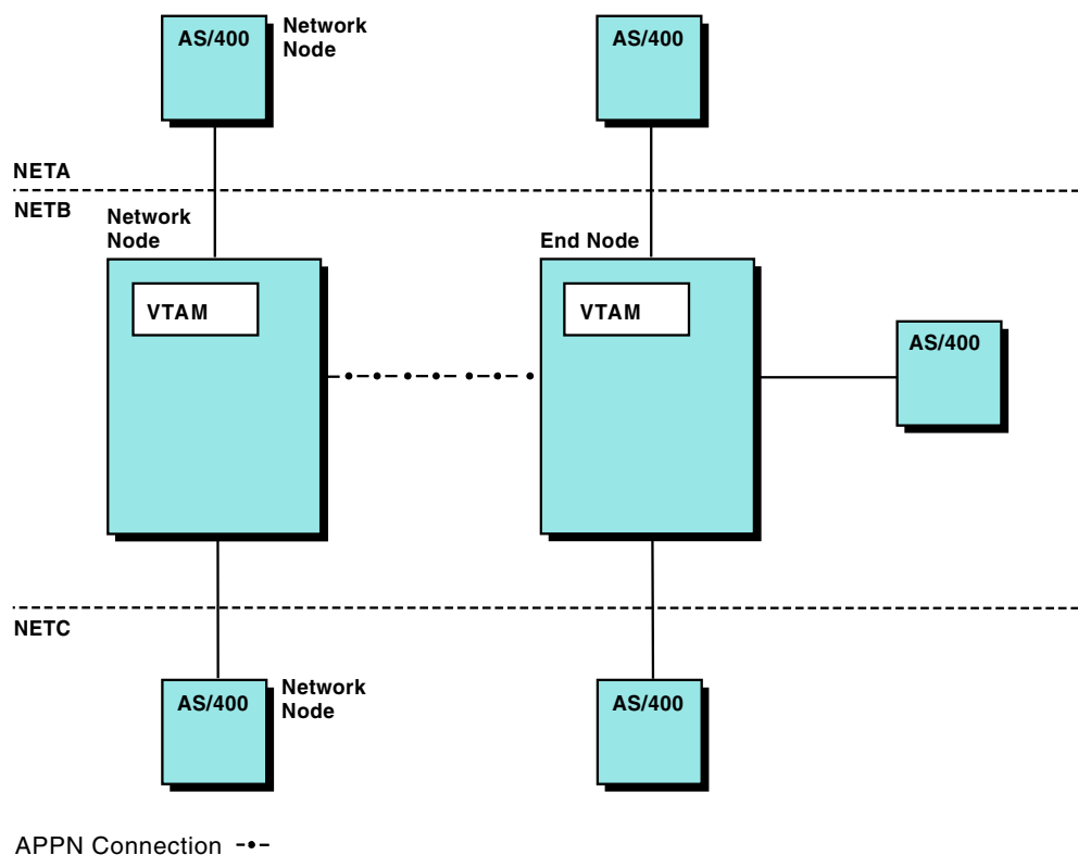
Figure 156. Nonnative network type 2.1 connections
