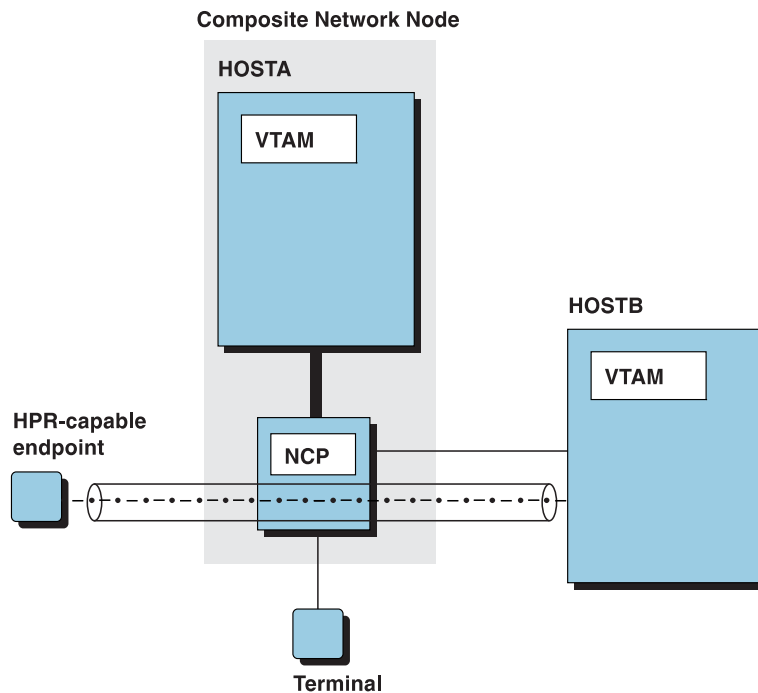
Figure 125. Using VR-based TGs for non-HPR endpoints
