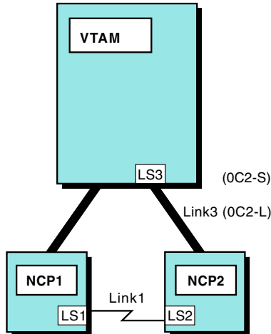
Figure 162. Automatic activation of link stations
