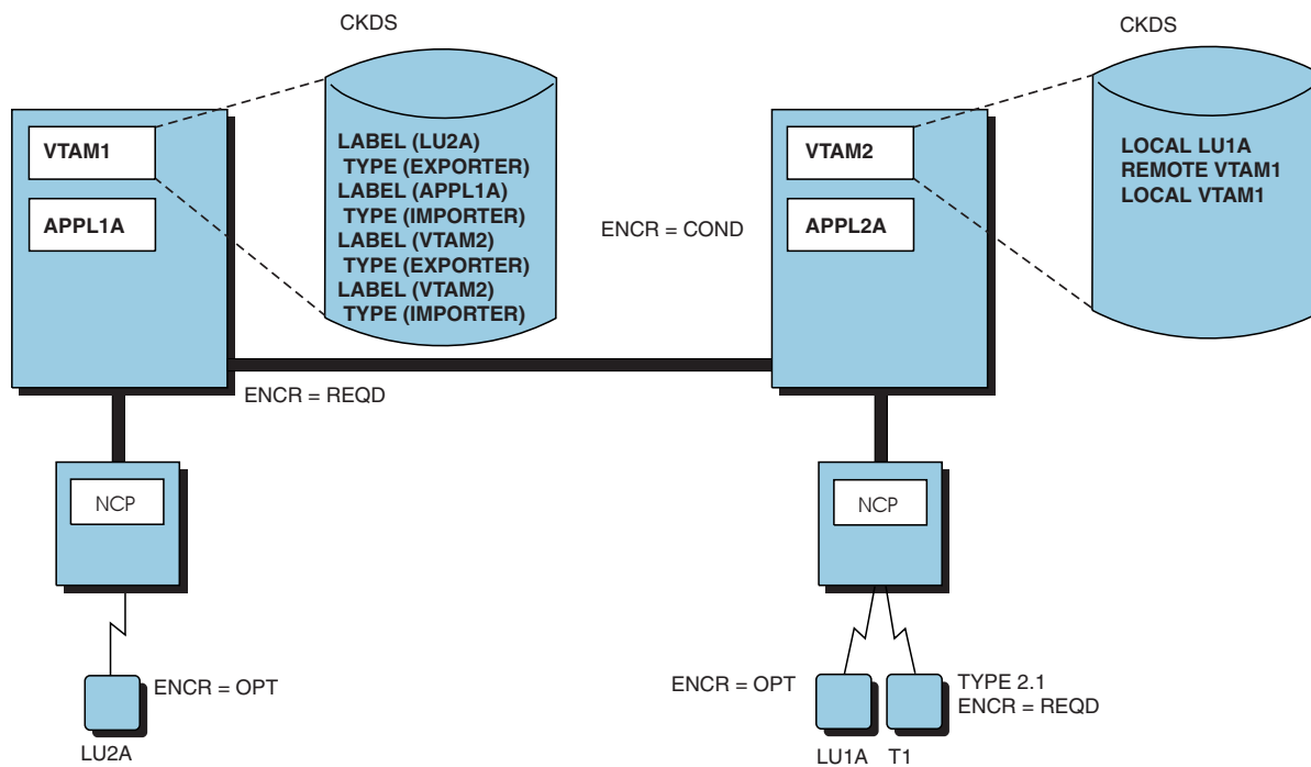
Figure 178. Cryptography in multiple-domain environment (Hosts use different cryptographic services)
