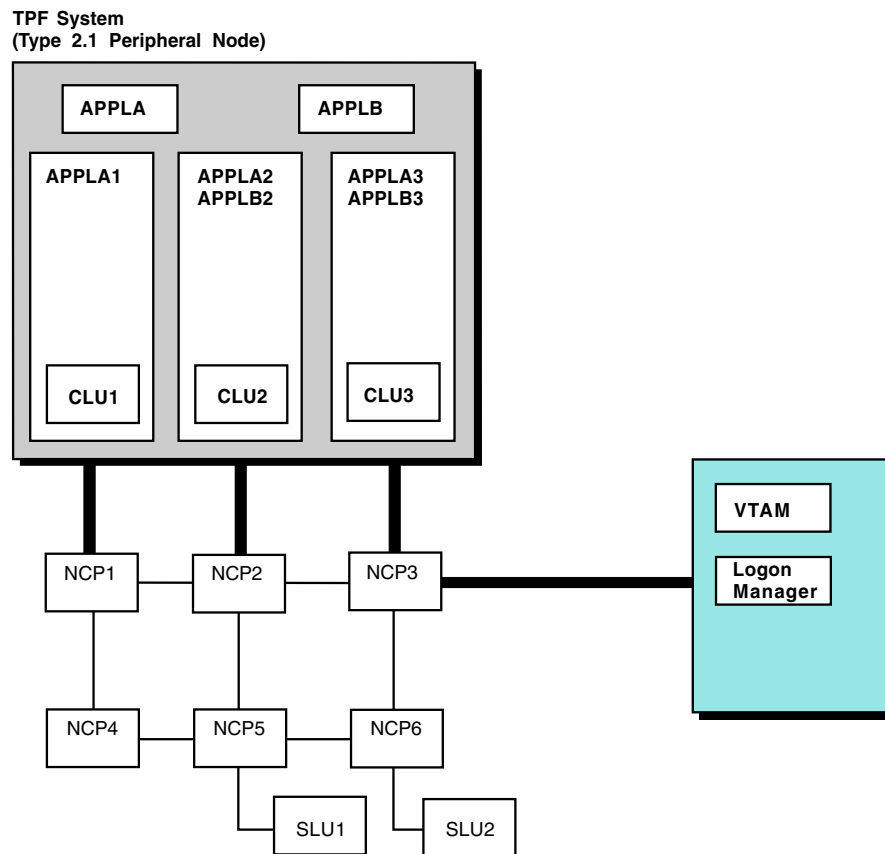
Figure 175. Sample Logon Manager Configuration
