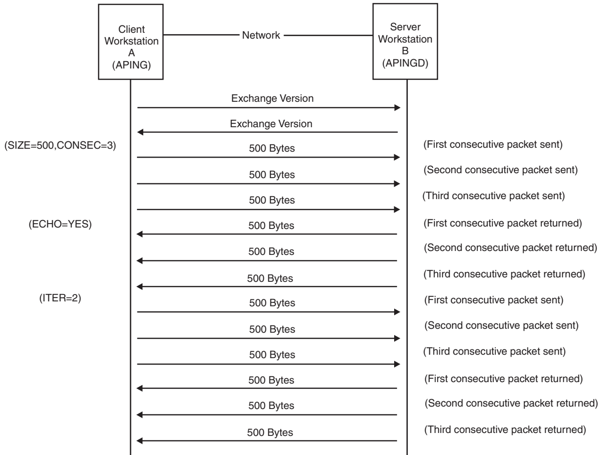
Figure 113. Example of flows between client and server for DISPLAY APING command
