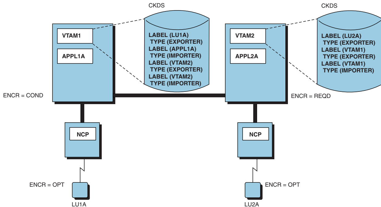
Figure 177. Cryptography in multiple-domain environment (Both hosts use ICSF/MVS)
