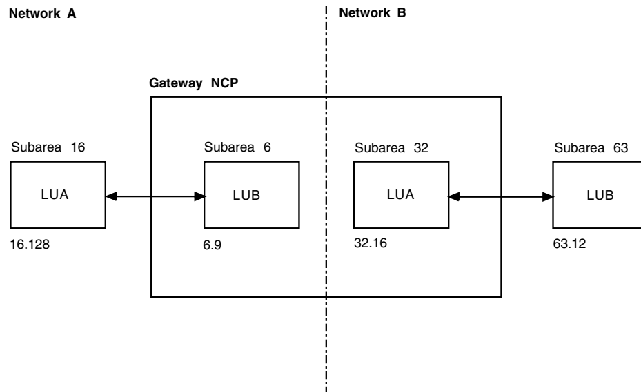
Figure 154. Address translation
