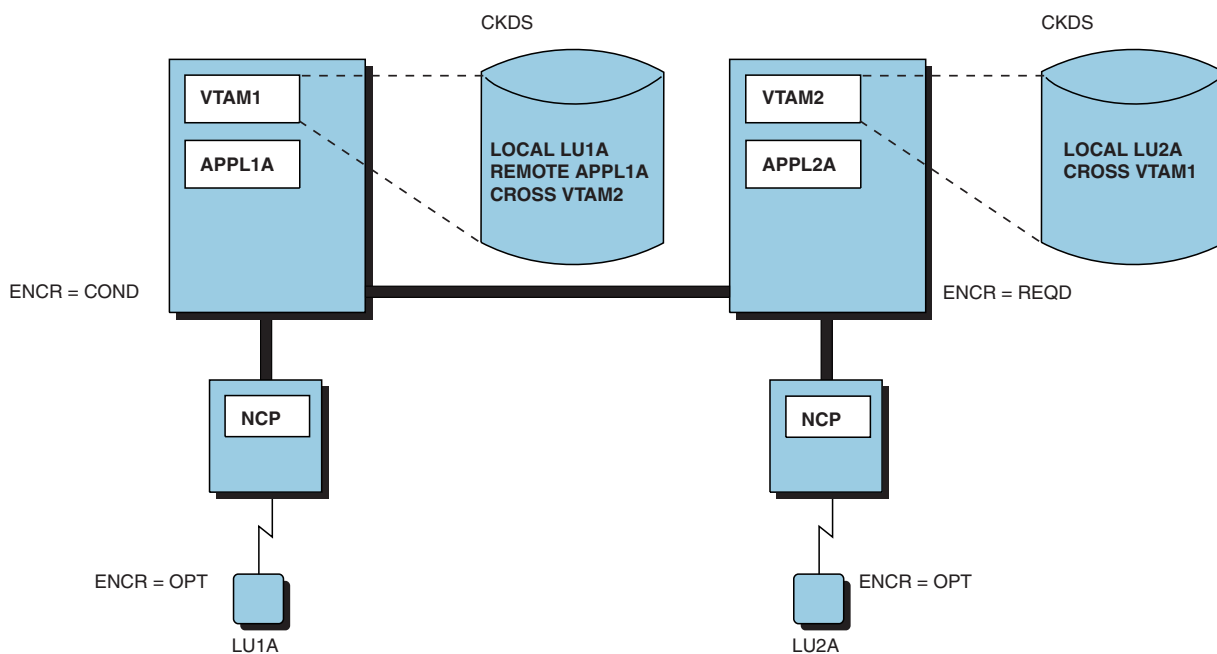
Figure 176. Cryptography in multiple-domain environment (Both hosts use PCF/CUSP)
