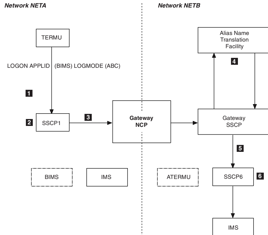
Figure 155. Example of name translation
