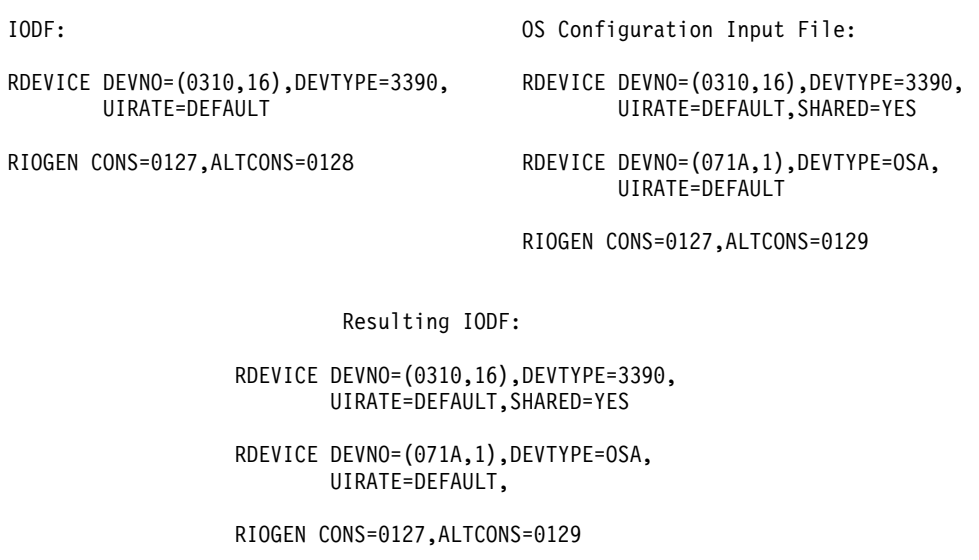
Figure 30. Partial Migration of an OS Configuration Input File
