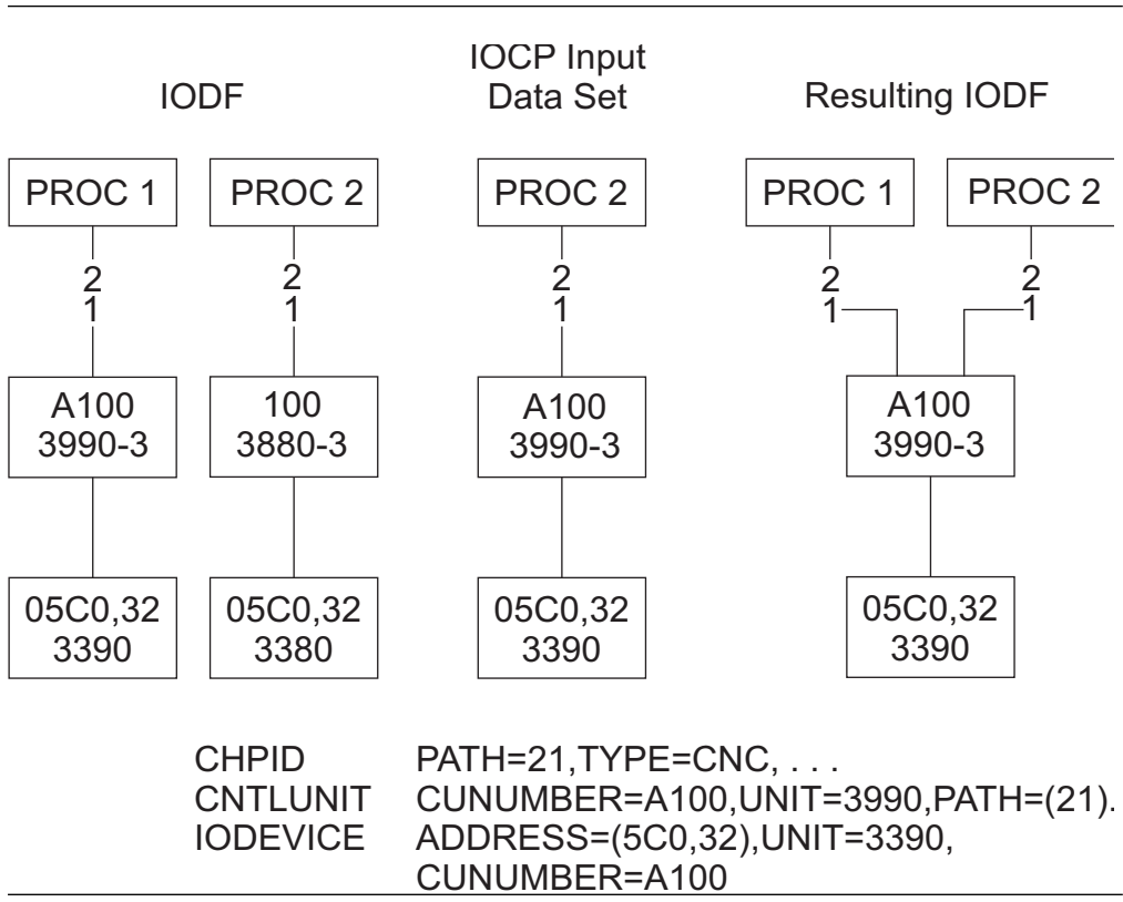
Figure 29. Partial Migration of an IOCP Input File. Control unit defined for two processors is migrated to the second processor.
