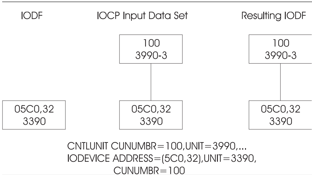
Figure 21. IOCP Migration. Devices are mapped, because the attached control unit is not yet defined in the IODF.
