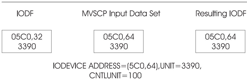
Figure 24. OS Migration. 32 devices are mapped, the other 32 devices are newly defined.
