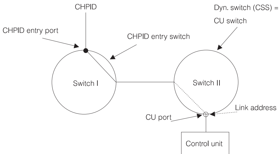
Figure 13. Example of a Configuration with Two Switches (1)
