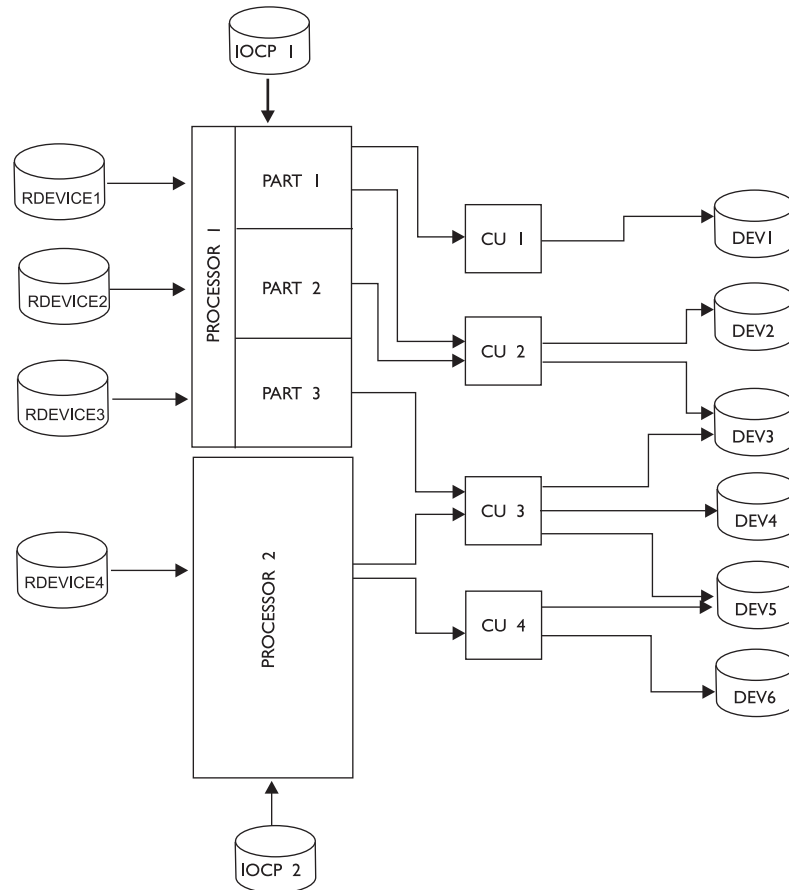
Figure 1. Configuration Definition without HCD/with Multiple Files
