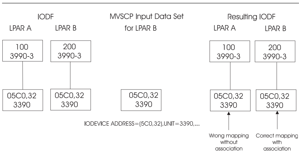
Figure 23. OS Migration. Devices are mapped to the first devices found with the same type and number.
