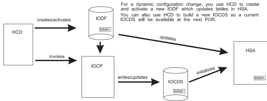
Figure 9. I/O Configuration to Hardware
