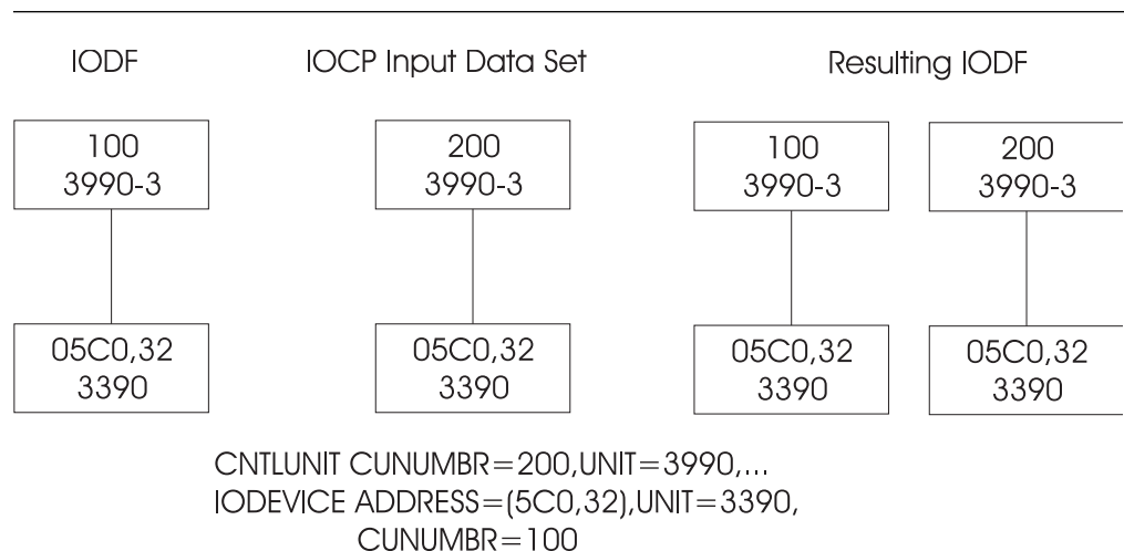
Figure 22. IOCP Migration. Devices are not mapped, because the control unit number does not exist in the IODF.
