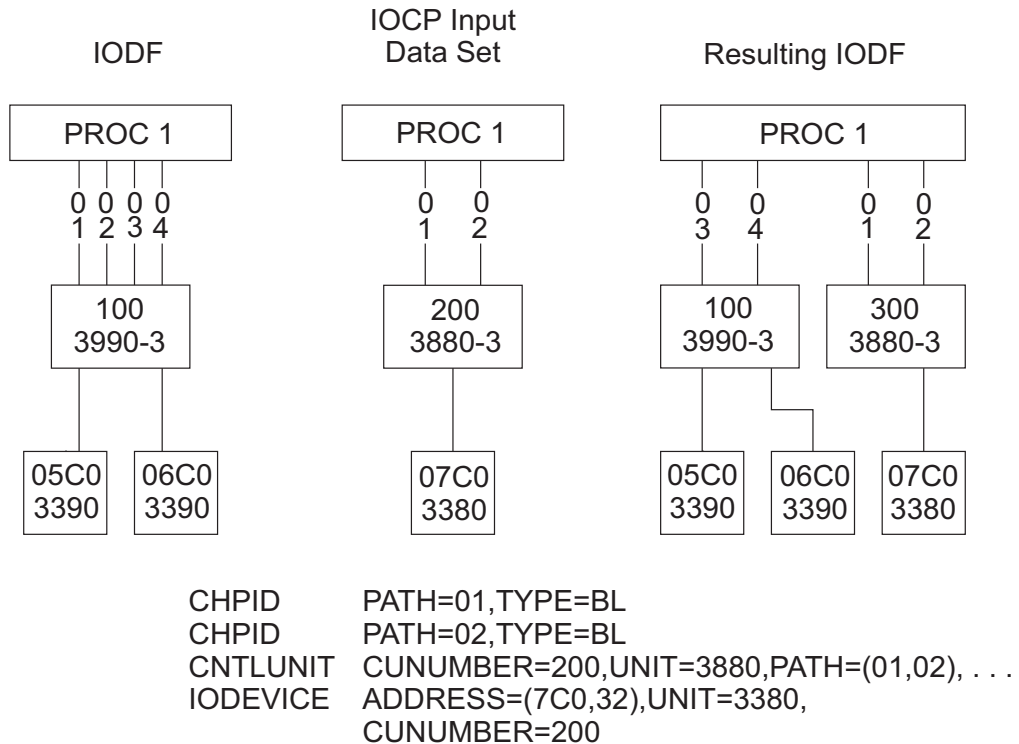
Figure 27. Partial Migration of an IOCP Input File. CHPIDs are defined as in the IOCP input file
