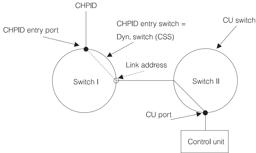
Figure 14. Example of a Configuration with Two Switches (2)
