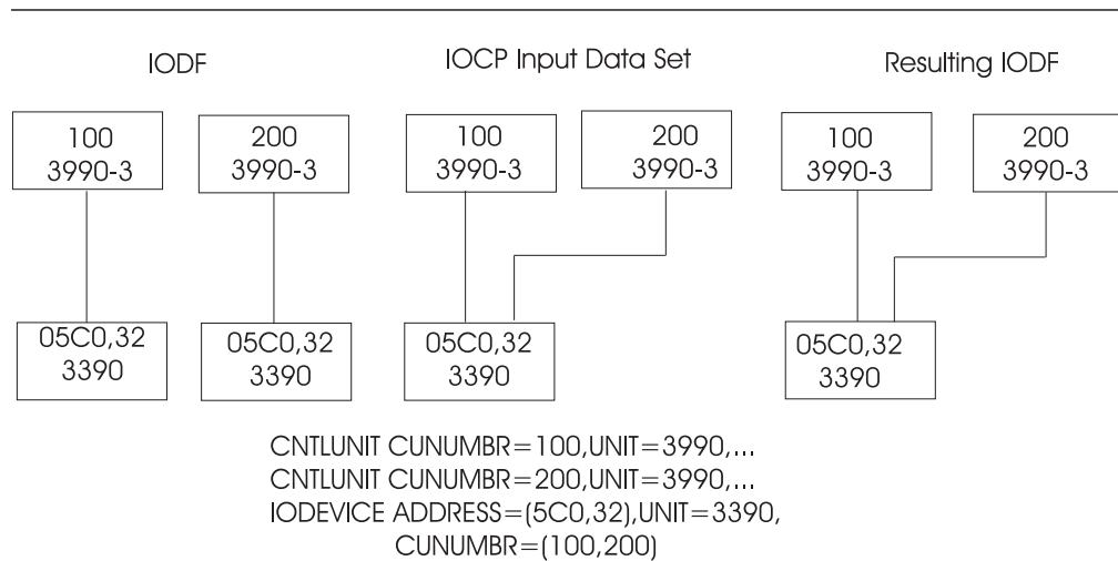
Figure 19. IOCP Migration. Control units and devices are mapped (only if the control units do not connect to the same processor configuration).
