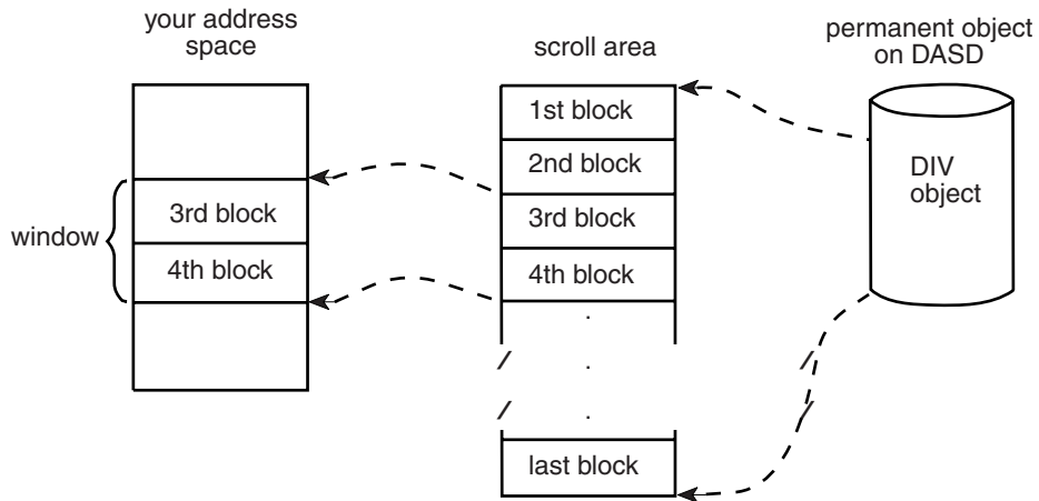
Figure 17-3. Mapping a Permanent Object That Has A Scroll Area
