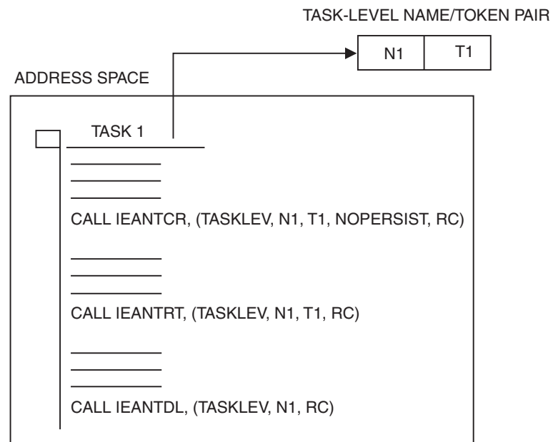
Figure 18-2. Using the Task Level in a Single Address Space
