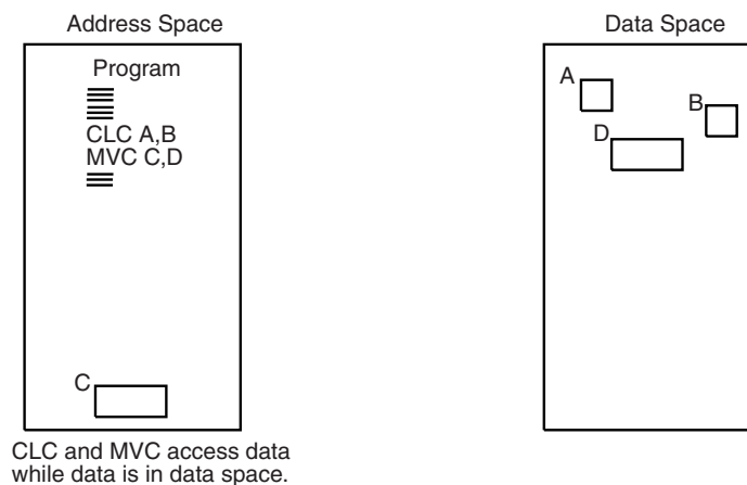
Figure 16-1. Accessing Data in a Data Space
