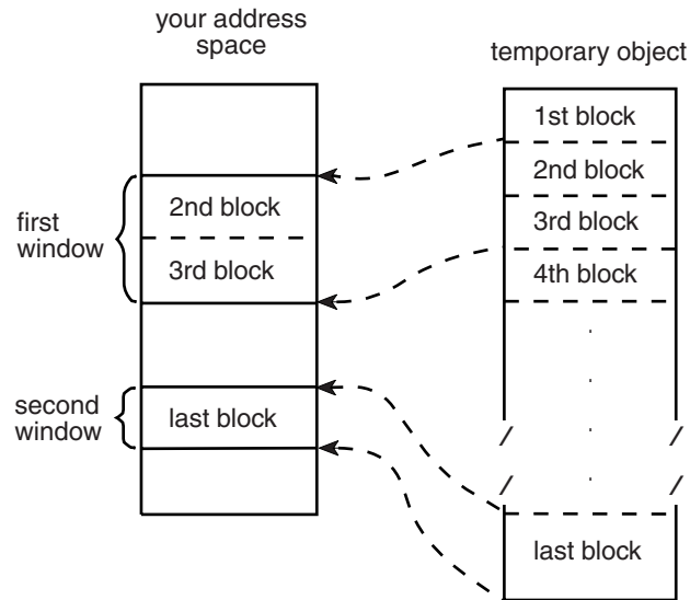
Figure 17-5. Mapping an Object To Multiple Windows
