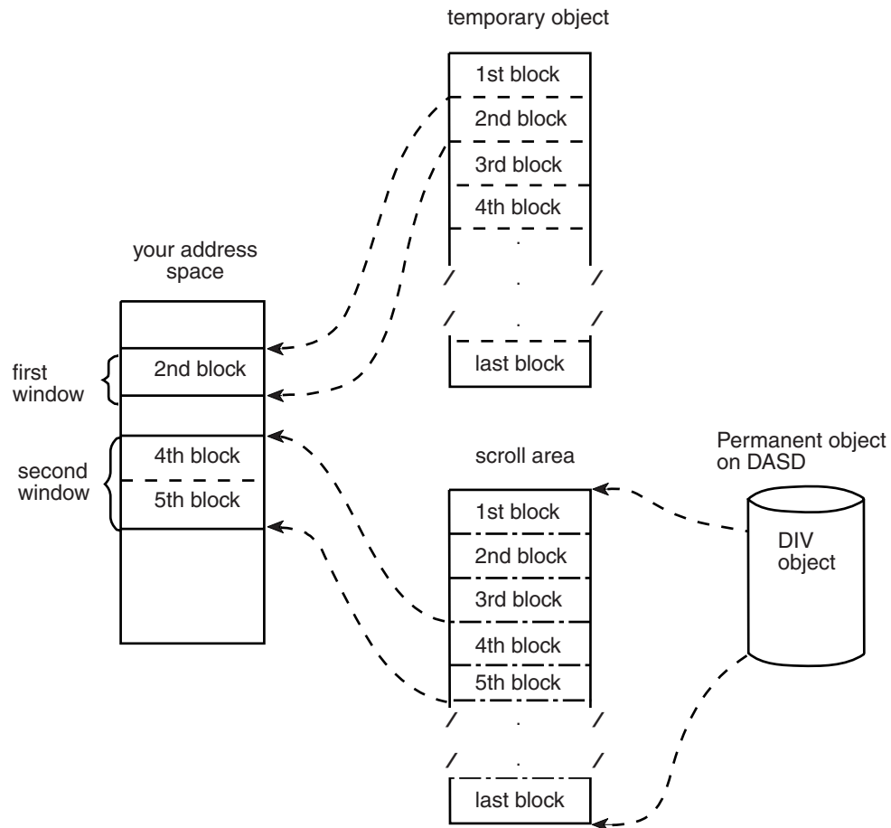
Figure 17-6. Mapping Multiple Objects
