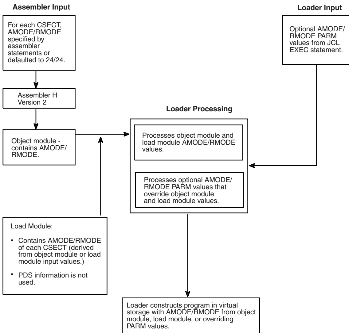
Figure 5-5. AMODE and RMODE Processing by the Loader
