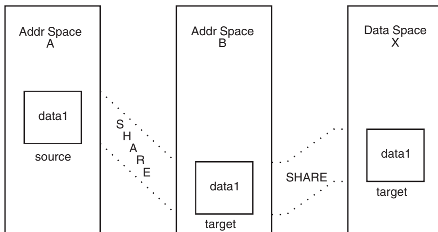
Figure 20-1. Data Sharing with IARVSERV
