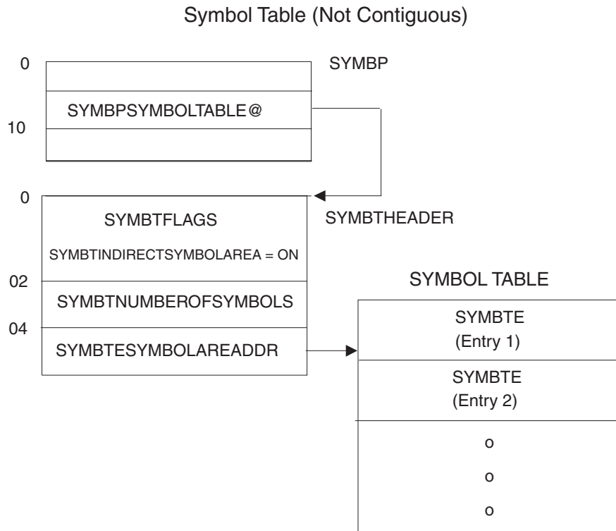
Figure 26-2. Non-contiguous Symbol Table
