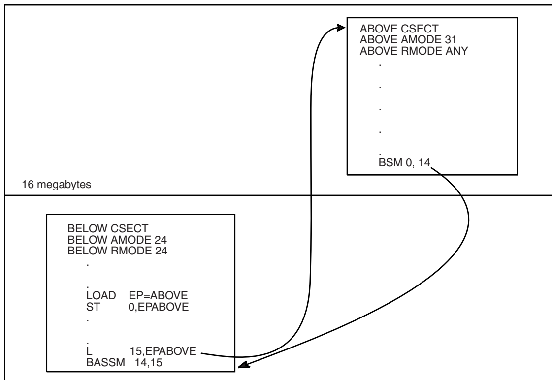
Figure 5-10. Using BASSM and BSM
