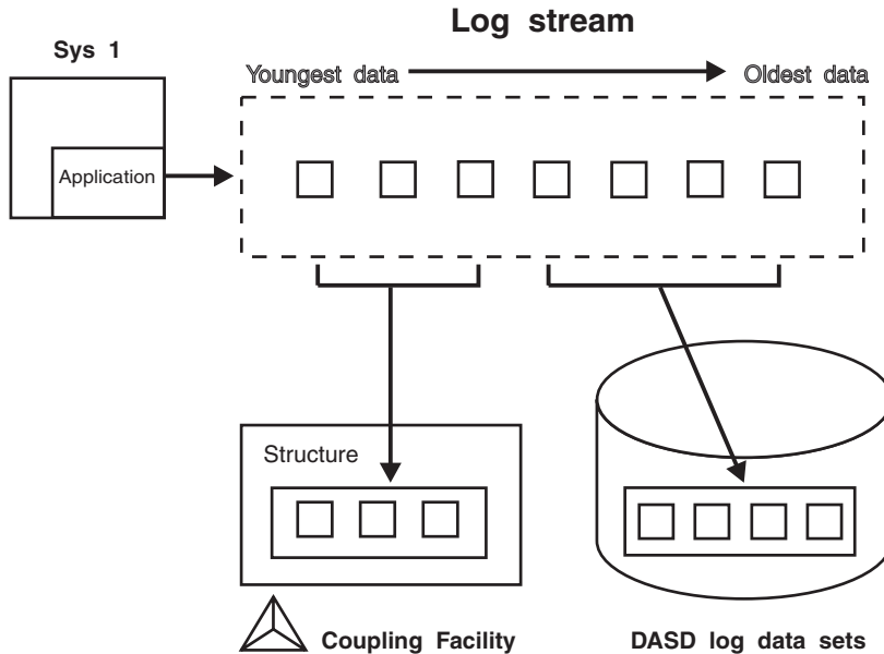
Figure 27-2. Log Stream Data on the Coupling Facility and DASD
