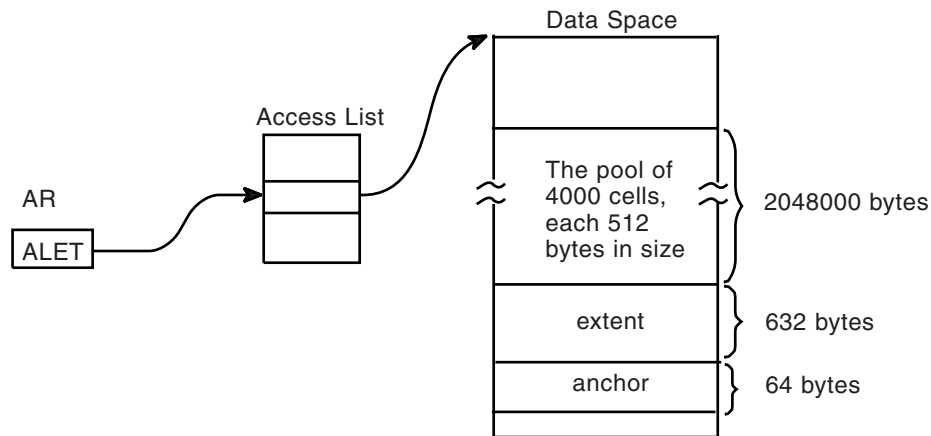
Figure 16-5. Example of Using Callable Cell Pool Services for Data Spaces
