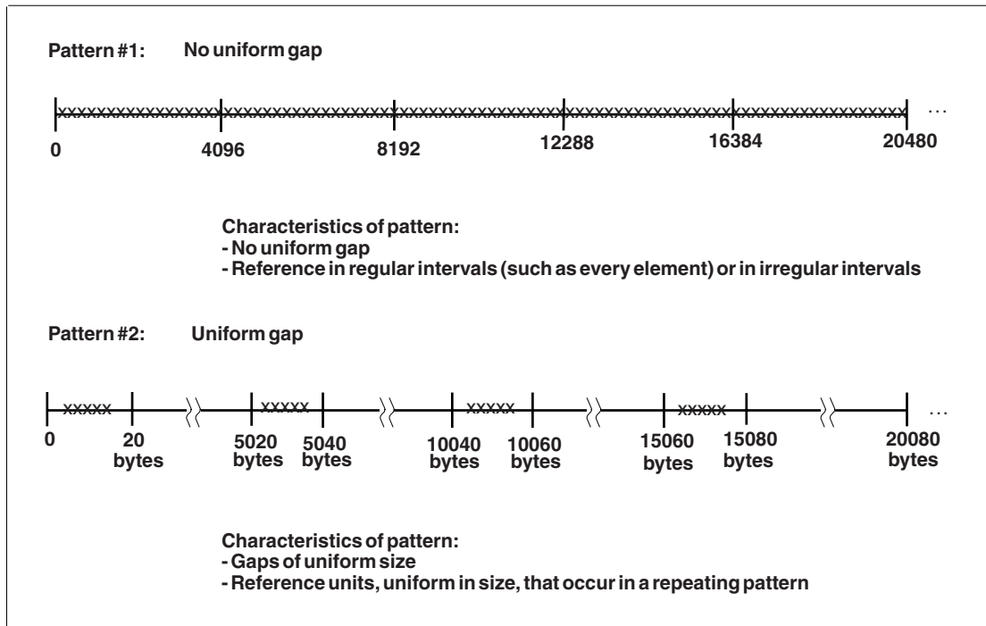
Figure 19-6. Two Typical Reference Patterns
