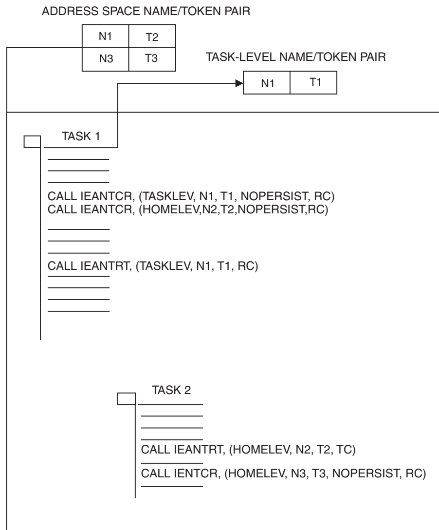
Figure 18-3. Using Home-Level and Task-Level Name/Token Pairs
