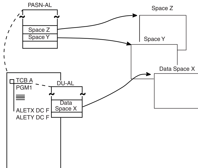
Figure 15-2. An Illustration of a DU-AL
