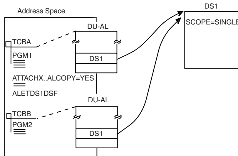
Figure 16-6. Two Problem Programs Sharing a SCOPE=SINGLE Data Space
