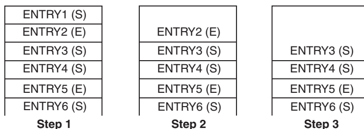
Figure 6-6. ISGENQ Macro Processing
