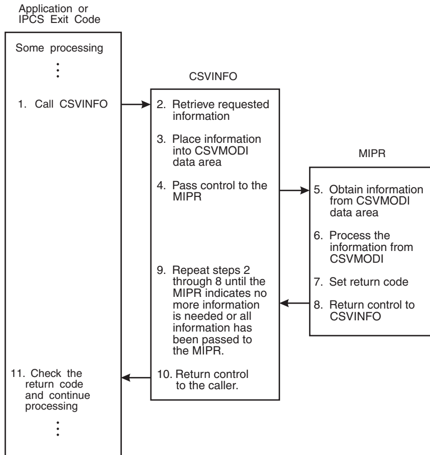
Figure 4-20. Processing Flow for the CSVINFO Macro and the Caller's MIPR
