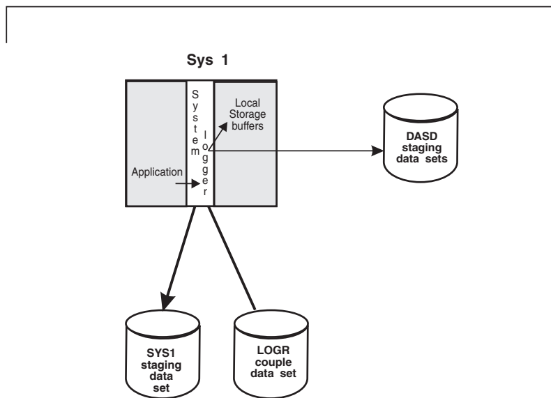
Figure 27-5. A DASD-Only Configuration
