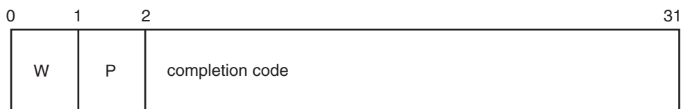
Figure 6-1. Event Control Block (ECB)
