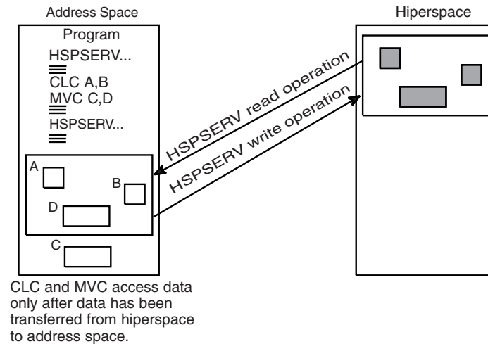
Figure 16-2. Accessing Data in a Hiperspace
