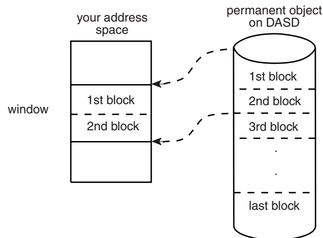
Figure 17-2. Mapping a Permanent Object That Has No Scroll Area
