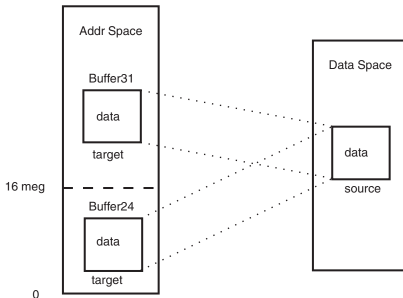
Figure 20-2. Sharing Storage with IARVSERV
