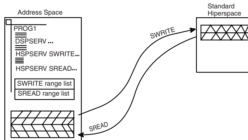
Figure 16-9. Example of Creating a Standard Hiperspace and Transferring Data
