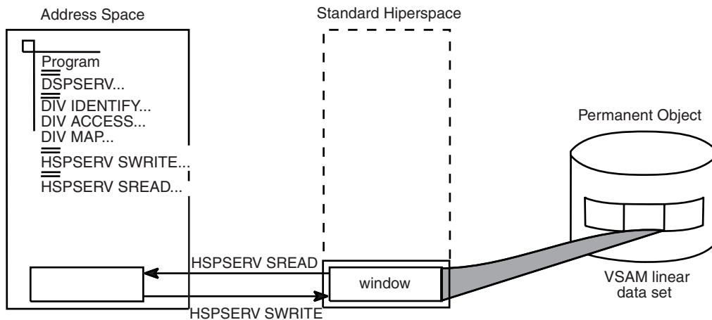
Figure 16-10. Example of Mapping a Data-in-Virtual Object to a Hiperspace
