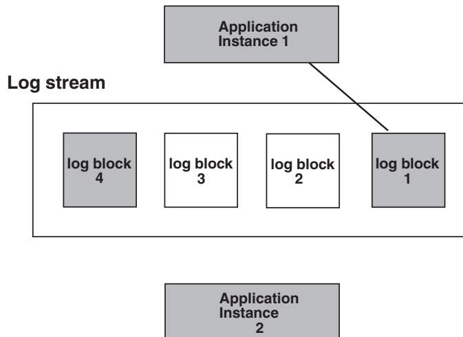
Figure 27-1. System Logger Log Stream
