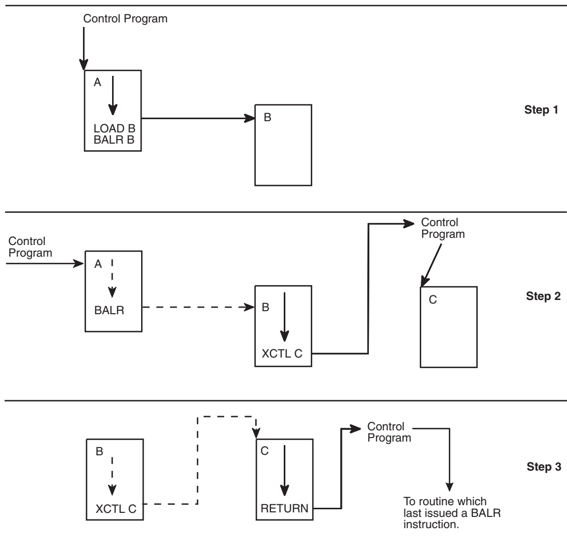
Figure 4-19. Misusing Control Program Facilities Causes Unpredictable Results
