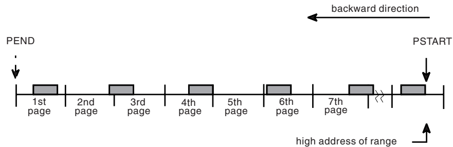
Figure 19-5. Illustration of Backward Direction in a Reference Pattern
