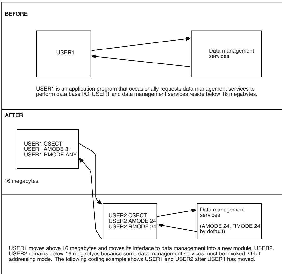
Figure 5-15. Performing I/O While Residing Above 16 Megabytes
