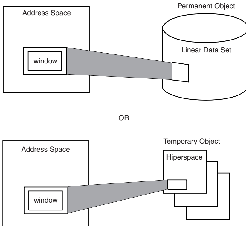
Figure 14-1. Mapping from an Address Space
