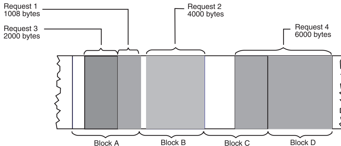
Figure 11-2. Virtual Storage Control
