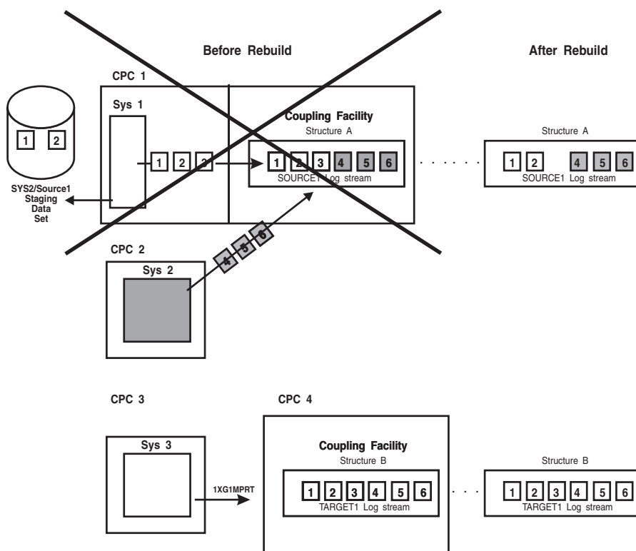
Figure 27-10. How Source and Target Log Streams Can Get Out of Sync
