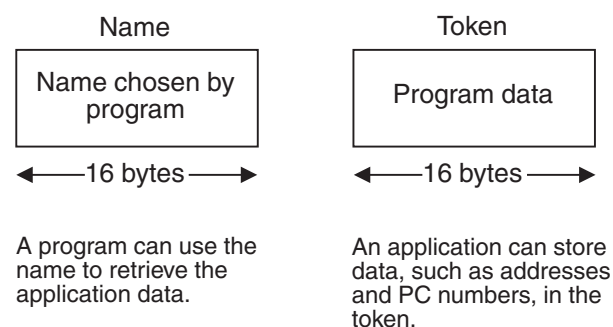
Figure 18-1. Using the Name and the Token
