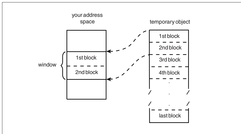
Figure 17-4. Mapping a Temporary Object
