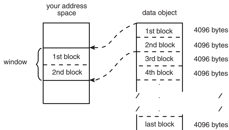
Figure 17-1. Structure of a Data Object
