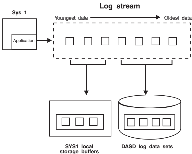
Figure 27-3. Log Stream Data in Local Storage Buffers and DASD Log Data Sets
