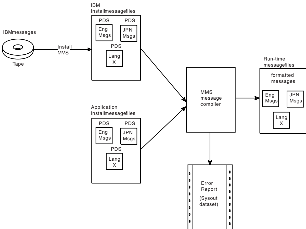
Figure 22-1. Preparing Messages for Translation
