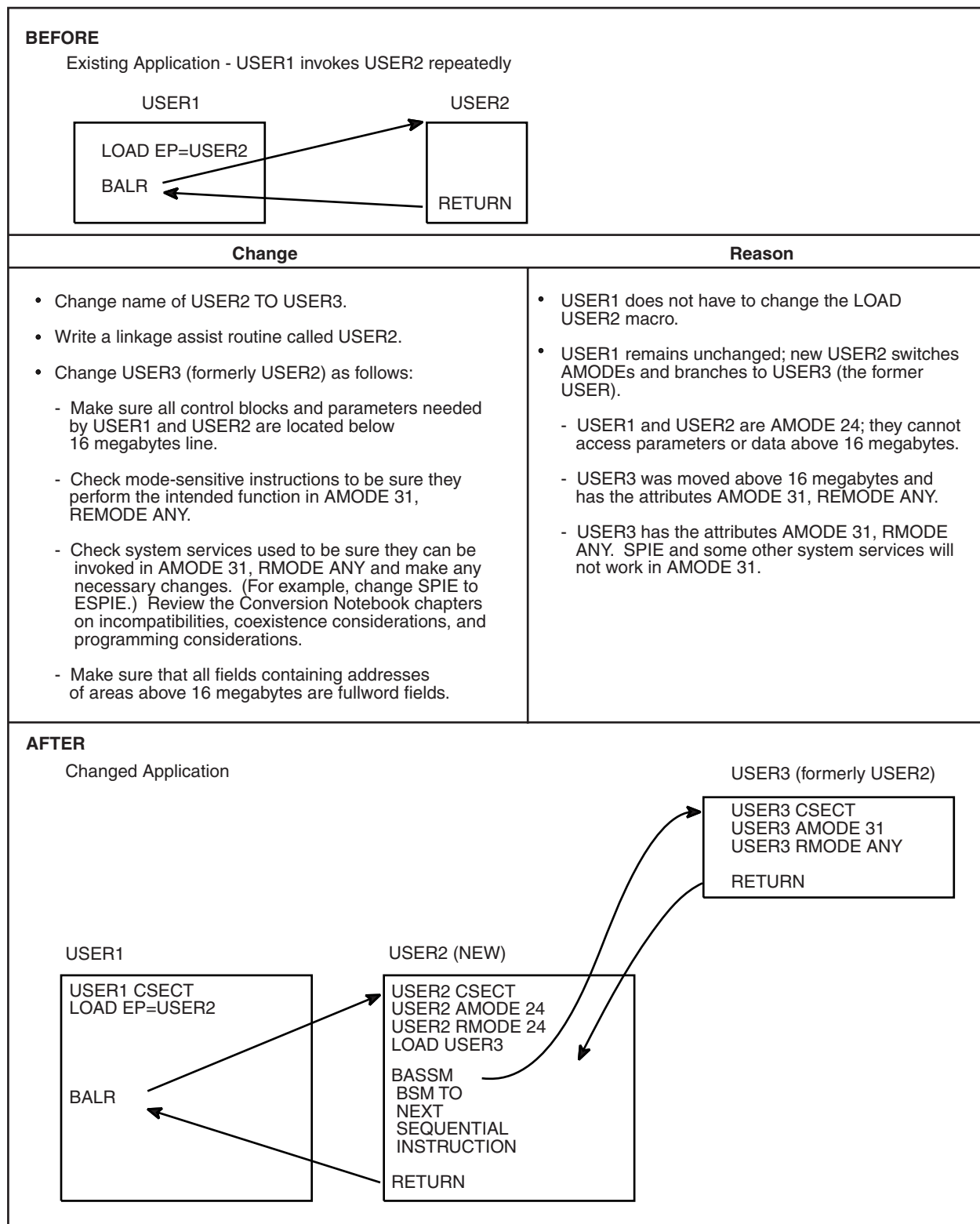
Figure 5-13. Example of a Linkage Assist Routine (Part 1 of 4)
