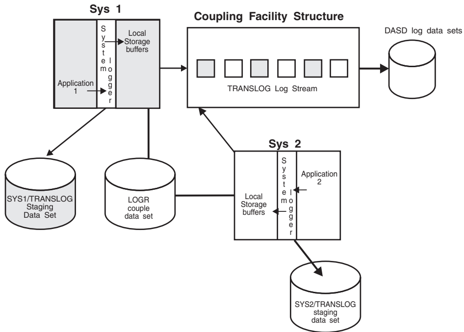
Figure 27-4. A Complete Coupling Facility Log Stream Configuration
