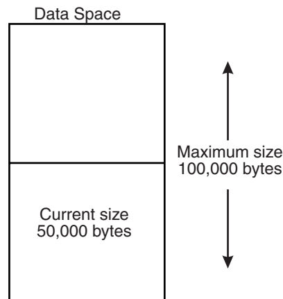
Figure 16-4. Example of Extending the Current Size of a Data Space
