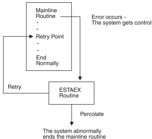
Figure 8-1. Mainline Routine with One Recovery Routine
