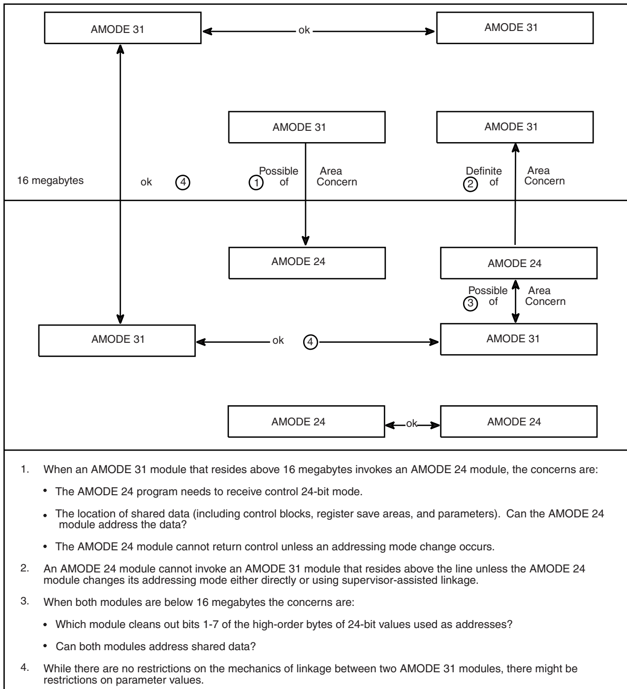
Figure 5-7. Linkage Between Modules with Different AMODEs and RMODEs
