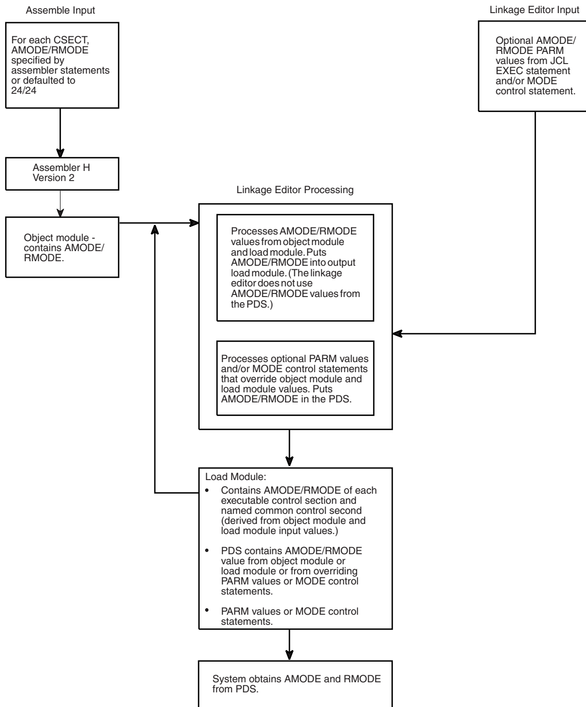
Figure 5-4. AMODE and RMODE Processing by the Linkage Editor
