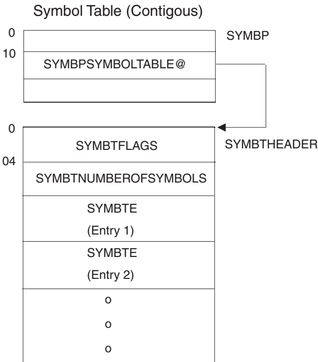
Figure 26-1. Contiguous Symbol Table
