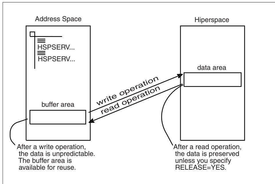
Figure 16-8. Illustration of the HSPSERV Write and Read Operations
