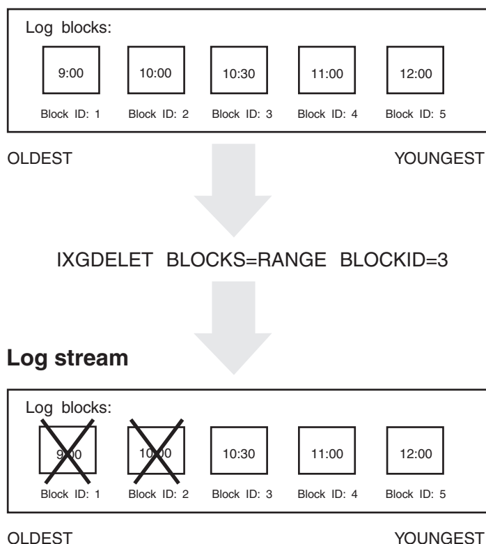
Figure 27-9. Deleting a Range of Log Blocks
