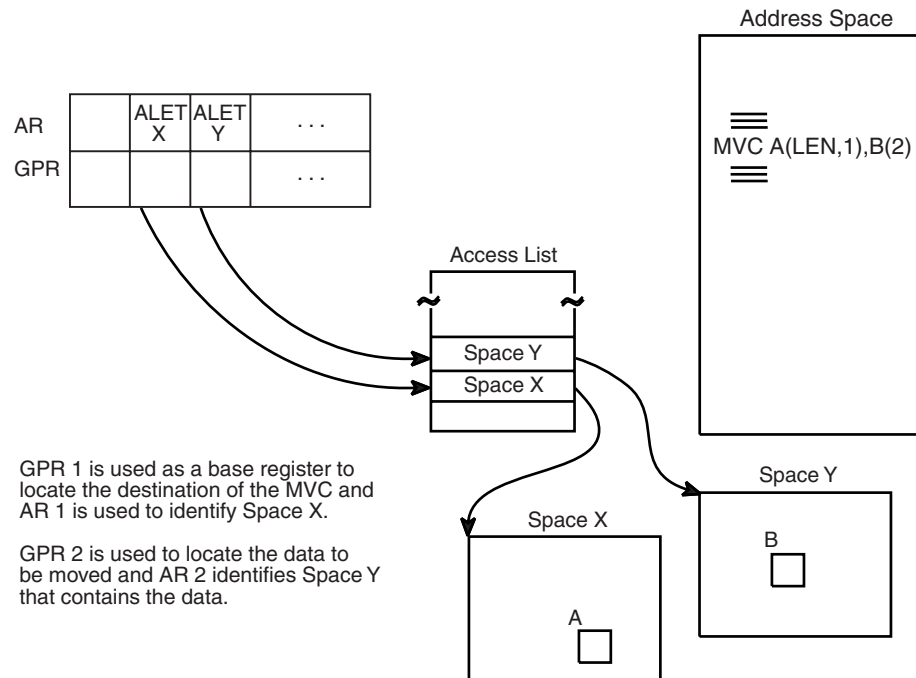
Figure 15-3. Using Instructions in AR Mode
