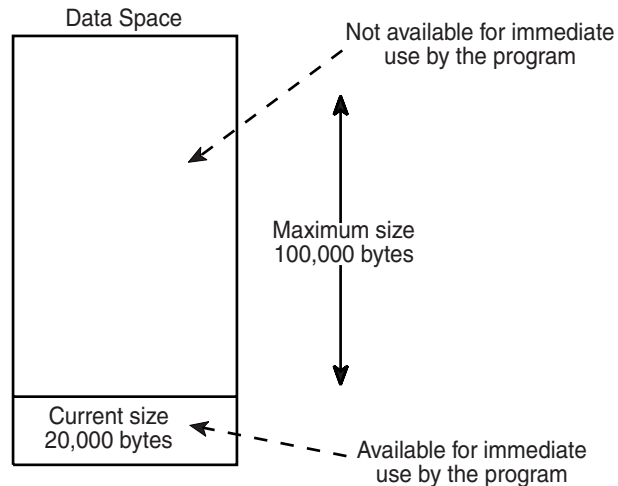
Figure 16-3. Example of Specifying the Size of a Data Space
