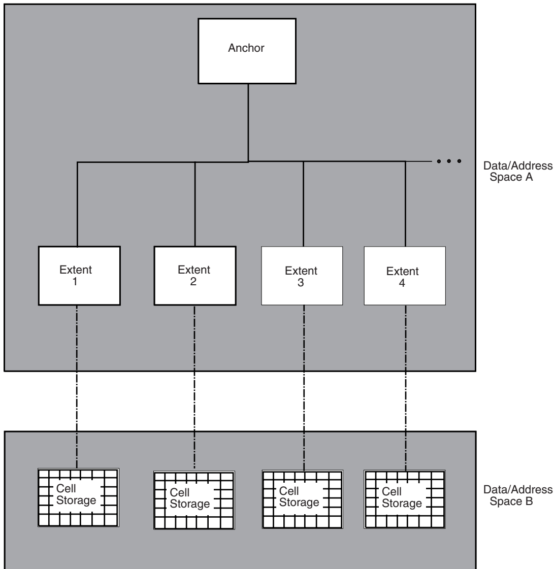
Figure 13-1. Cell Pool Storage
