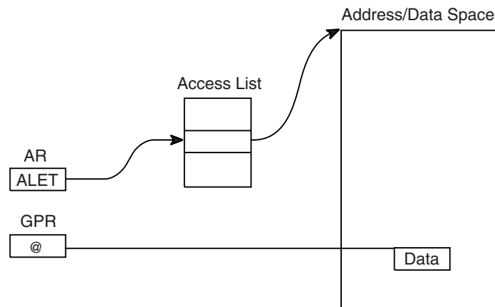
Figure 15-1. Using an ALET to Identify an Address Space or a Data Space
