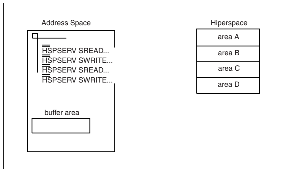
Figure 16-7. Example of Scrolling through a Standard Hiperspace
