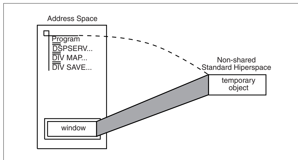
Figure 16-11. A Standard Hiperspace as a Data-in-Virtual Object
