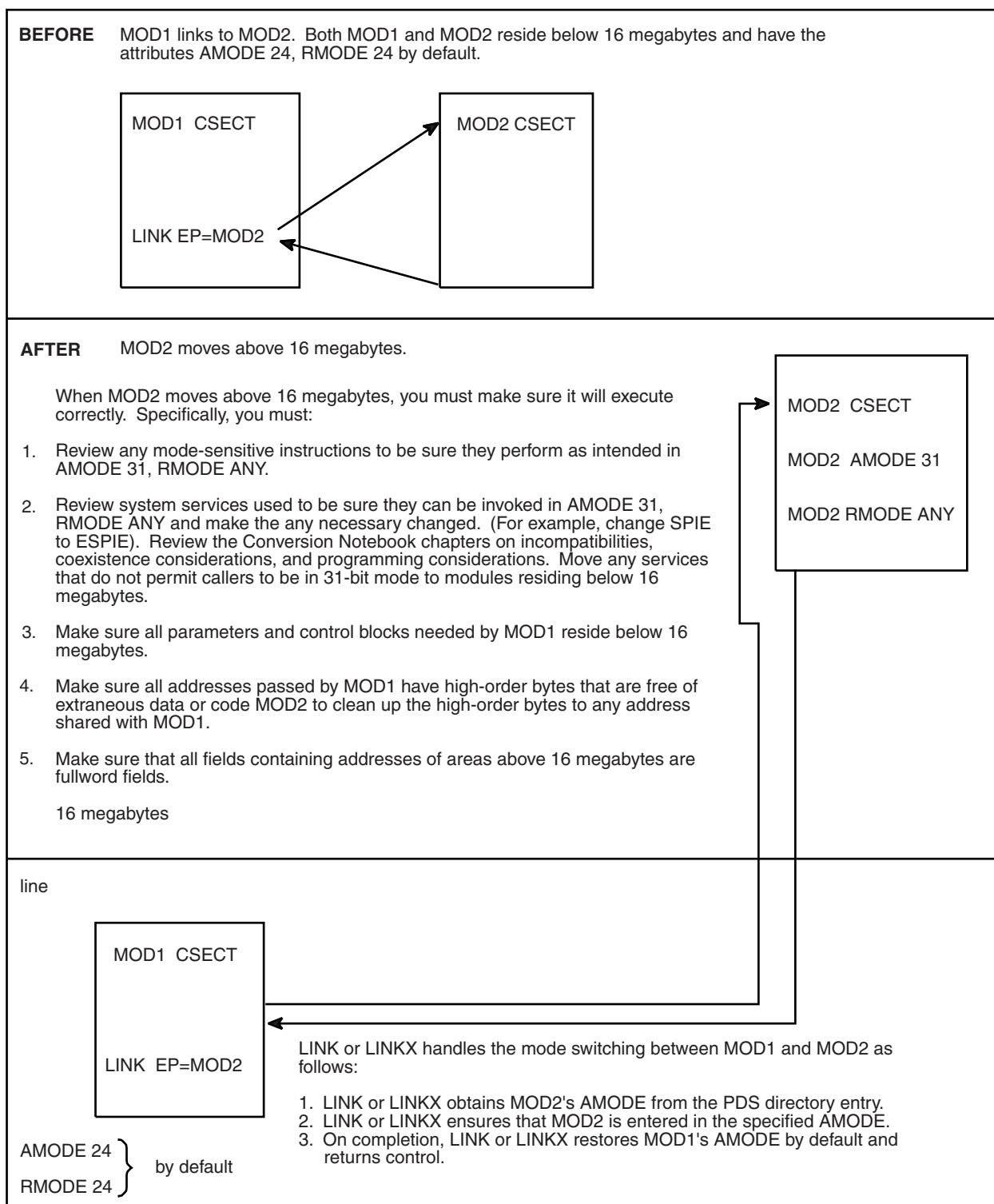
Figure 5-12. Example of Supervisor-Assisted Linkage
