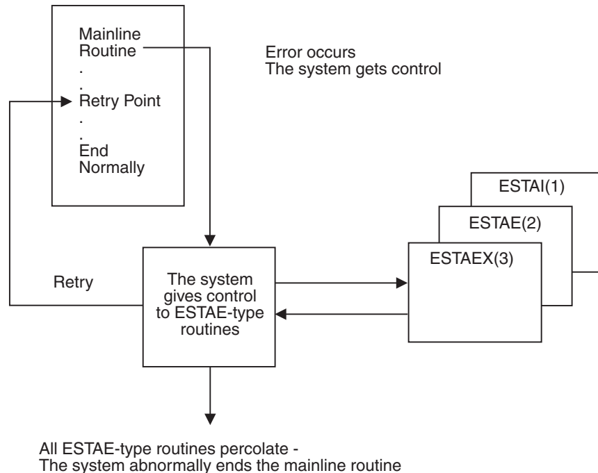
Figure 8-2. Mainline Routine with Several Recovery Routines
