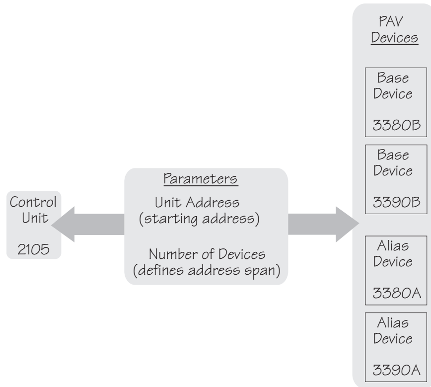
Figure 2-8. Control Unit - PAV Device Relationship
