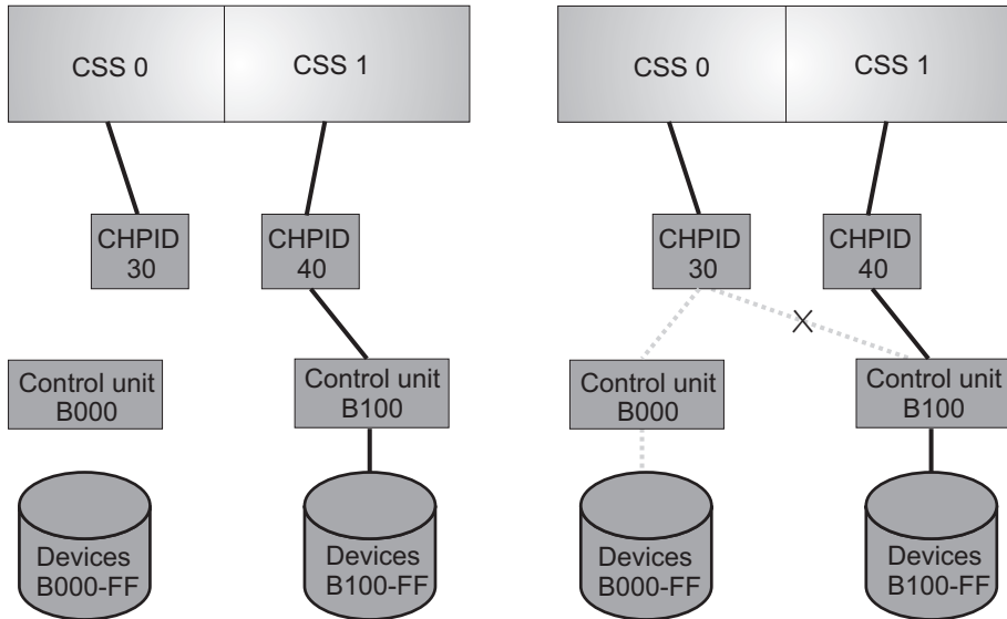
Figure 4-4. Dynamically adding control units and devices in a two LCSS environment on a z990 with compatibility support
