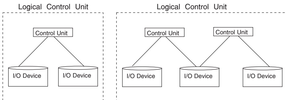
Figure 2-2. Logical Control Unit Examples
