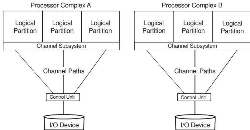
Figure 2-5. Shared Channel Paths
