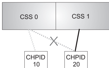
Figure 4-3. Dynamically adding CHPIDs in a two LCSS environment on a z990 with compatibility support
