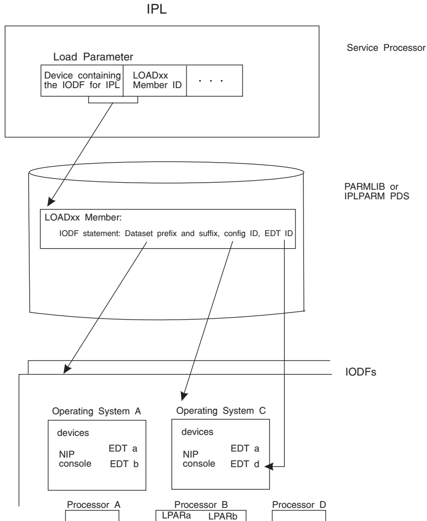
Figure 3-1. Specifying IODF at IPL
