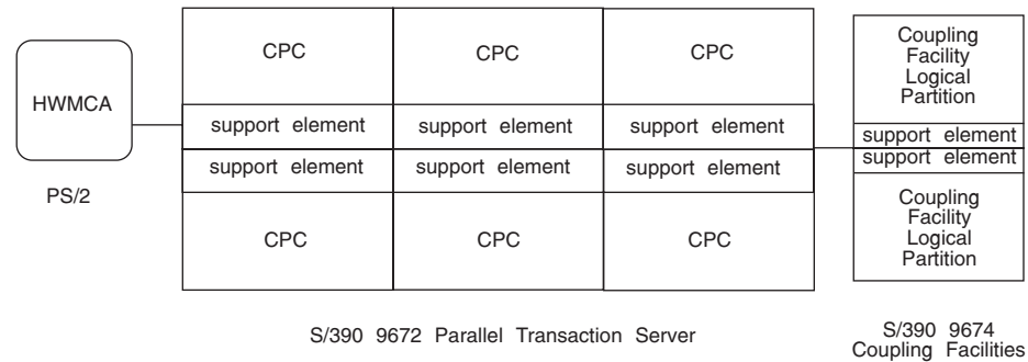
Figure 2-4. Support Elements connected to the Hardware Management Console
