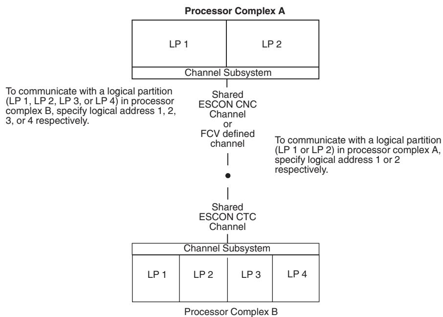
Figure 2-6. Logical Addresses and Logical Partition Numbers
